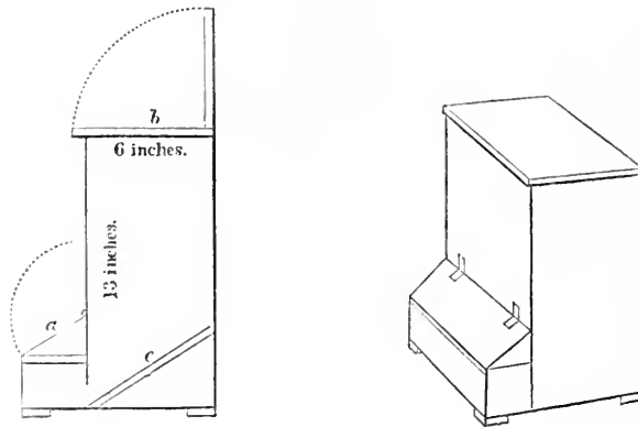
FEEDER FOR GRAIN.
