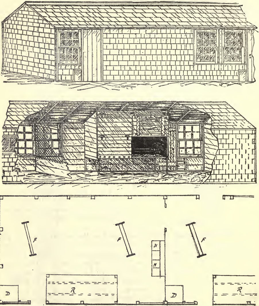
Fig. 21. Poultry House with Roosts on South Side.—Showing in the upper drawing the exterior perspective of a section 12 x 28 ft.; below it interior view of the south side and roost box; in the lower drawing the ground plan in which R is the roost box; N, nests; D, dust box; F, feed troughs; the small squares indicate the positions of studs.
