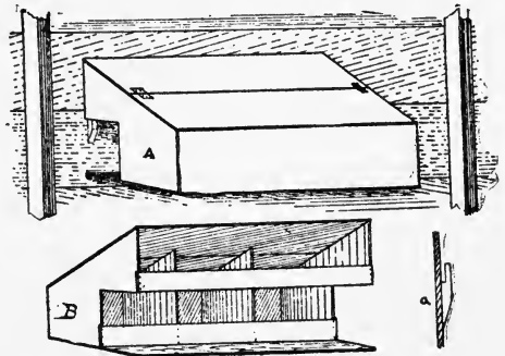
Fig. 36. Dark Nest to hang on Wall. A, exterior view; B, interior view; a, mortised block to hold nest in place.
