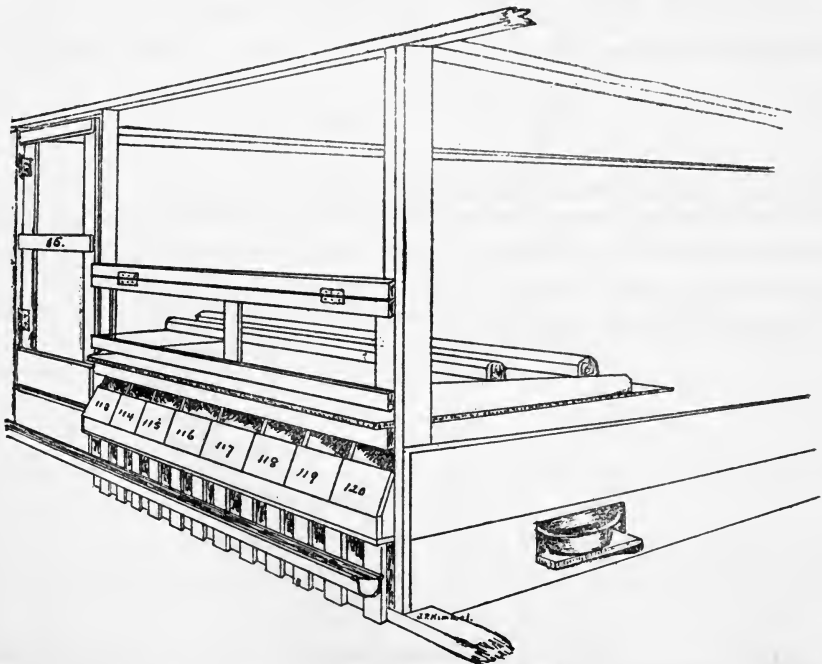
Fig. 28. Section of a Poultry House Arranged to Do all Work from the Walk. (By courtesy of J. P. Kimmel).
