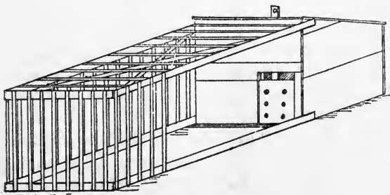
Fig. 44. Convenient Box Coop with Knock-down Pen.
