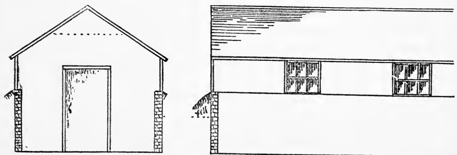
Fig. 29. Incubator Cellar — End and Side Elevations.
