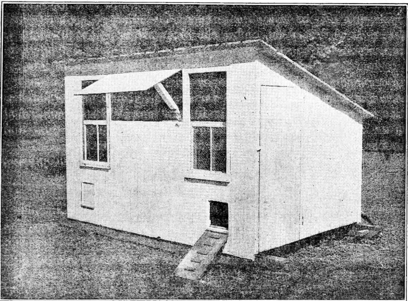
FIG. 1.—House for small flock. Will accommodate any number of fowls up to 25.
