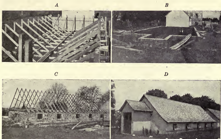
FIG. 156.—Four views showing construction of hollow-tile incubator cellar. A, Forms ready for pouring concrete foundation wall; B, forms removed; C, hollow-tile construction and manner of framing roof; D, completed cellar.
