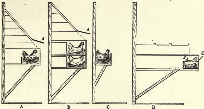
FIG. 95.—Four ways of locating nests,—end boards are removed to show construction. Eggs are taken out from the covered nests by raising the door, d .
