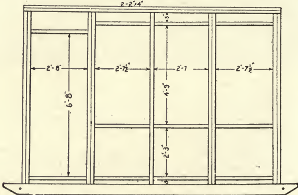
FIG. 92a.—Portable laying house: Working plans.
