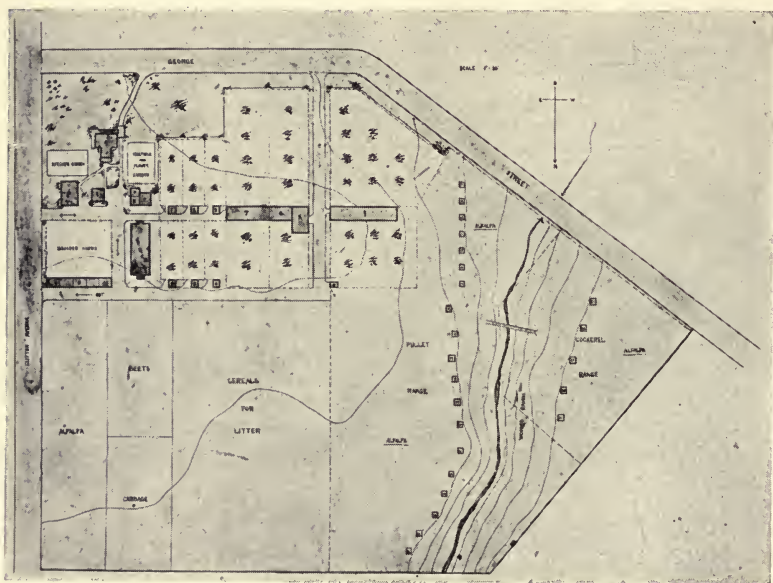
FIG. 217.—A typical plan showing layout of a poultry farm.
