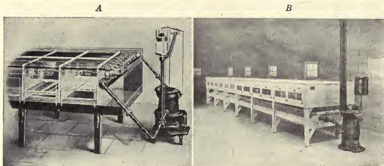
FIG. 158.—Modern mammoth incubators. A , Phantom view showing arrangement of pipes and circulation of water; B , another make of incubator with brooders below. (Photos, A , Hall Mammoth Incubator Co.; B , Candee Incubator Co.)
