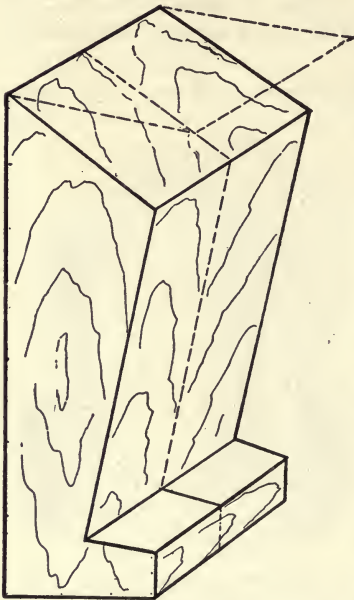
FIG. 104.—A hopper for grit and shell. These materials are usually fed separately—not with dry mash.
