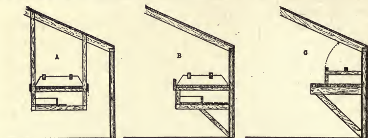
FIG. 93.—Arrangements of nests, perches, and dropping boards. A, suspended; B and C, attached to back wall.
