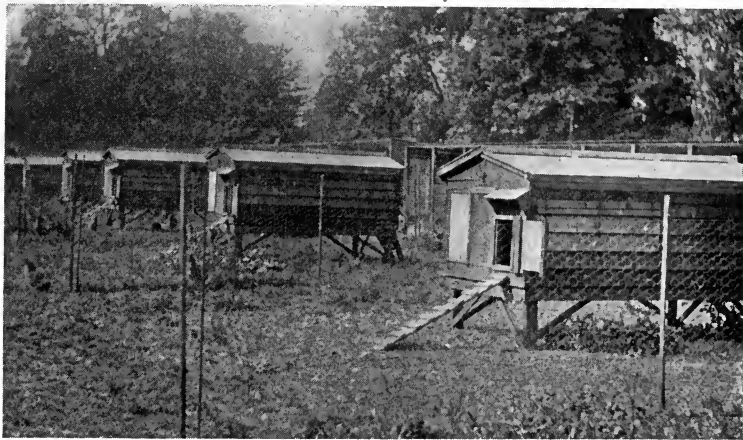
FIG. 27.—An English scene of intensive poultry keeping, with small, elevated, unit houses. (Photo by Edward Brown.)
