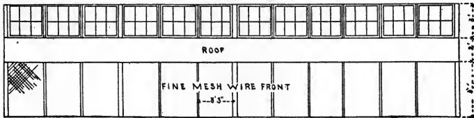
Fig. 91a.—Half-monitor type of laying house; Working plans.
