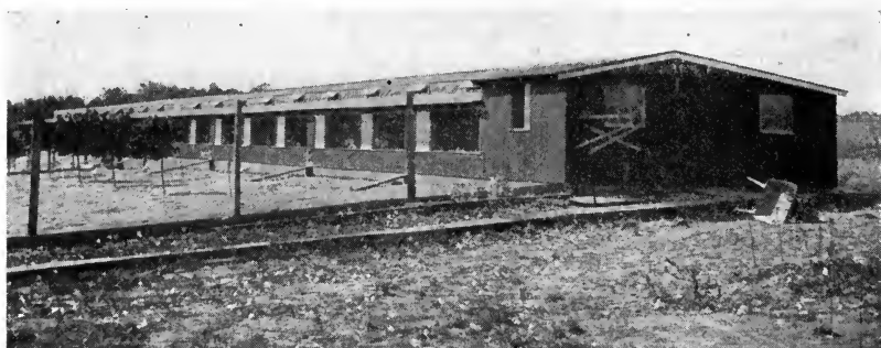
FIG. 32.—Large community house, holding five hundred birds.
