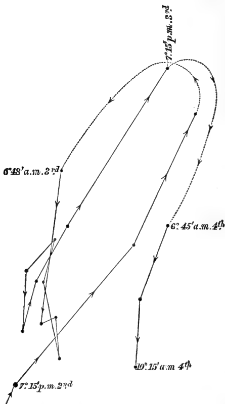
Ficia fabi : circumnutation of leaf, traced from 7.15 P.M. July 2nd to 10.15 A.M. 4th. Apex of the two terminal leaflets 7\frac{1}{4} inches from the vertical glass. Figure here reduced to two-thirds of original scale. Temp. 17^\circ - 18^\circ C.
