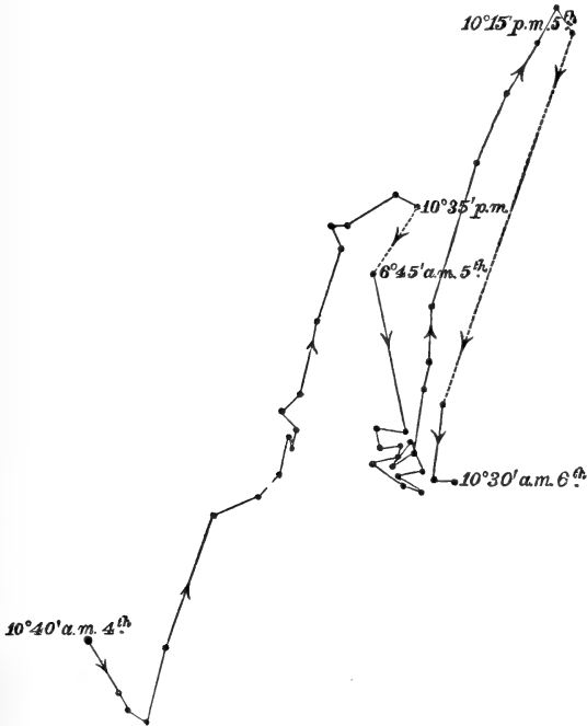
Vicia faba : circumnutation of one of the two terminal leaflets, the main petiole having been secured, traced from 10.40 A.M. July 4th to 10.30 A.M. 6th. Apex of leaflet 6\frac{3}{8} inches from the vertical glass. Tracing here reduced to one-half of original scale. Temp. 16^{\circ} - 18^{\circ} C.
