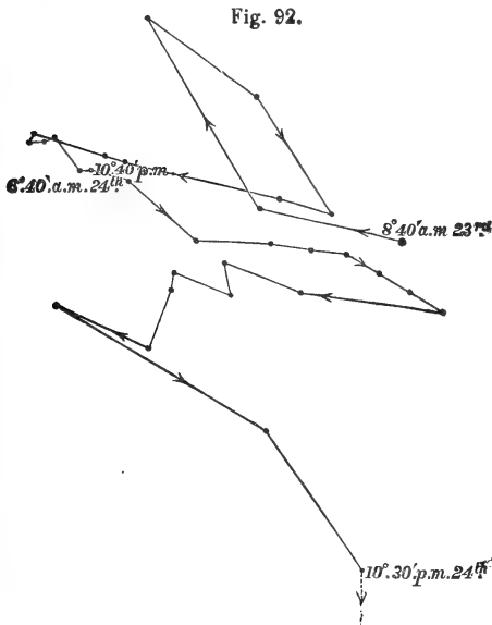
Trifolium subterraneum : main flower-peduncle, illuminated from above, circumnutated traced on horizontal glass, from 8.40 A.M. July 23rd to 10.30 P.M. 24th.
