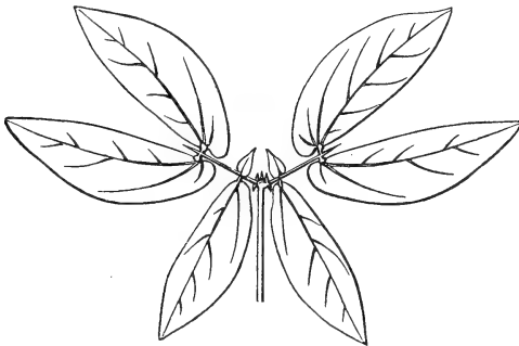
Mimosa albida : leaf seen from vertically above.
