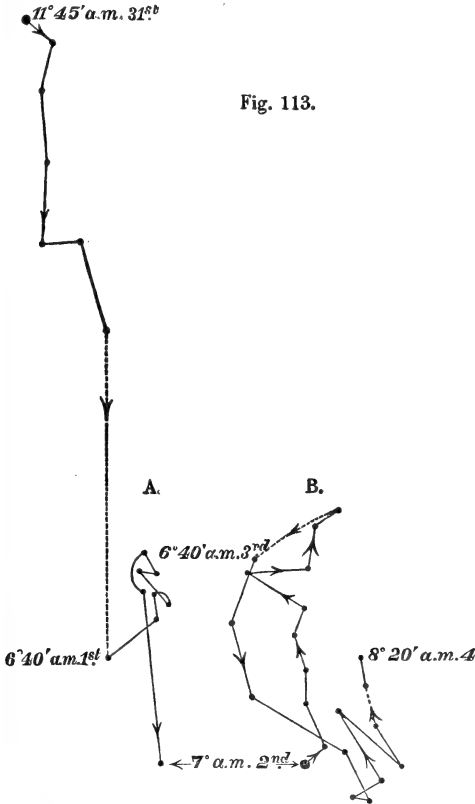
Pinus pinaster : circumnutated of young leaf, traced from 11.45 A.M. July 31st to 8.20 A.M. Aug. 4th. At 7 A.M. Aug. 2nd the pot was moved an inch to one side, so that the tracing consists of two figures. Apex of leaf 14\frac{1}{2} inches from the vertical glass, so movements much magnified.
