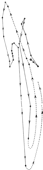
Porlieria hygrometrica : circumnutation and nyctitropic movements of petiole of leaf, traced from 9.35 A.M. July 7th to about midnight on the 8th. Apex of leaf 7½ inches from the vertical glass. Temp. 19½°–20½° C.
