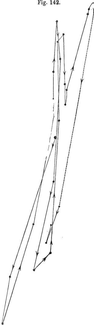
Trifolium subterraneum : circumnutation and nyctitropic movement of terminal leaflet (.68 inch in length), traced from 6.45 A.M. July 4th to 9.15 A.M. 5th. Apex of leaf \frac{3}{8} inches from the vertical glass, and movement, as here shown, magnified 5\frac{1}{4} times, reduced to one-half of original scale. Plant illuminated from above; temp. 16^{\circ} – 17^{\circ} C.
