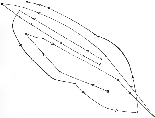
Brassica oleracea ordinary circumnutating movement of the hypocotyl of a seedling plant.
