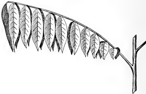
Averrhoa bilimbi : leaf asleep; drawing reduced.
