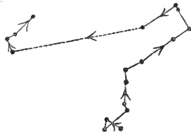
Cucurbita ovifera : circumnutations of arched hypocotyl at a very early age, traced in darkness on a horizontal glass, from 8 A.M. to 10.20 A.M. on the following day. The movement of the bead magnified 20 times, here reduced to one-half of original scale.
