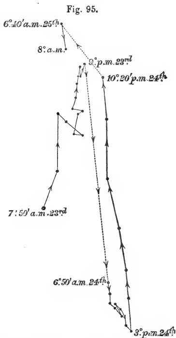
Crambe maritima : circumnutating of leaf, disturbed by being insufficiently illuminated from above, traced from 7.50 A.M. June 23rd to 8 A.M. 25th. Apex of leaf 15\frac{1}{4} inches from the vertical glass, so that the tracing was much magnified, but is here reduced to one-fourth of original scale.
