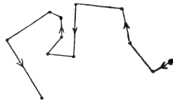
Phalaris Canariensis : circumnutation of a very young cotyledon, with a mark placed below the apex, traced on a horizontal glass, from 11.37 A.M. to 9.30 P.M. Dec. 13th. Movement of apex greatly magnified, here reduced to one-fourth of original scale.
