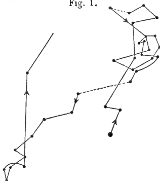
Brassica oleracea : circumnutatation of radicle, traced on horizontal glass, from 9 A.M. Jan. 31st to 9 P.M. Feb. 2nd. Movement of bead at end of filament magnified about 40 times.
