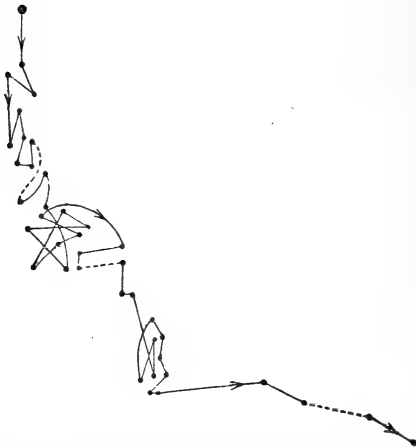
Cyclamen Persicum : downward apheliotropic movement of a flower-peduncle, greatly magnified (about 47 times?), traced on a horizontal glass from 1 P.M. Feb. 18th to 8 A.M. 21st.
