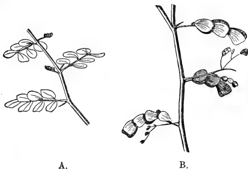
Hamatoxylon Campechianum : A, branch during daytime ; B, branch with leaves asleep, reduced to two-thirds of natural scale.
