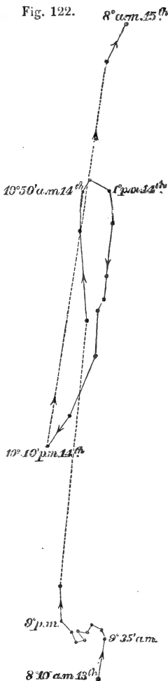
Ampelopsis tricuspidata : hyponastic movement of hooked tip of leading shoot, traced from 8.10 A.M. July 13th to 8 A.M. 15th. Apex of shoot 5½ inches from the vertical glass. Plant illuminated through a skylight. Temp. 17½°-19° C. Diagram reduced to one-third of original scale.
