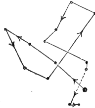
Phalaris Canariensis : circumnutation of a cotyledon, with a mark placed below the apex, traced on a horizontal glass, from 8.35 A.M. Nov. 26th to 8.45 A.M. 27th. Movement of apex magnified 7 times, here reduced to one-half scale.
