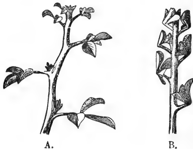
Medicago marina : A. leaves during the day; B, leaves asleep at night.
