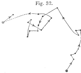
Helianthus annuus : circumnutation of hypocotyl, with filament fixed across its summit, traced on a horizontal glass in darkness, from 8.45 a.m. to 10.45 p.m., and for an hour on following morning. Movement of bead magnified 21 times, here reduced to one-half of original scale.
