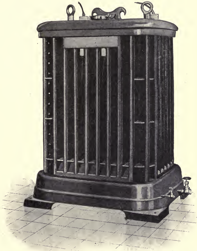
Fig. 14. 150 K.W. Self-Cooled Oil Transformer.
