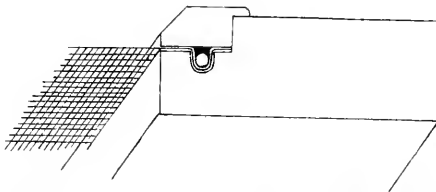
METHOD OF ATTACHING WIRE-GAUZE SCREEN TO FRAMES.
