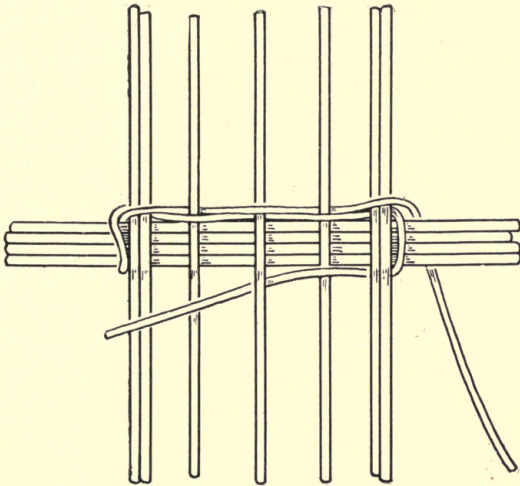
Fig 23.—Showing Two Strands of Rattan.
