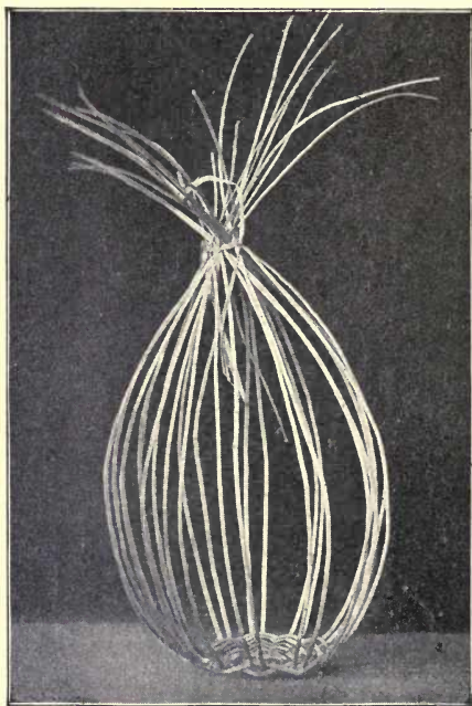
Fig. 29.—Spokes tied together.
