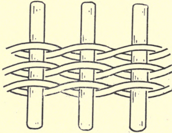
Fig. 10.—Pairing or Twining.
