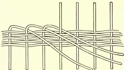
Fig. 18.—Detail of Heavy Border.
