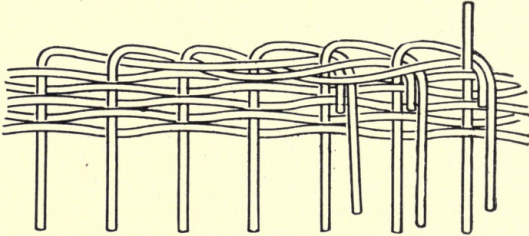
Fig. 19.—Detail of Heavy Border.
