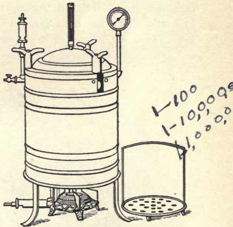
FIG. 76—AUTOCLAV, FOR STERILIZING UNDER STEAM PRESSURE
