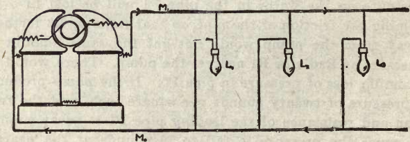
Figure 3 System for distributing electricity at constant pressure.
