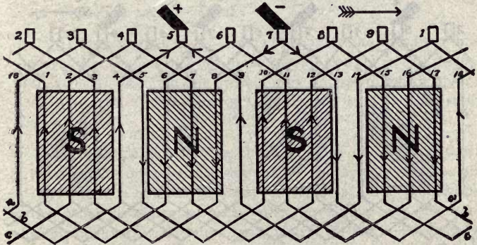
Figure 62 Wave winding on four pole dynamo.
