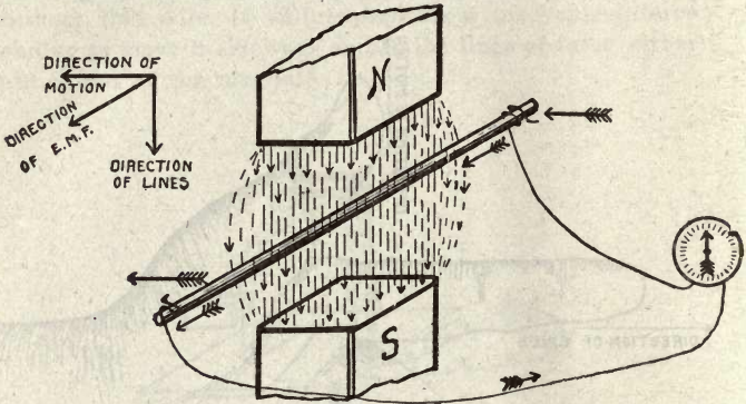
Figure 23 Production of E. M. F. by moving wire in magnetic field.
