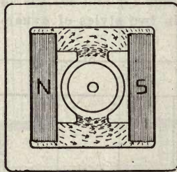
Figure 40 Magnetic leakage in internal pole bipolar frame.
