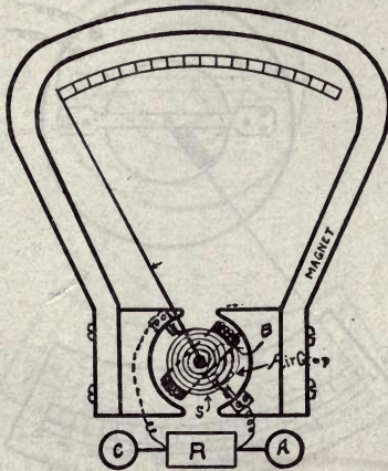
Figure 72 Connection of Weston ammeter.
