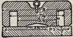
Figure 37 Pull of iron clad magnet.
