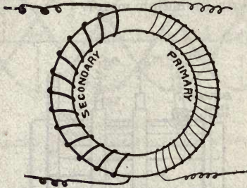
Figure 87 Diagram of alternating current transformer.
