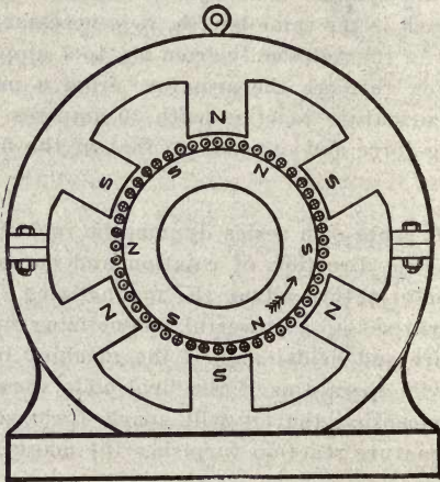
Figure 54 Flow of current in multipolar dynamo.
