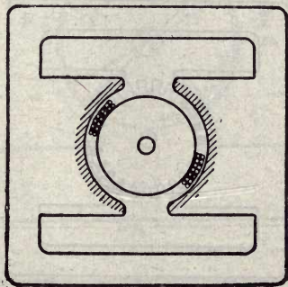
Figure 29 Smooth core armature.
