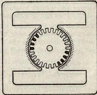
Figure 30 Iron clad armature.
