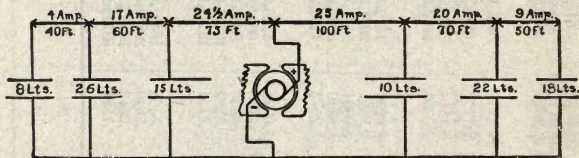
Figure 5 Ordinary lighting circuit.
