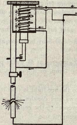
Figure 69 Diagram showing action of series arc lamp
