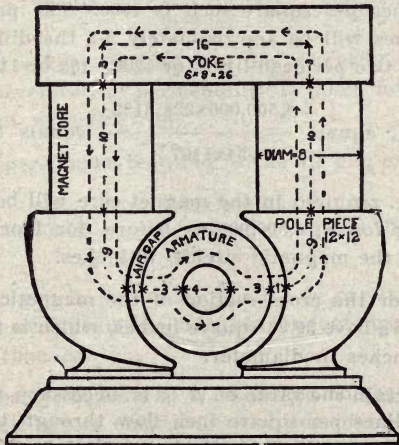
Figure 28 Magnetic circuit of Edison bipolar dynamo.
