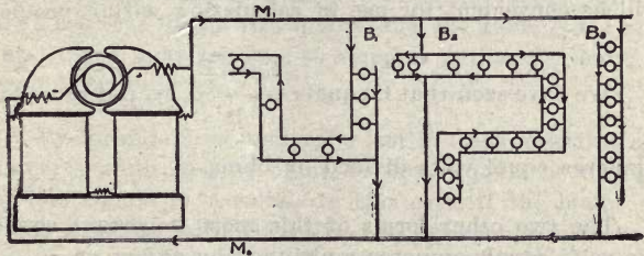
Figure 4 Typical constant potential system.
