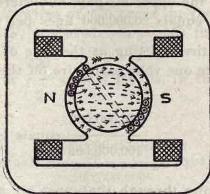
Figure 46 Production of E. M. F. in drum armature.
