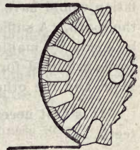
Figure 33 Bunching of magnetic lines in air gap.
