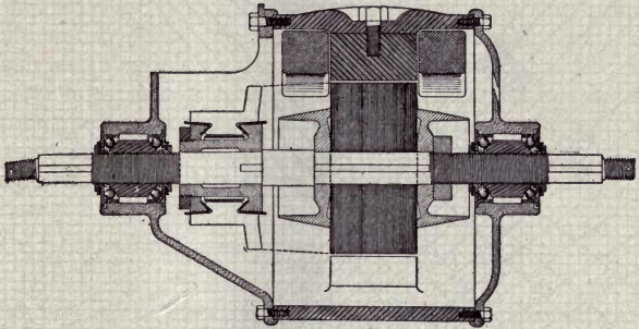
Figure 88 Outline drawing of automobile motor.
