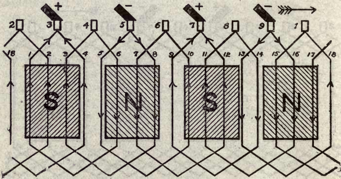
Figure 63 Lap winding on four pole dynamo
