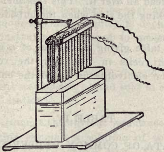
Figure 11 Dip or plunge battery.
