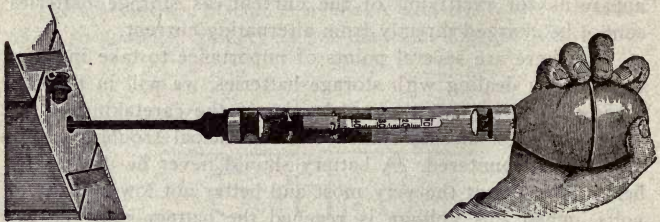
Figure 94 Automobile Hydrometer.
