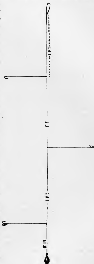
FIG. 87. PATERNOSTER.
