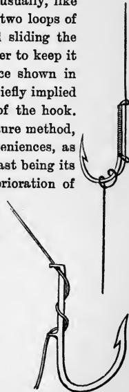
FIG. 31. LIP HOOK WITH BOTH LOOPS ONE WAY.
