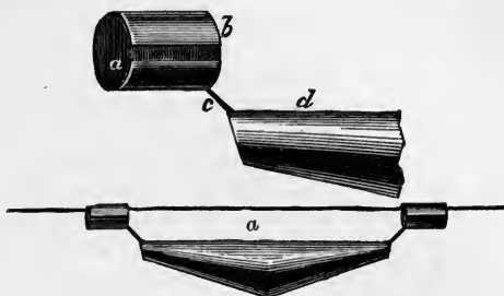
FIG. 56. IMPROVED LEAD.
