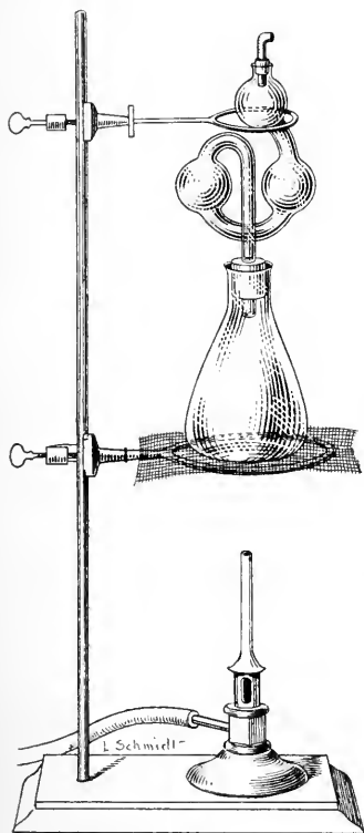
FIG. 159.—FOLIN'S UREA APPARATUS.
