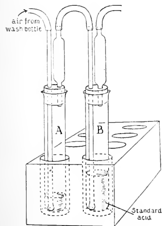
FIG. 158.—VAN SLYKE AND CULLEN APPARATUS.
