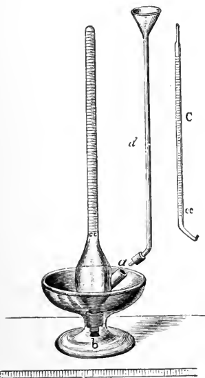
FIG. 161.—MARSHALL UREA APPARATUS. (Tyson.)
