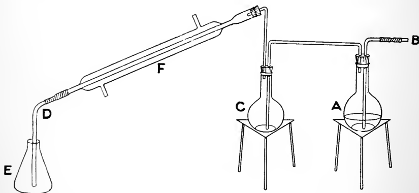
FIG. 168.—SCOTT-WILSON APPARATUS.
