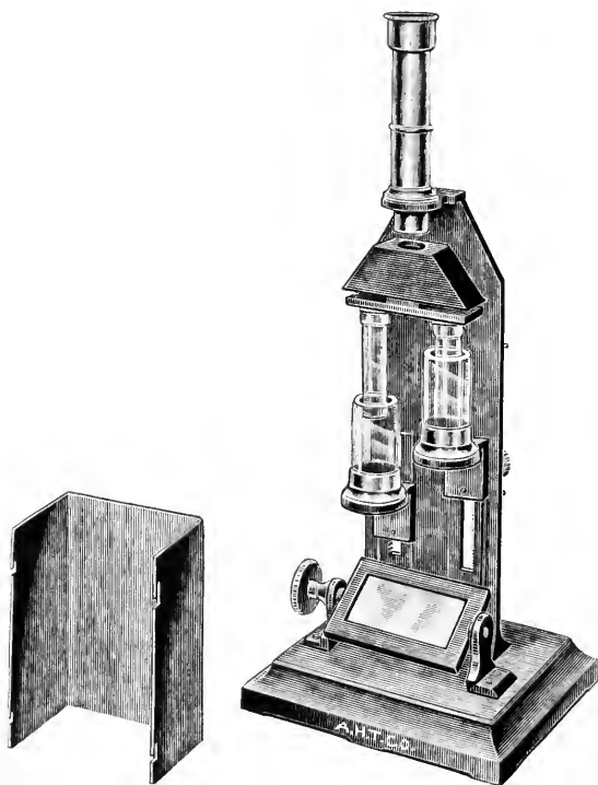
FIG. 153.—DUBOSCQ COLORIMETER.
