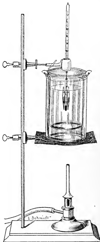
FIG. 54.—MELTING-POINT APPARATUS.
