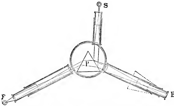
FIG. 88.—DIAGRAM OF ANGULAR-VISION SPECTROSCOPE. (Long.)
