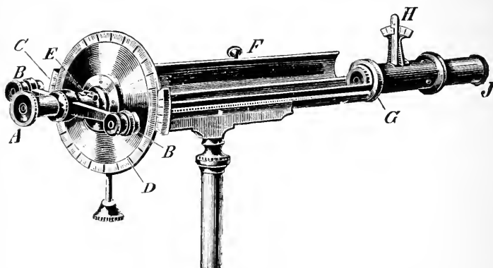
FIG. 5.—ONE FORM OF LAURENT POLARISCOPE.
