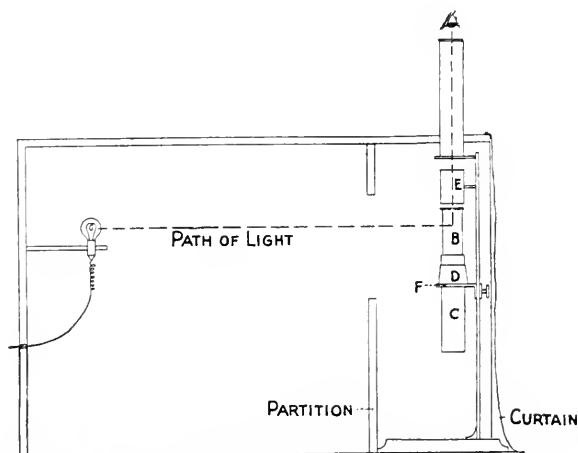
FIG. 84.—NEPHELOMETER IN POSITION, SHOWING RELATION TO SOURCE OF LIGHT.
