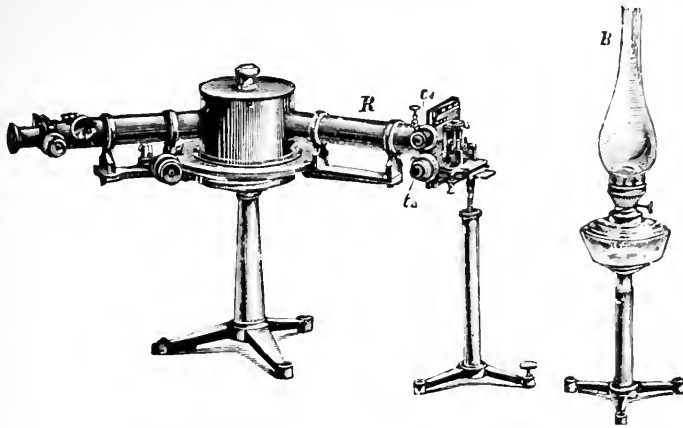
FIG. 87.—ANGULAR-VISION SPECTROSCOPE ARRANGED FOR ABSORPTION ANALYSIS.
