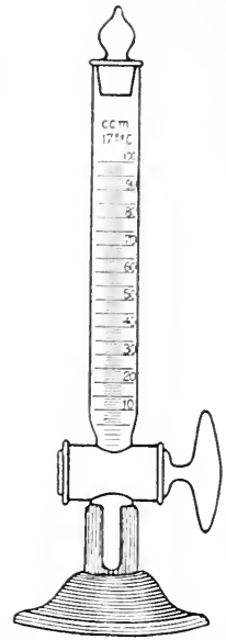
FIG. 166.—HALL'S PURINOMETER.
