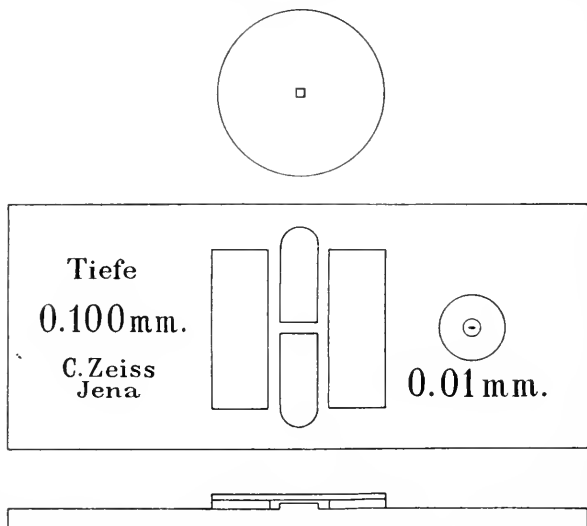
FIG. 102.—BÜRKER COUNTING CHAMBER.
