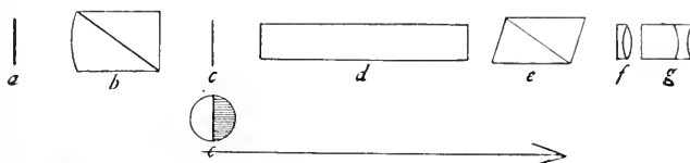
FIG. 6.—DIAGRAMMATIC REPRESENTATION OF THE COURSE OF THE LIGHT THROUGH THE LAURENT POLARISCOPE. (The direction is reversed from that of Fig. 5, p. 32.)
