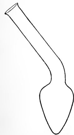
FIG. 157.—GULICK MICRO-OXIDATION FLASK.
