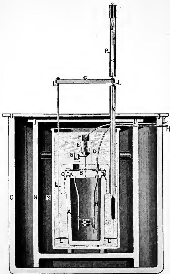
FIG. 172.—BERTHELOT-ATWATER BOMB CALORIMETER.
