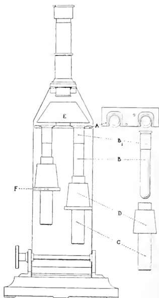
FIG. 83.—BLOOR'S NEPHELOMETER.
