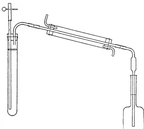
FIG. 156.—BOCK AND BENEDICT APPARATUS.
