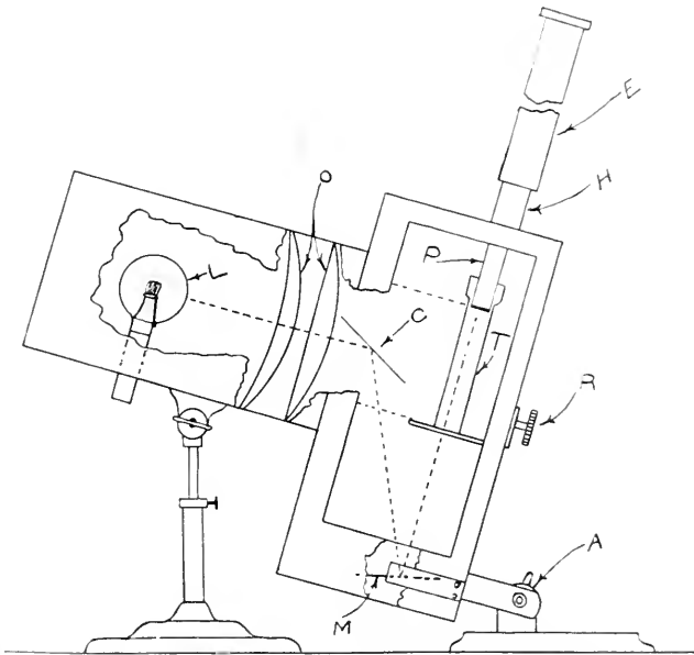
FIG. 85.—LENZMANN-KOBER NEPHELOMETER.
