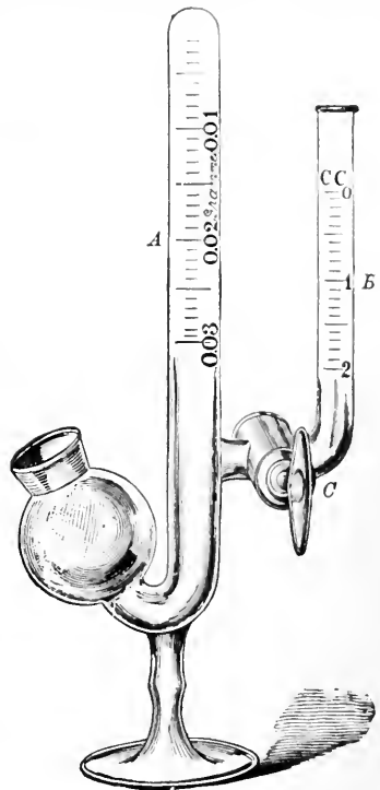
FIG. 160.—DOREMUS-HINDS UREOMETER.
