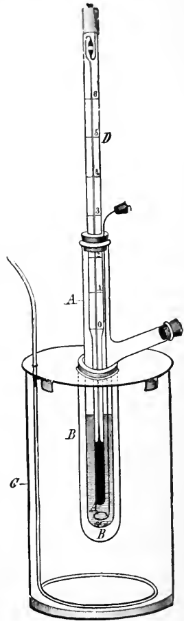
FIG. 117.—BECKMANN-HEIDENHAIN FREEZING-POINT APPARATUS. (Long.)
