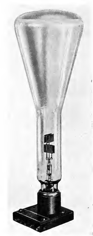
FIG. 65.—The Cathode-ray Tube or Oscillograph.
