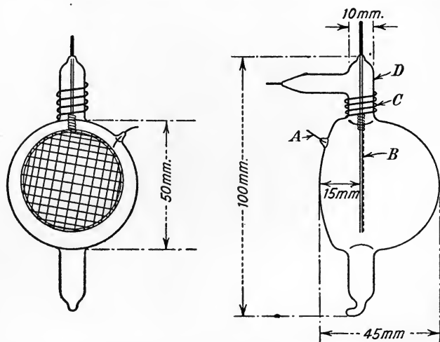
FIG. 44.—The General Electric Co.'s Gas-filled Photo-electric Cell.
