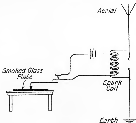
FIG. 24.—Knudsen's Transmitter Circuit.
