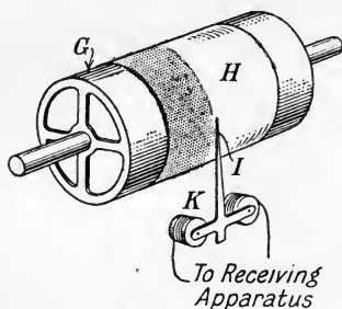
FIG. 26.—Diagrammatic Sketch of Ranger's Receiver.
