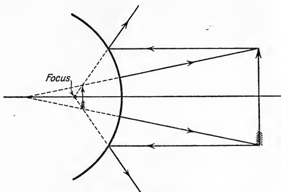
FIG. 75.—Image formed by Convex Mirror.
