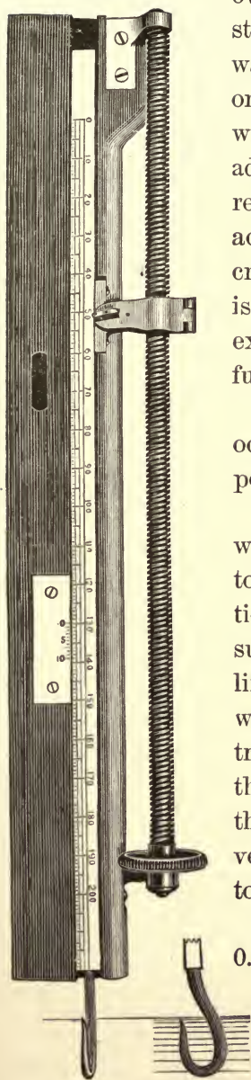
HOOK GAUGE.
