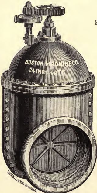
COFFIN'S STOP-VALVE.—(Boston Machine Co., Boston.)
