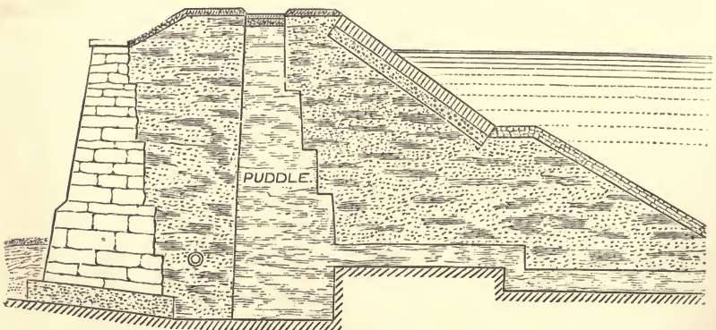
REVETTED RESERVOIR EMBANKMENT.
