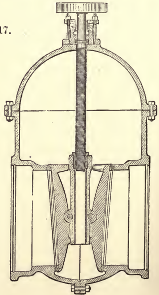
COFFIN'S STOP-VALVE.—(Boston Machine Co., Boston.)
