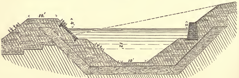
PUDDLED CHANNEL BANK.
