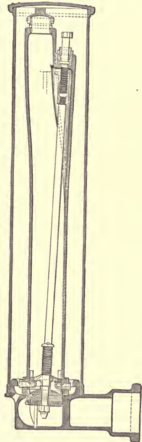
FLUSH HYDRANT.
