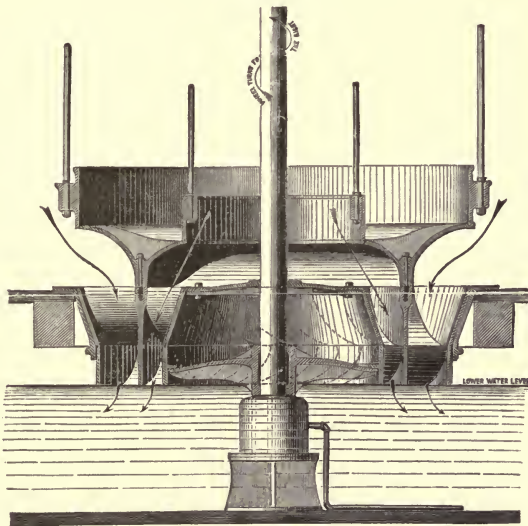
GEVELIN'S DUPLEX-JONVAL TURBINE (R. D. WOOD &amp; CO., PHILA.)
