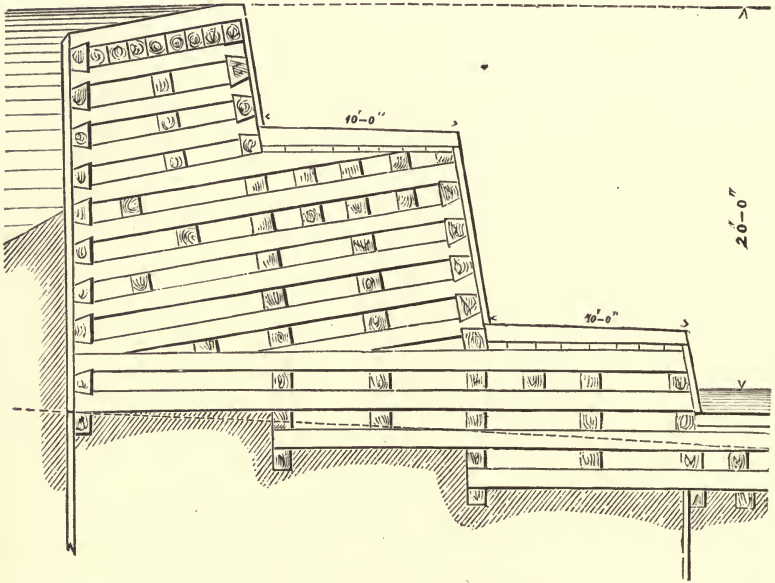
TIMBER CRIB-WEIR.
