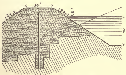
SHEET-PILED CHANNEL BANK.
