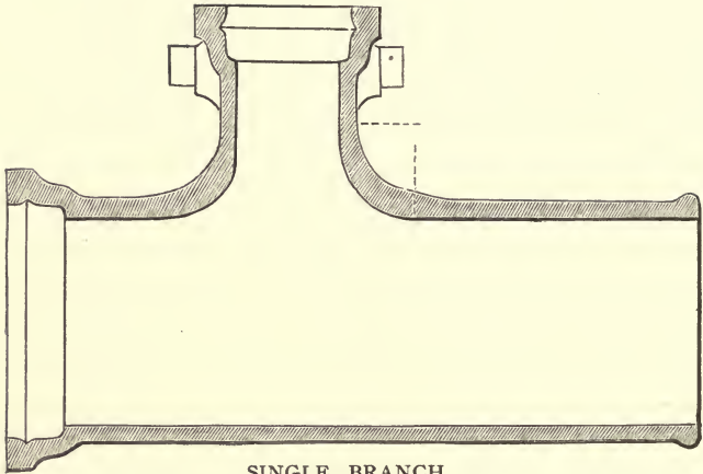
SINGLE BRANCH.
