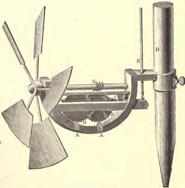
WOLTMANN'S TACHOMETER.
