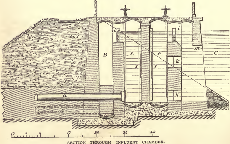
SECTION THROUGH INFLUENT CHAMBER.
