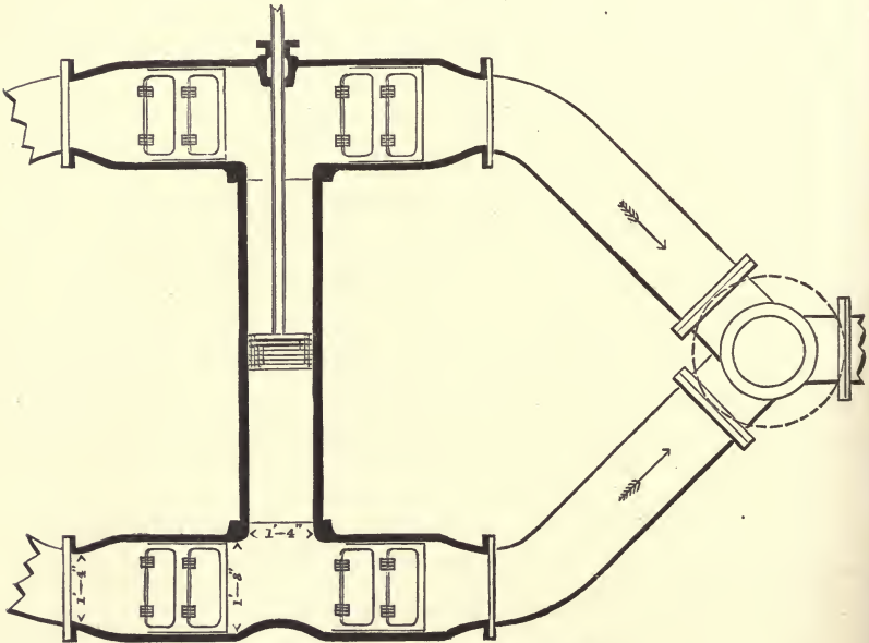
HORIZONTAL DOUBLE-ACTING PISTON PUMP.
