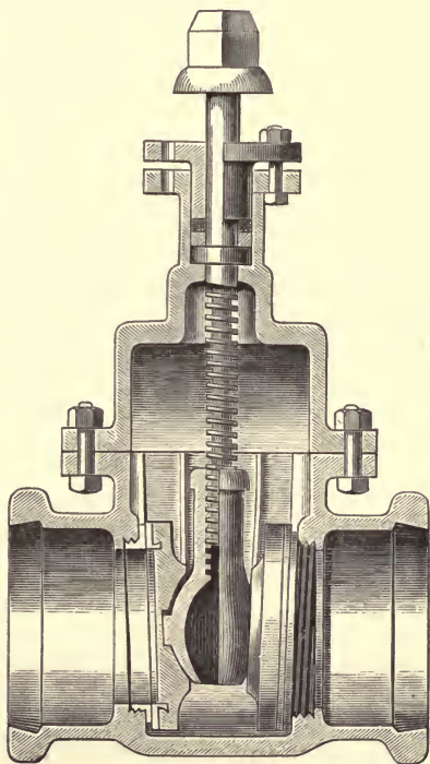
EDDY'S STOP-VALVE.
