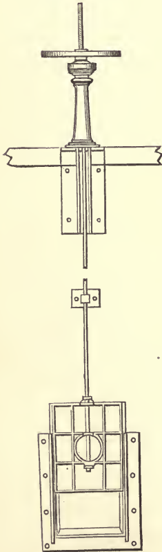
IRON SLUICE-VALVE.
