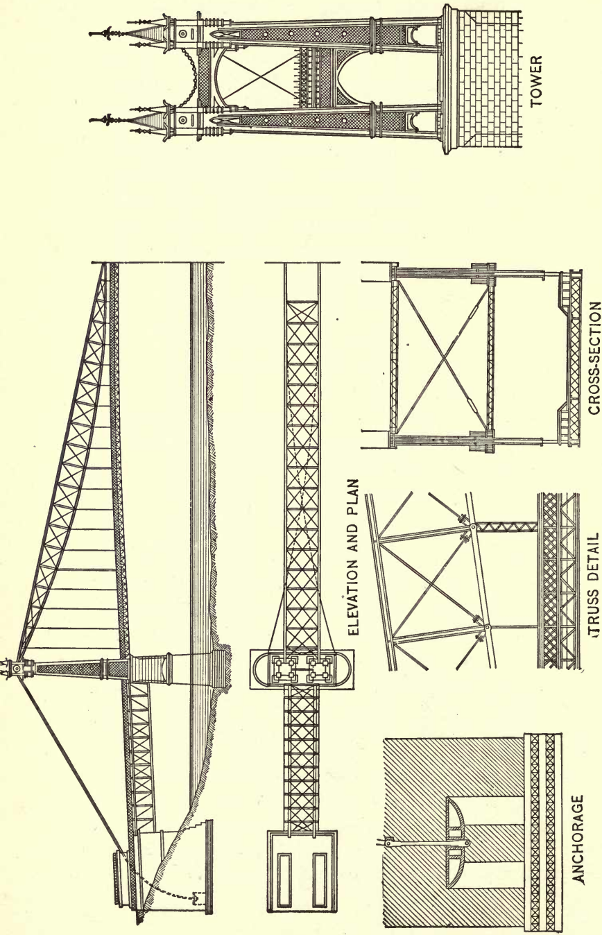
Fig. 38.—Point Bridge at Pittsburgh. (Type 3BLF). Span, 800 feet. Braced Chain. Erected 1877.
