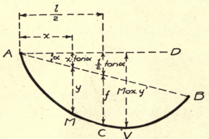
FIG. 2.—Unsymmetrical Parabolic Cable.
