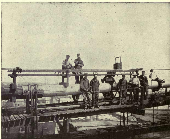
FIG. 55.—Manhattan Bridge. Cable Wrapping Machine.
