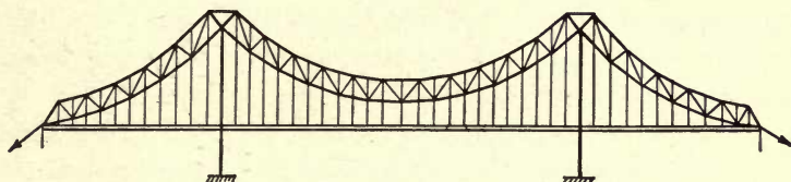
FIG. 24.—Hingeless Braced Chain Suspension Bridge. (Type OB .
