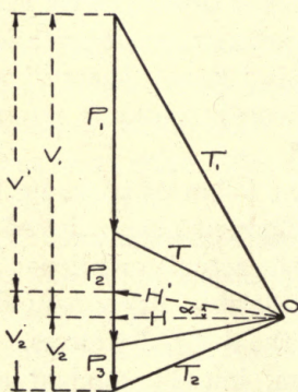
FIG. 7.—Forces Acting on the Stiffening Truss.
