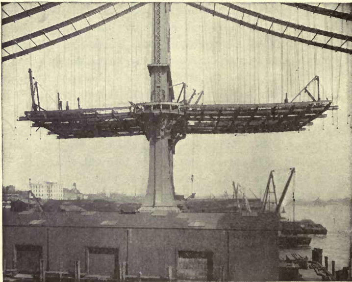
FIG. 50.—Manhattan Bridge. Erection of Lower Chords and Floor System.
