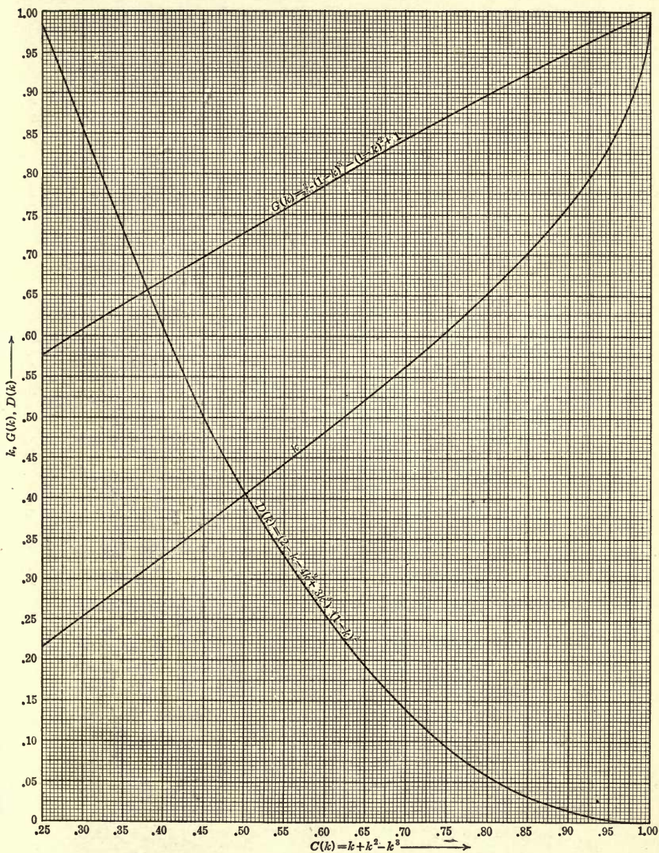
FIG. 13.—Graphs for the Solution of Suspension Bridge Formulas. (Supplementary to Fig. 12).
