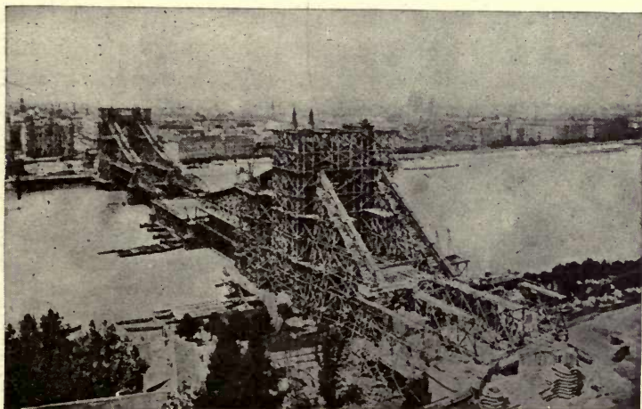
FIG. 58.—Falsework for the Elizabeth Bridge (Eyebar Chains).
