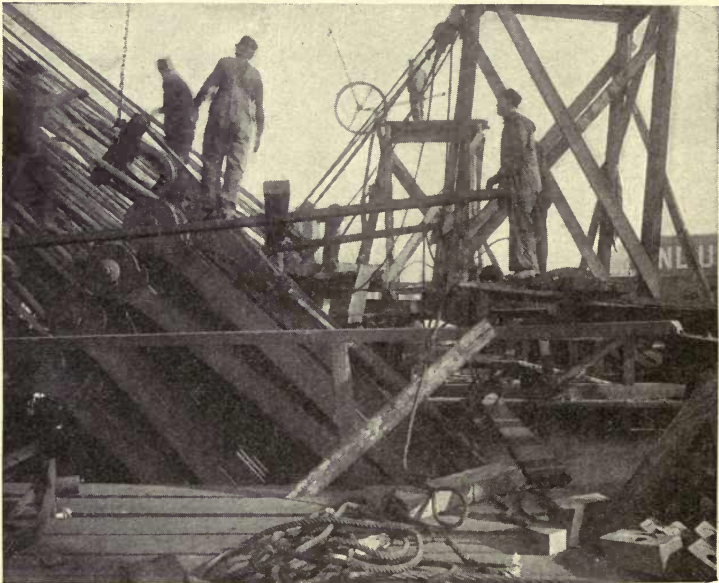
FIG. 49.—Manhattan Bridge. Anchoring a Completed Strand.
