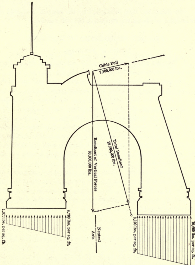
FIG. 44.—Design of Anchorage.
