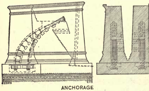
FIG. 32.—Williamsburg Bridge. (Type 2F).
