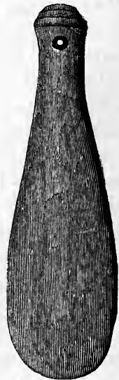
Patoo Patoo.
