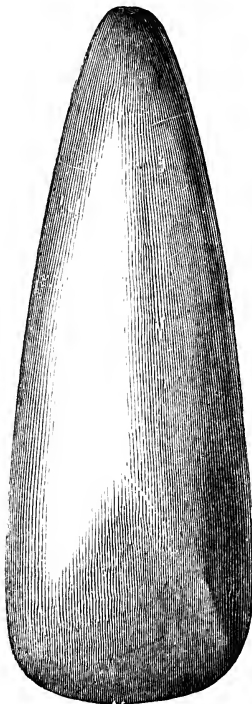
Stone Axes.—Ireland.
