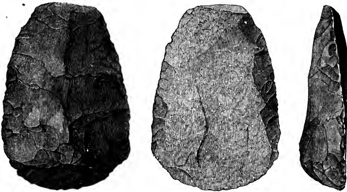
Esquimaux Scraper.
