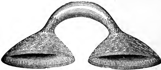
Gold Ornament.—Ireland.
