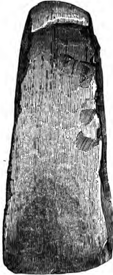
Hollow Chisel.
