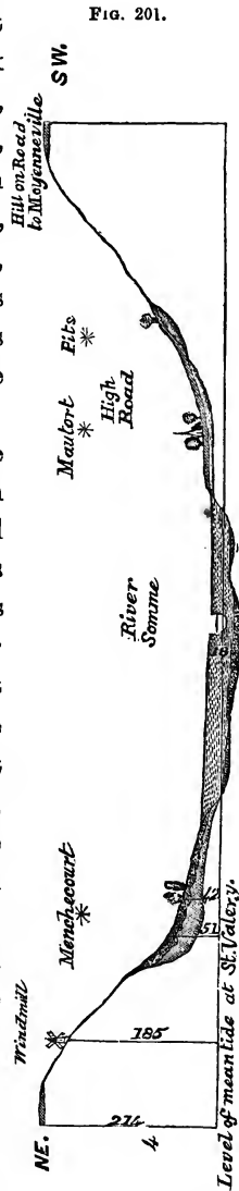
Section across the Valley of the Somme at Abbeville.
