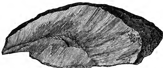
Flint Implement.
