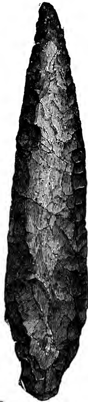
Spear-head.
