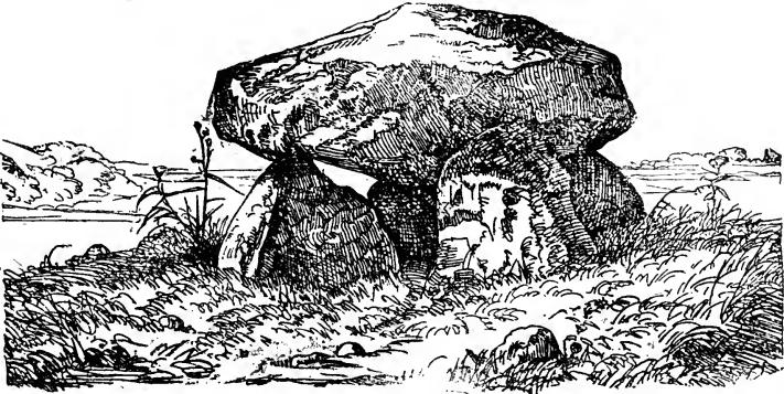
Danish Dolmen.
