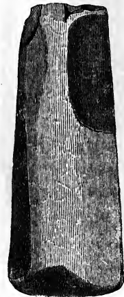
Bone Implement.
