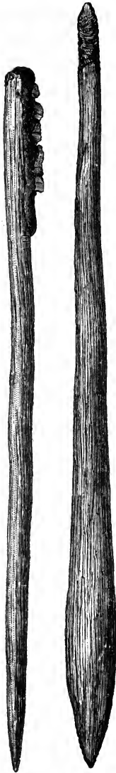
Australian Knife.
