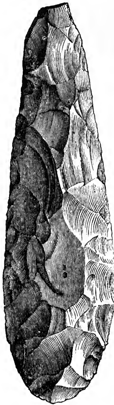
Lance-heads.
