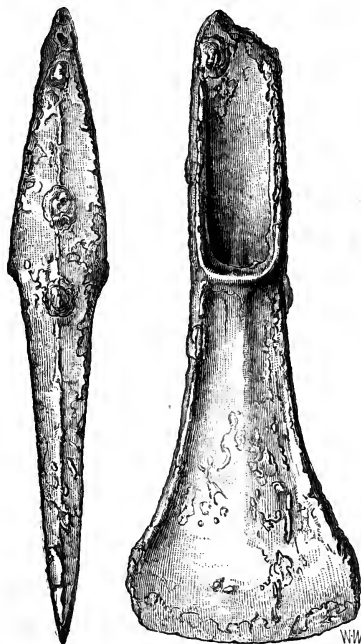
Kentish Celt.
