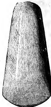
Stone Axes.—Ireland.
