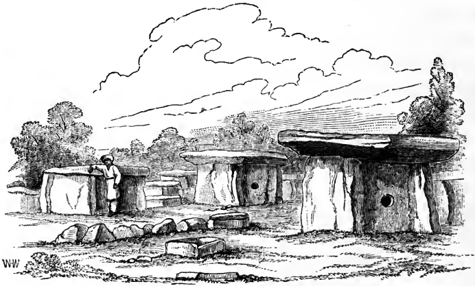
Indian Dolmens.
