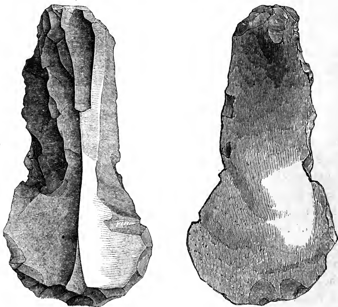
Scraper.
