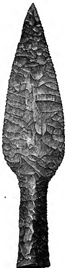
Dagger.
