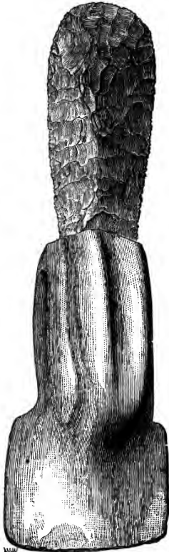
Esquimaux Knife.
