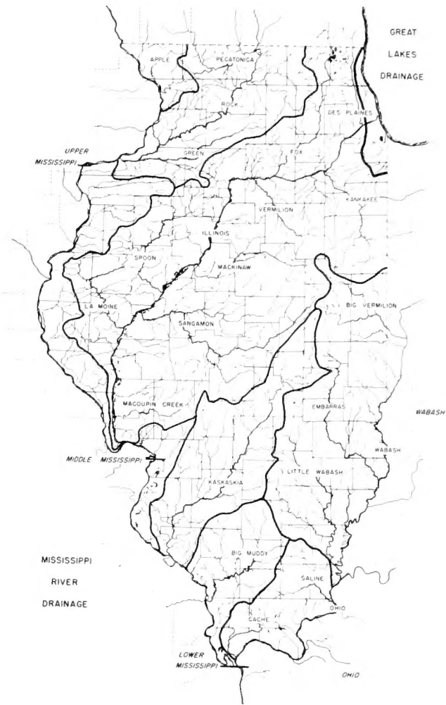
FIG. 2.—Drainage systems and some of the principal streams of Illinois. The heavy curved lines indicate drainage systems of three categories, based on size: (1) the Great Lakes and the Mississippi River; (2) the Wabash, the Ohio, and the Mississippi (Upper, Middle, and Lower); and (3) other rivers named. The short, heavy line to the right of each of the designations Upper Mississippi , Middle Mississippi , and Lower Mississippi shows the downriver limit of one of the three sections of the river as understood in this paper.
