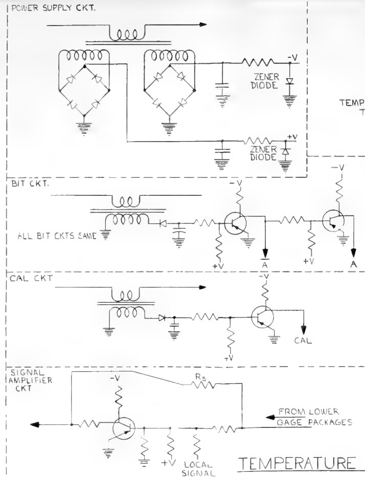
FIGURE 16 TEMPERATURE MEASURING GAGE PACKAGE
