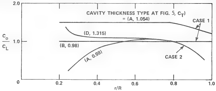
Figure 9 – Camber Distributions for Model 3770
