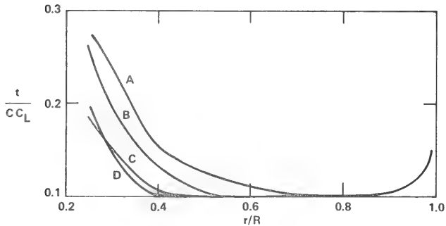
Figure 5 - Leading-Edge Cavity Thickness Distributions at x/c = 0.1 for Model 3770
