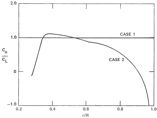
Figure 10 – Camber Distributions for Model 3870
