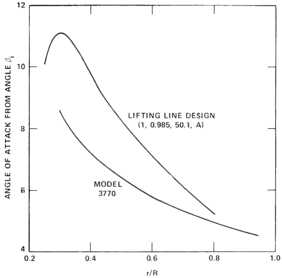
Figure 8 – Angle of Attack from Angle \beta_1
