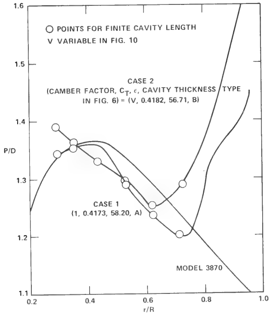
Figure 4 - Pitch Distributions for Model 3870
