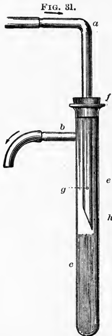
Mercurial thermo-regulator.
