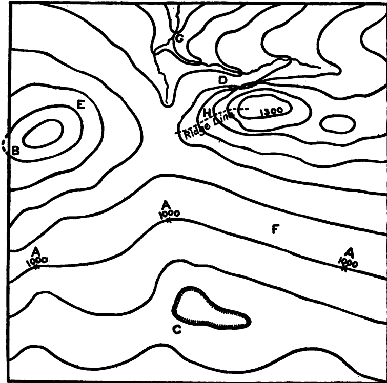
FIG. 121. ILLUSTRATING CHARACTERISTICS OF CONTOURS.
