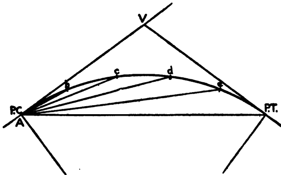
FIG. 103. DEFLECTION ANGLES.
