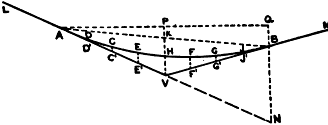
FIG. 108. VERTICAL PARABOLIC CURVE.
