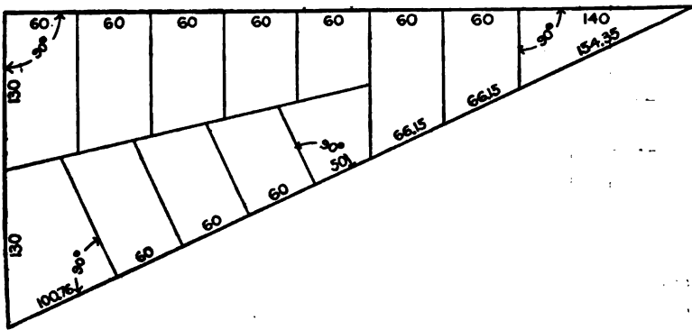
FIG. 112. ARRANGEMENT OF LOTS IN A WEDGE-SHAPED BLOCK.
