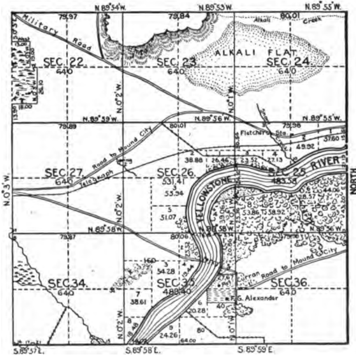
FIG. 59. PORTION OF TOWNSHIP ILLUSTRATING SUBDIVISION OF SECTIONS.
