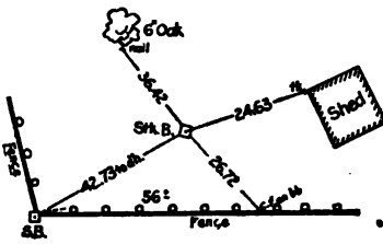
FIG. 55. EXACT TIES.
