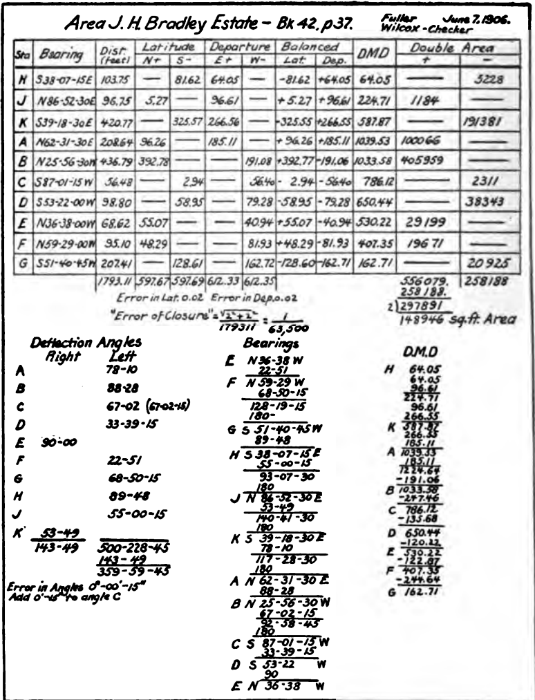
FIG. 161. AREA OF A TRANSIT AND TAPE SURVEY BY DOUBLE MERIDIAN DISTANCE METHOD.
