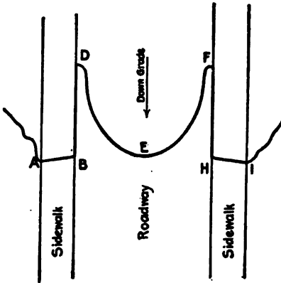
FIG. 120. CONTOUR CROSSING A STREET.
