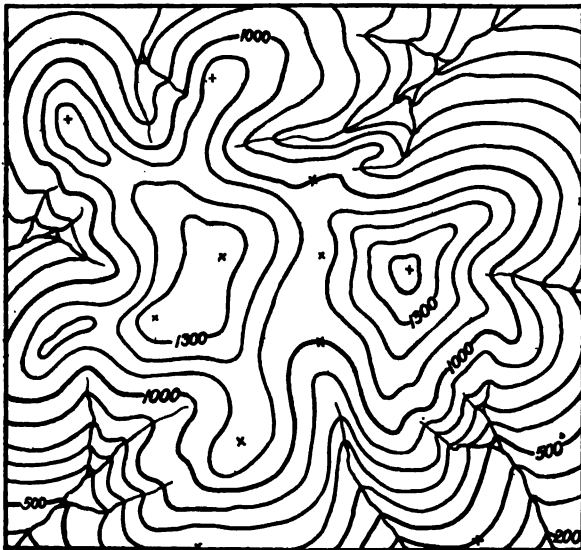
FIG. 127. CONTOURS SKETCHED FROM THE DATA GIVEN IN THE MAP ABOVE.
