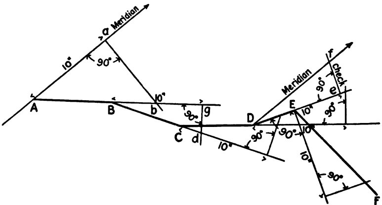
FIG. 177. PLOTTING BY TANGENT OFFSETS.
