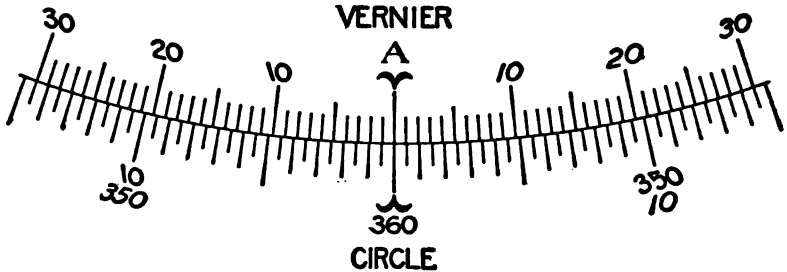
FIG. 20. ONE-MINUTE VERNIER SET AT 0^\circ .
