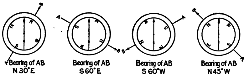
FIG. 4. DIAGRAM ILLUSTRATING READING OF BEARINGS.
