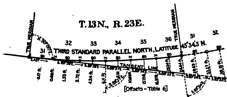
FIG. 61. TANGENT METHOD FOR ESTABLISHING A PARALLEL OF LATITUDE.
