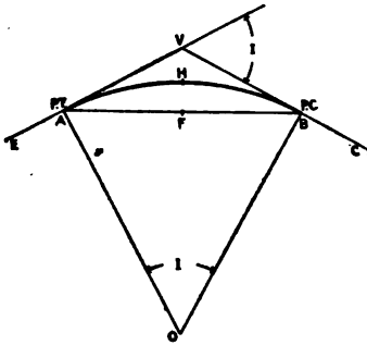
FIG. 102. CIRCULAR CURVE.
