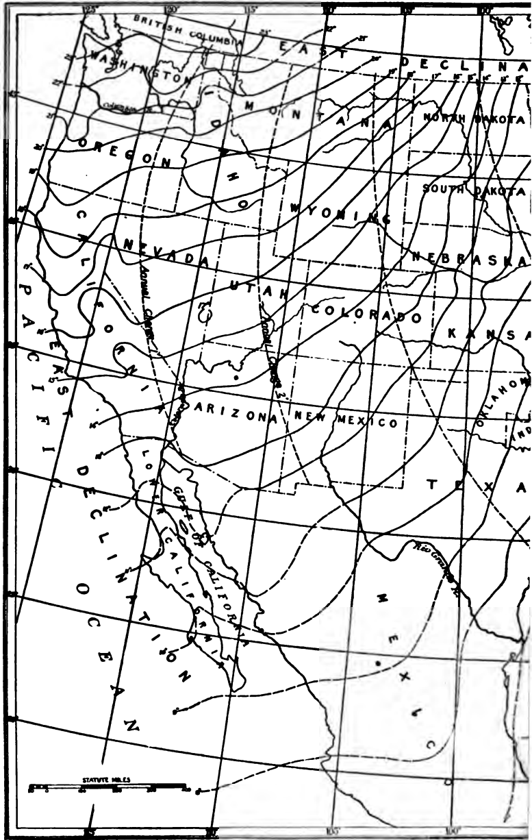
FIG. 5. ISOGONIC CHART OF THE UNITED STATES
