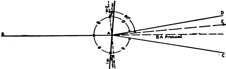
FIG. 81. ADJUSTMENT OF THE CROSS-HAIRS (SECOND PART).
