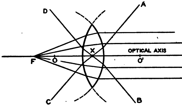
FIG. 15. BI-CONVEX LENS.
