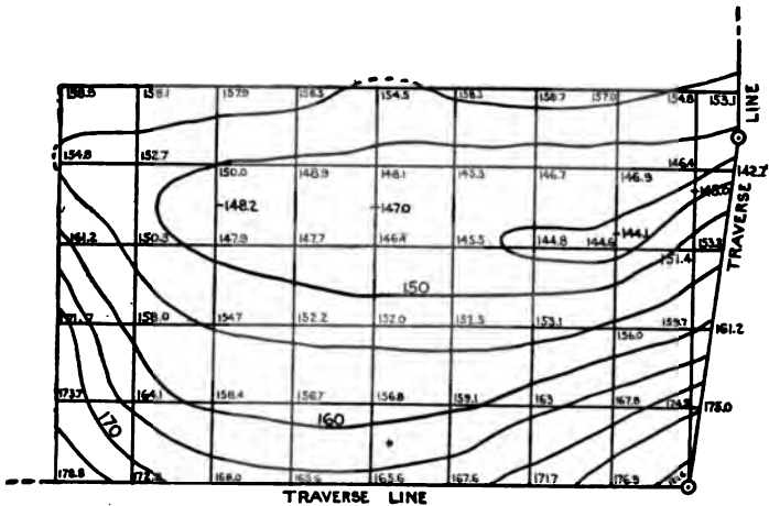
FIG. 125. CONTOUR SKETCHED FOR CROSS-SECTION NOTES.
