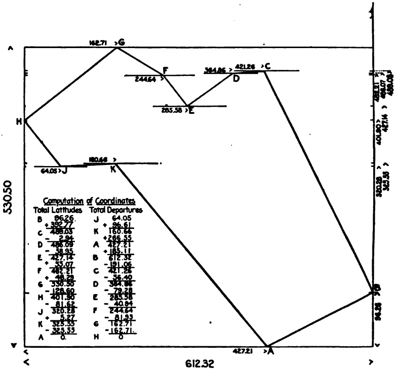
FIG. 176. COMPUTATIONS AND PLOTTING BY RECTANGULAR COÖRDINATES.
