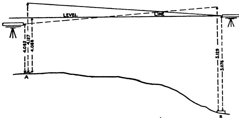
FIG. 48. PEG ADJUSTMENT.
