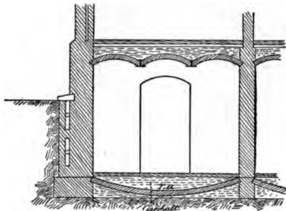
FIG. 57.—Double foundation walls.
