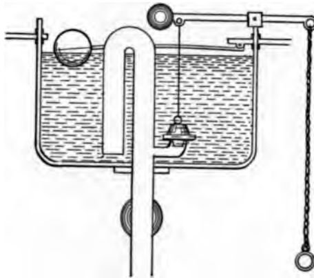
FIG. 34.—Water-waste preventer.
