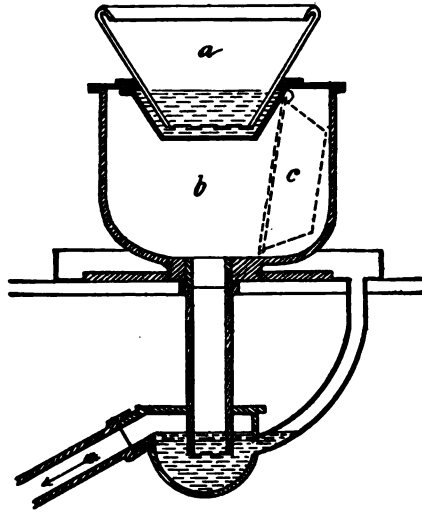
FIG. 30.—Pan closet.
