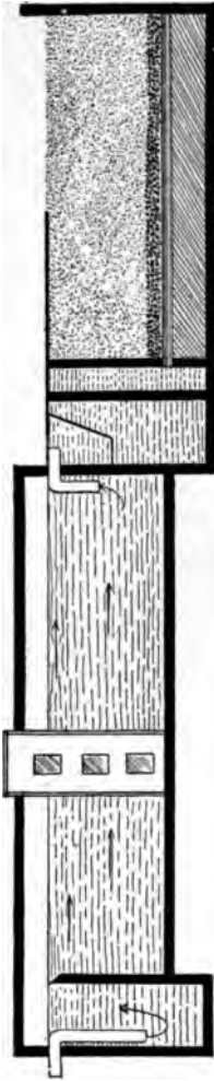
FIG. 45.—Section of septic tank and filter.
