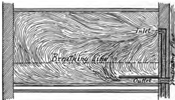
FIG. 16.—Inlet near top, discharge near bottom.
