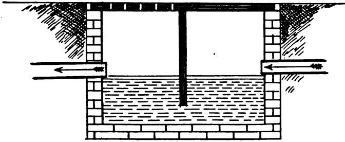
FIG. 39.—Mason's trap.
