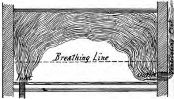
FIG. 15.—Air admitted at bottom, discharged near bottom.
