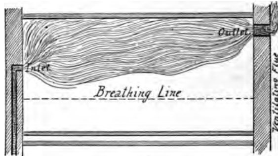
FIG. 12.—Air introduced on side, discharged at top.
