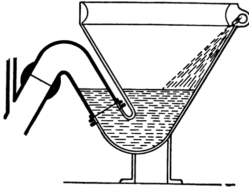
FIG. 33.—Wash-down closet.
