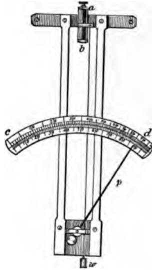
FIG. 4.—The hair hygrometer: a , b , point of suspension of hair; p , pointer; c , d , scale; w , weight.
