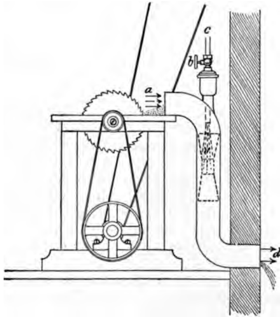
FIG. 19.—Apparatus for removing dust in manufacturing establishments: a , inlet to exhaust shaft; b , valve regulating spray; c , water-supply pipe; d , outlet of exhaust shaft.
