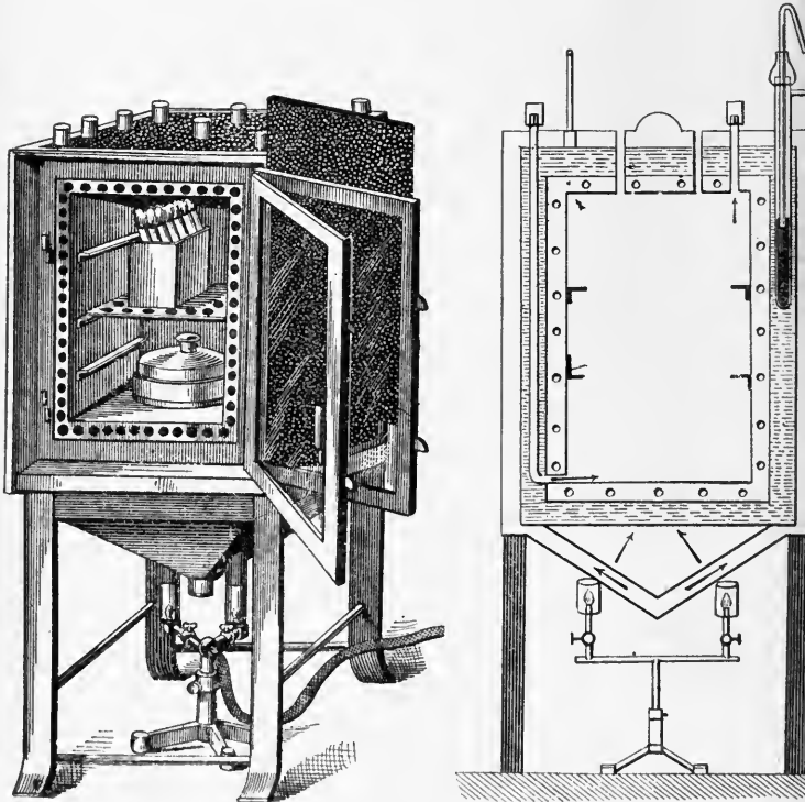
Incubator used in bacteriological work.
