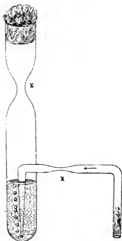
Liborius tube for anaerobic cultures.
