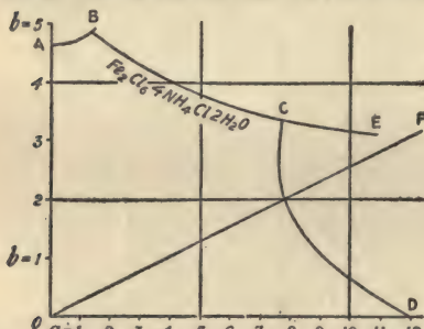
FIG. 98.—Diagram of the formation, at 15^\circ , of the double salt \text{Fe}_2\text{Cl}_6 \cdot 4\text{NH}_4\text{Cl} \cdot 2\text{H}_2\text{O} or \text{Fe}(\text{NH}_4)_2\text{Cl}_4 \cdot \text{H}_2\text{O} . (After Roozeboom.)
