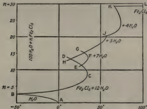
FIG. 95.—Diagram of the solubility of \text{Fe}_2\text{Cl}_6 .
