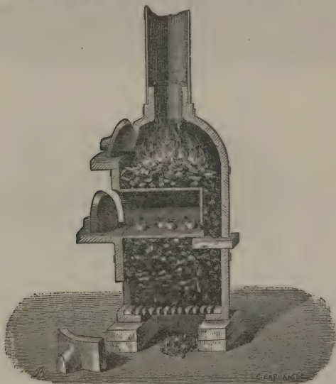
FIG. 97.—Portable muffle furnace
