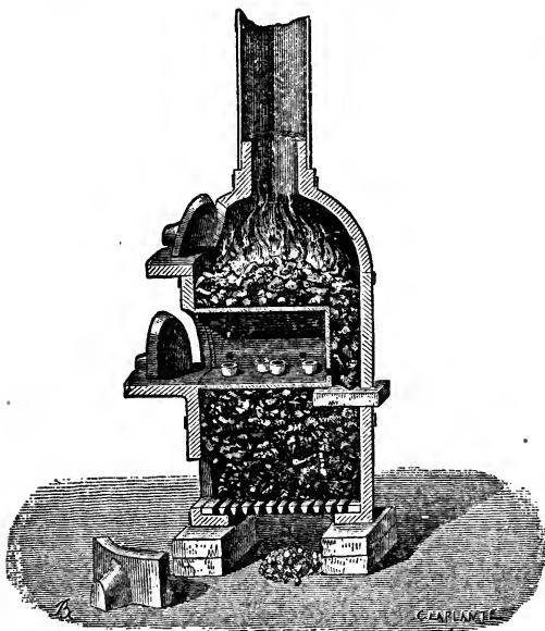
FIG. 97.—Portable muffle furnace
