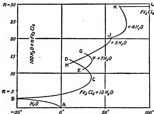
FIG. 95.—Diagram of the solubility of \text{Fe}_2\text{Cl}_6 .
