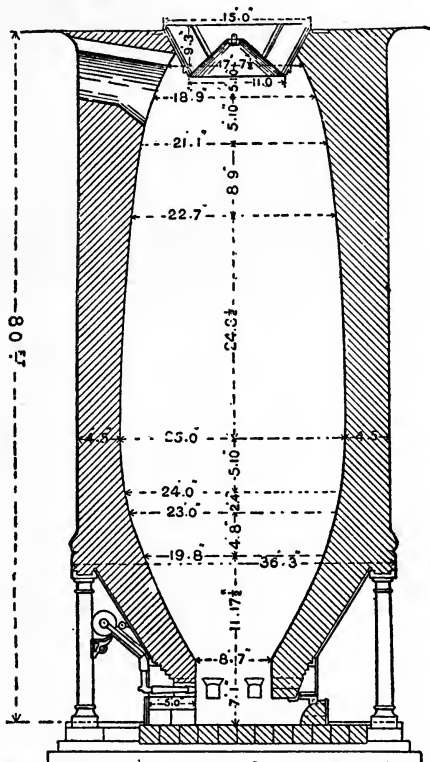
FIG. 93.—Vertical section of a modern Cleveland blast furnace capable of producing 300 to 1,000 tons of pig iron weekly. The outer casing is of riveted iron plates, the furnace being lined with refractory fire-brick. It is closed at the top by a 'cap and cone' arrangement, by means of which the charge can be fed into the furnace at suitable intervals by lowering the moveable cone.
