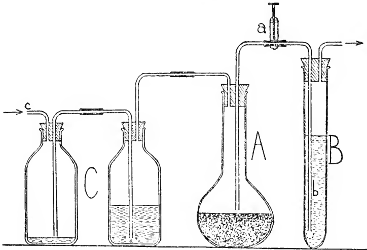
FIG. 60. Method for determining the ability of soil to decompose organic matter (from Waksman and Starkey).
