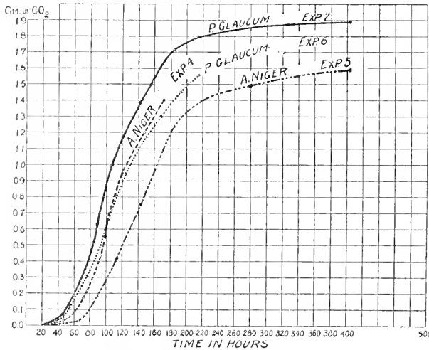
FIG. 14. Rate of \text{CO}_2 production from xylose by two fungi (after Peterson, Fred and Schmidt).
