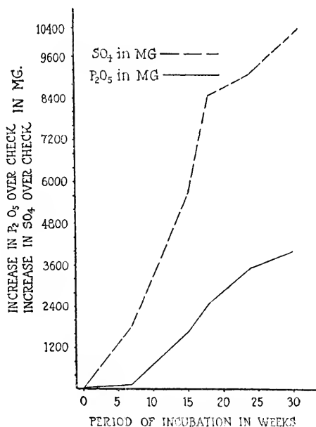
FIG. 43. Course of accumulation of citrate-soluble P_2O_5 and SO_4 in composts of soil-rock phosphate and sulfur (from Lipman, McLean and Lint).
