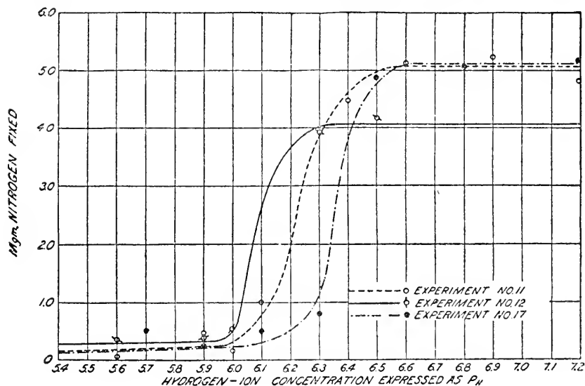
FIG. 41. Influence of reaction of medium upon nitrogen-fixation by Azotobacter (from Gainey and Batchelor).
