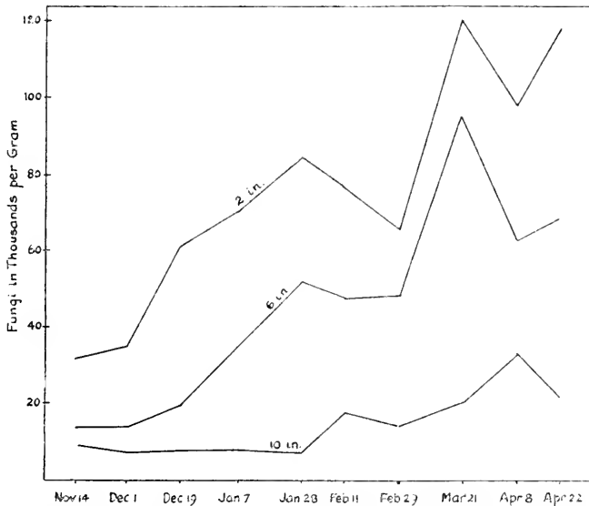
FIG. 4. Variation of numbers of fungi at different seasons of the year and different depths of soil (from Lochhead).
