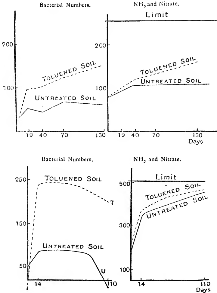
FIG. 68. Influence of toluene upon numbers of bacteria and available nitrogen (ammonia and nitrate) formed in the soil; upper figures from a soil in which small amounts of available nitrogen were initially present; lower figures from a soil in which large amounts of available nitrogen were initially present (after Russell).
