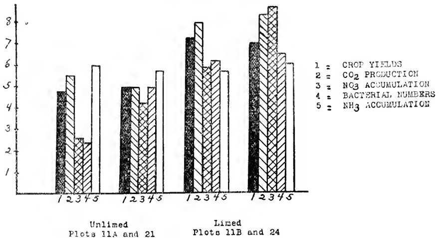
FIG. 61. The correlation between crop yields, \text{CO}_2 -producing power of the soil, bacterial numbers, \text{NH}_3 and \text{NO}_3 accumulation in soil from limed and unlimed plots (from Neller).
