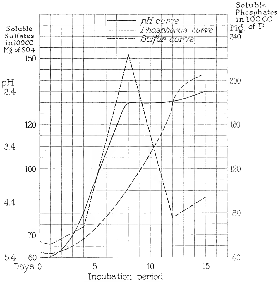
FIG. 44. Course of sulfur oxidation and transformation of insoluble phosphate into soluble forms by Th. thiooxidans in liquid media (from Waksman and Joffe).
