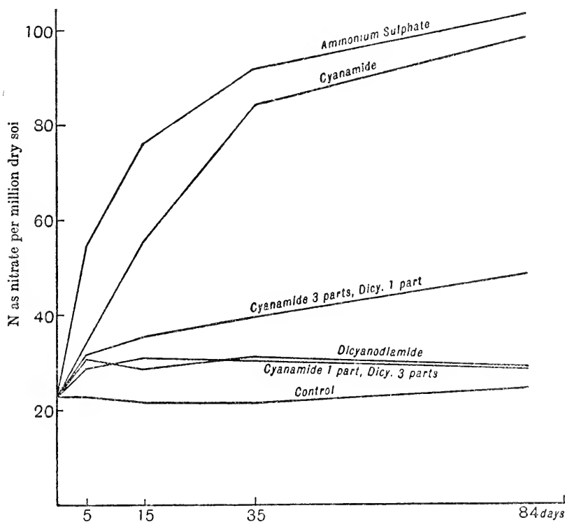
FIG. 34. Influence of dicyanodiamide upon nitrate production in the soil (from Cowie).
