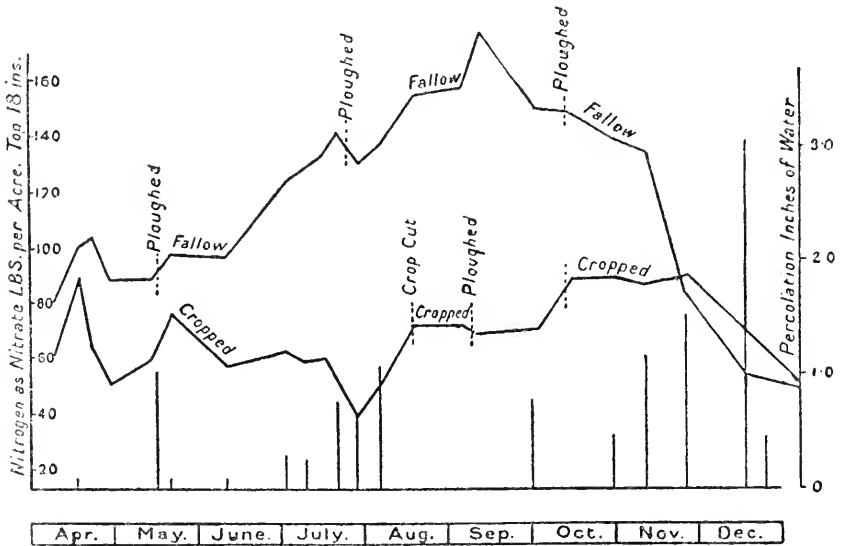
FIG. 75. Influence of cropping and fallowing upon nitrate accumulation at different seasons of the year in the soil (after Russell).
