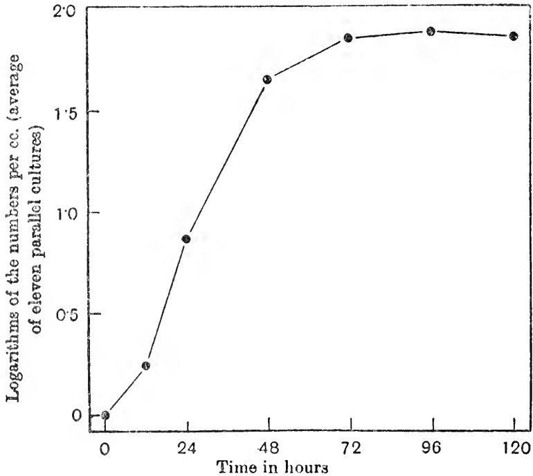
FIG. 12. Rate of increase in numbers of a protozoan (after Cutler and Crump)
