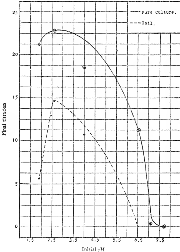
FIG. 46. Influence of hydrogen-ion concentration of medium upon sulfur oxidation by Th. thiooxidans (from Waksman and Starkey).
