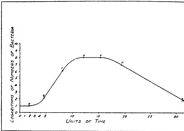
FIG. 11. Rate of increase in numbers of a bacterium (from Buchanan)
