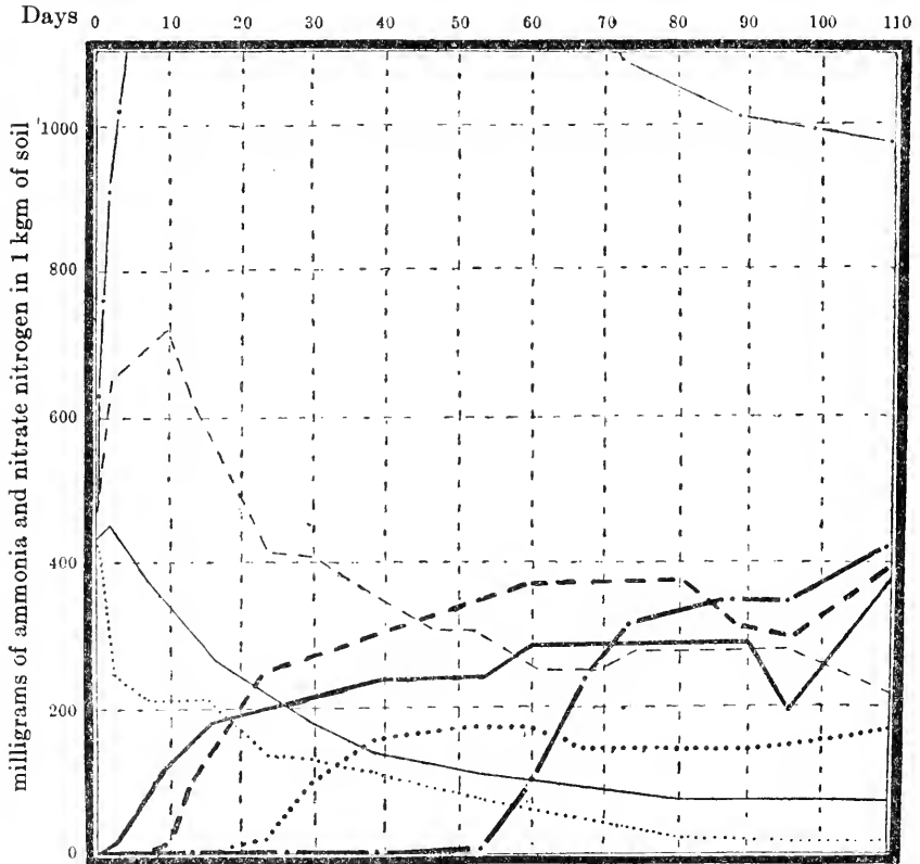
FIG. 33. Influence of organic matter upon the formation of nitrate in the soil: a , soil receiving 0.2 per cent ammonium sulfate, — nitrate N, — ammonia N; b , soil receiving 0.25 per cent peptone, --- nitrate N, --- ammonia N; c , soil receiving 1 per cent peptone, - - nitrate nitrogen, - - ammonia N; d , soil receiving 1 per cent dextrose ••• nitrate N, ..... ammonia N (after Barthel and de Rossi).
