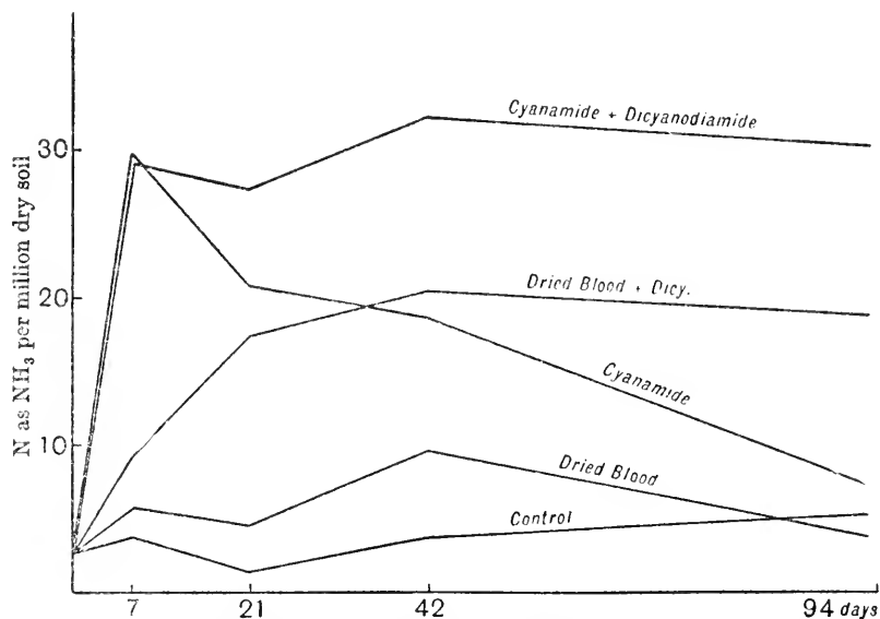
FIG. 26. Accumulation of ammonia from cyanamide and dried blood, as influenced by the presence of dicyanodiamide (from Cowie).
