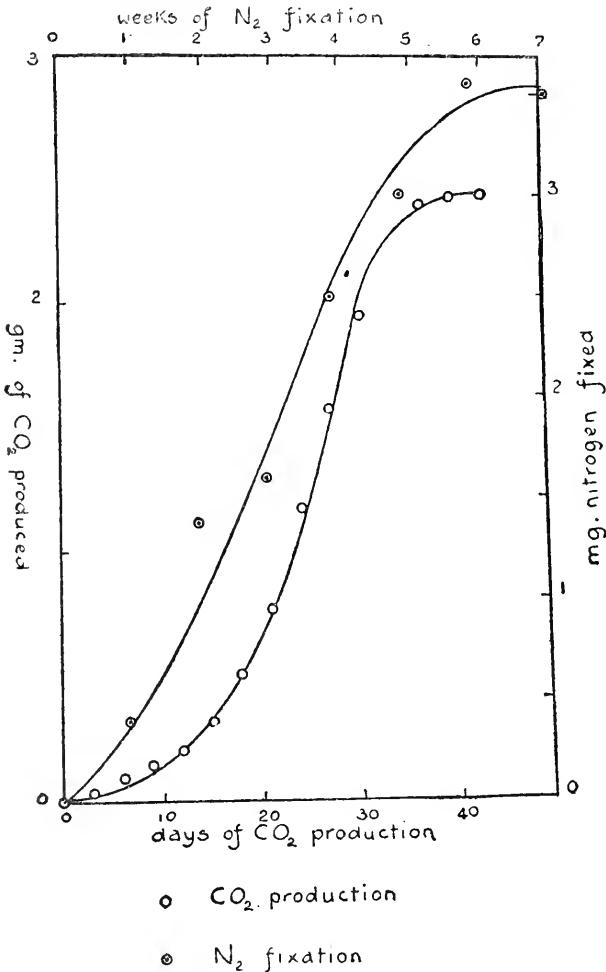
FIG. 40. Rate of nitrogen fixation and energy consumption (after Krainsky and Bonazzi).
