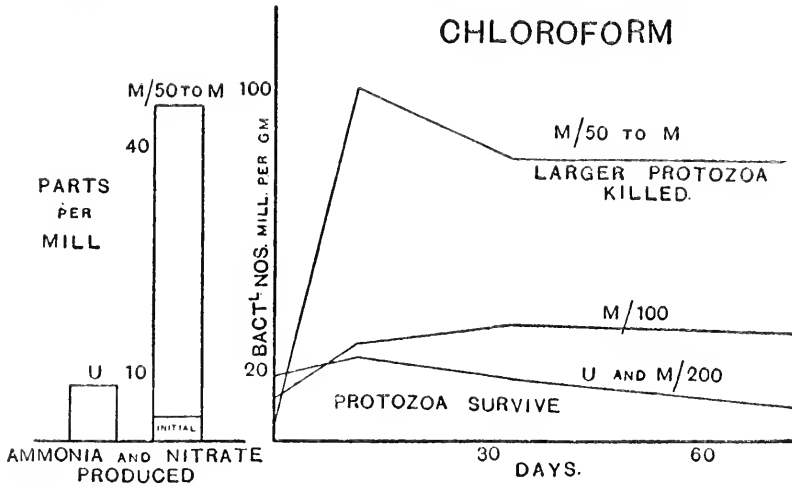
FIG. 67. Influence of different amounts of chloroform upon the bacteria, protozoa and available nitrogen in the soil (from Buddin).
