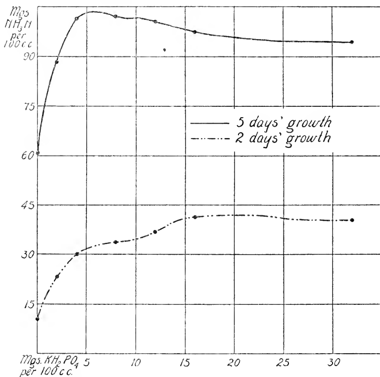
FIG. 51. Influence of \text{KH}_2\text{PO}_4 on the formation of ammonia from peptone by bacteria (from Fred and Hart).
