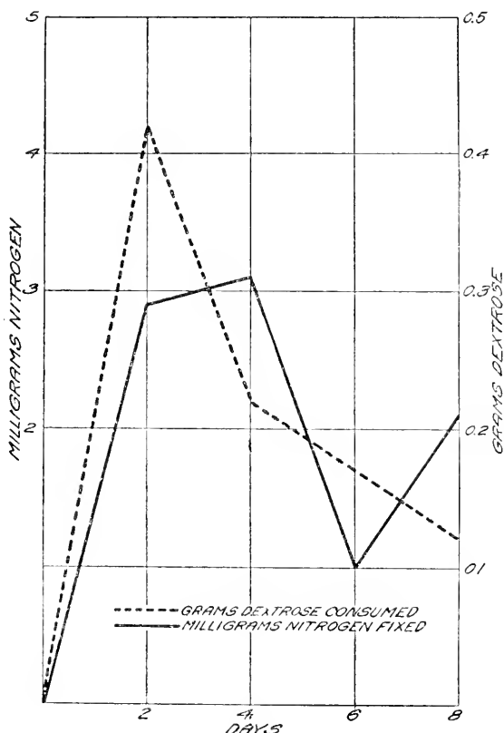
FIG. 39. Rate of decomposition of glucose and fixation of nitrogen by Azotobacter (after Hunter).
