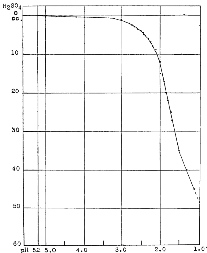
FIG. 50. Hydrogen-ion concentration at which rock phosphate becomes available (from Rudolfs).
