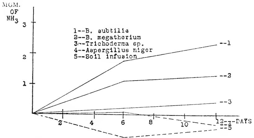
FIG. 33. Rate of decomposition of alfalfa meal by pure cultures of microorganisms and by the mixed soil flora, as indicated by the accumulation of ammonia (from Neller).
