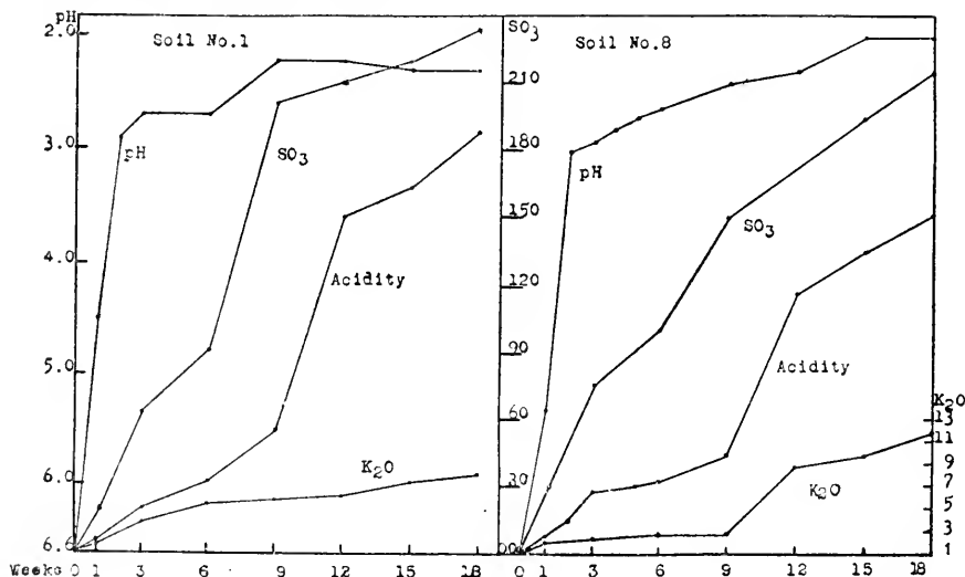
FIG. 47. Relation between sulfur oxidation and water-soluble potassium in composts containing sulfur and greensand marl (from Rudolfs).
