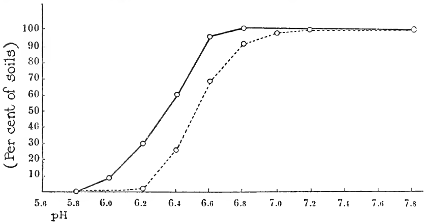
FIG. 42. A correlation between soil reaction and the presence of Azotobacter : ——— positive test; ----- abundant growth of Azotobacter (from Christensen).
