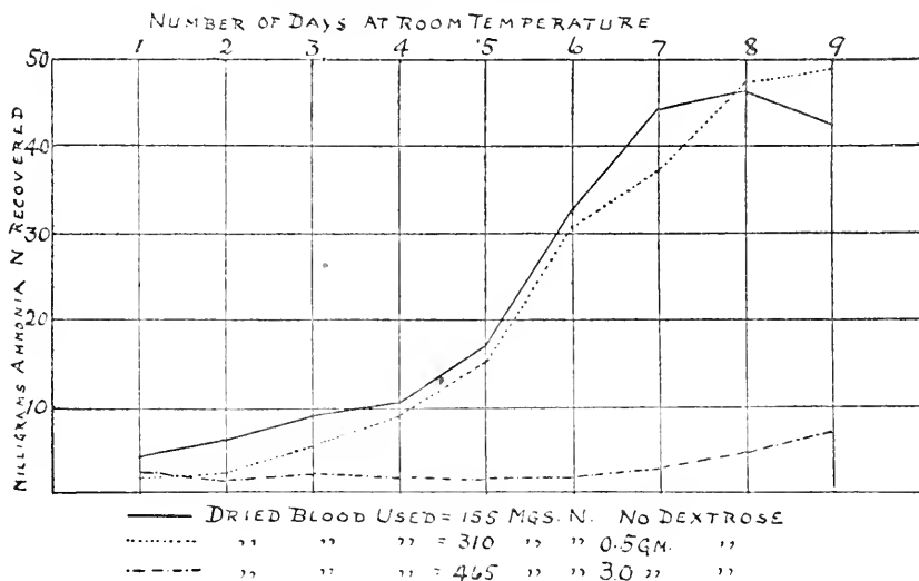
FIG. 30. Influence of glucose on ammonia accumulation from dried blood added to soil (after Lipman and associates).
