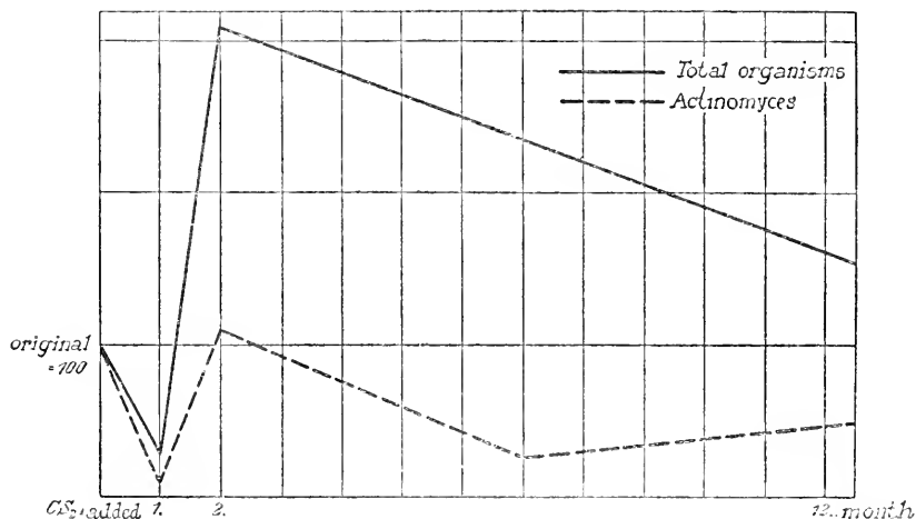
FIG. 66. Influence of \text{CS}_2 upon the numbers of bacteria and actinomyces in the soil (from Hiltner and Störmer).
