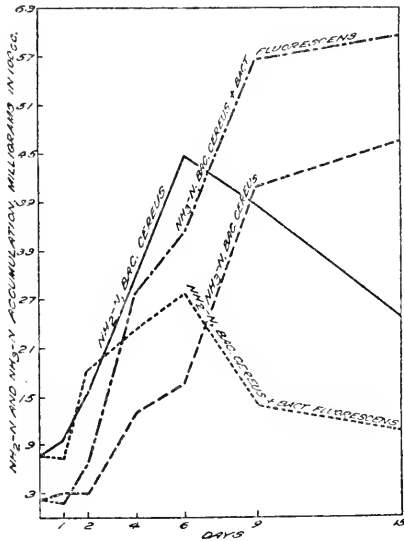
FIG. 27. Course of accumulation of amino- and ammonia-nitrogen from casein by Bac. cereus and Bact. fluorescens (from Waksman and Lomanitz).
