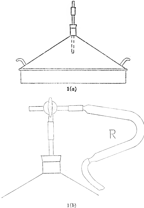
FIG. 58. Apparatus for determining the \text{CO}_2 -production in field soil: a , Zinc bell, in side view; b , arrangement for taking sample ( R = Recipient) (from Lundegardh).
