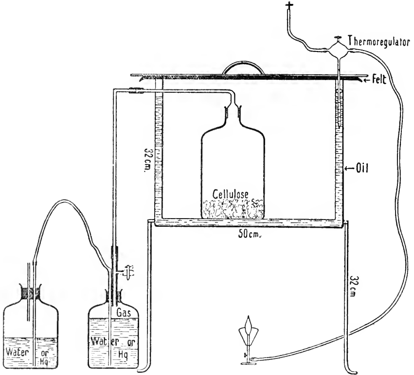
FIG. 23. Apparatus for study of cellulose decomposition, under anaerobic conditions (after Pringsheim).
