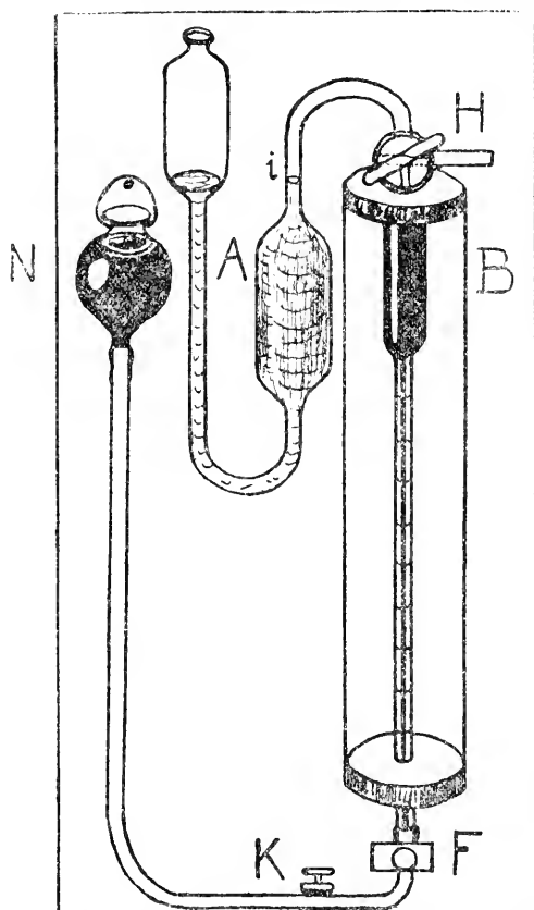
FIG. 59. Gas analysis apparatus: B , gas burette; H , three way stop cock; A , potash apparatus (30 per cent KOH); i , index; N , mercury vessel; F , fine adjustment (from Lundegardh).
