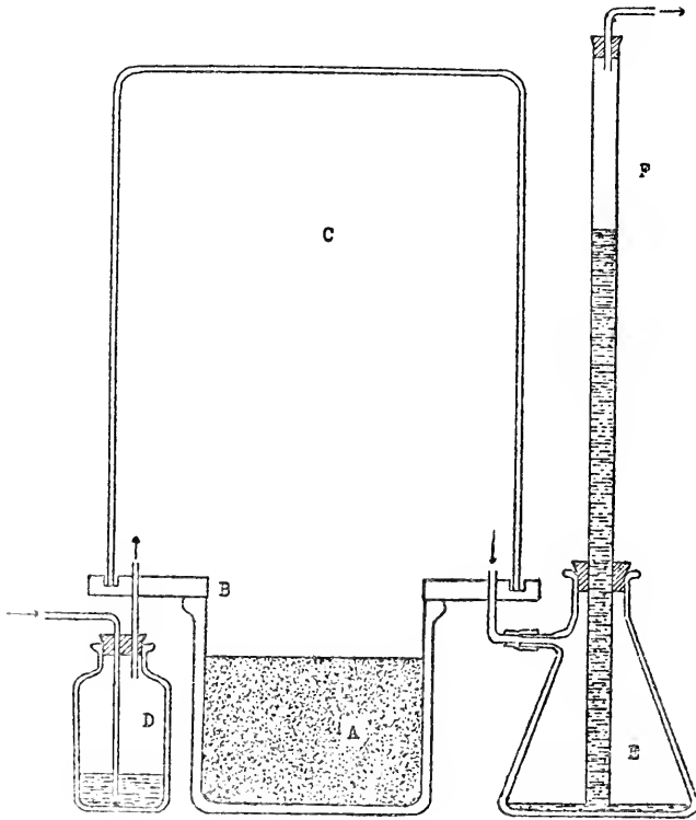
FIG. 76. Diagram representing a section through one of the units of the apparatus used in determining the carbon dioxide evolved from the soil cultures (from Neller).
