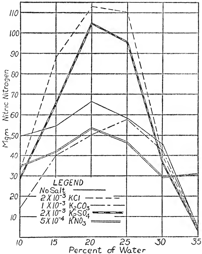
FIG. 72. Influence of moisture and potassium salts upon nitrate accumulation in the soil (from Greaves and Carter).
