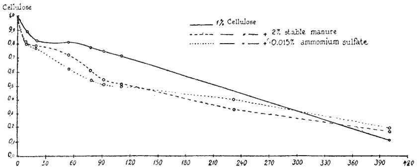
FIG. 25. Influence of nitrogen source upon the decomposition of cellulose in the soil (after Charpentier).
