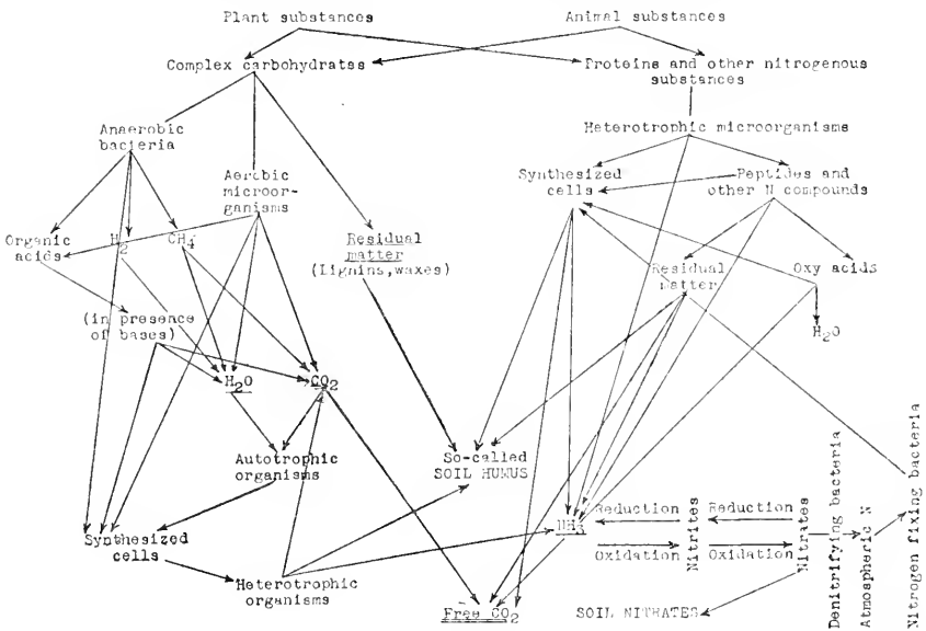
FIG. 55. Decomposition of organic matter in the soil by microorganisms (original.)
