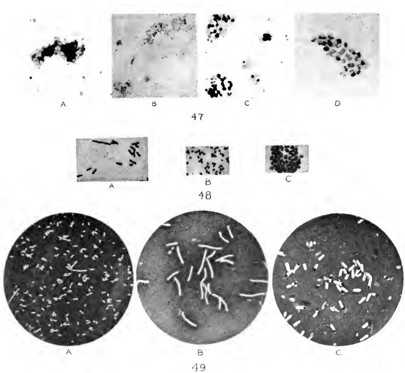
47. Life cycle of Azotobacter chroococcum : a , formation of symplasm by regenerative bodies on potato, in 9 days; b , regenerative units starting to grow, on beef gelatin, in 4 weeks; c , regenerative bodies growing from symplasm, on beef agar, in 4 weeks; d , formation of new cells by agglomeration of regenerative units on mannite soil extract, in 4 days; \times 600 (from Löhnis and Smith).
