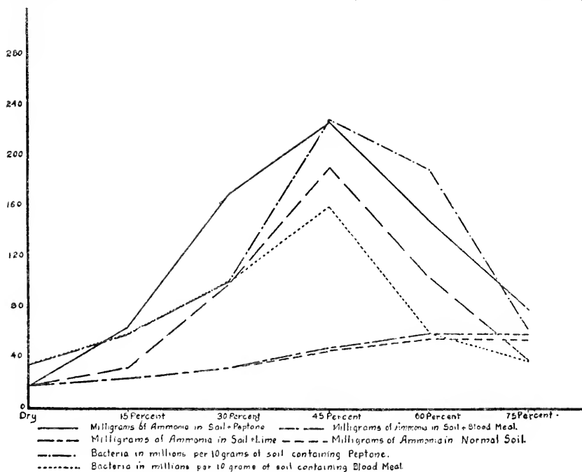
FIG. 74. Influence of moisture content of an Oregon soil upon ammonia formation and bacterial development from peptone and blood meal, 75 per cent moisture being that of full saturation (from Beckwith, Vass and Robinson).
