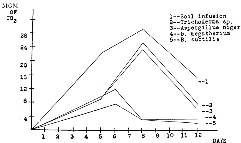
FIG. 32. Rate of decomposition of alfalfa meal by pure cultures of microorganisms and by the mixed soil flora, as indicated by the daily evolution of \text{CO}_2 (from Neller).
