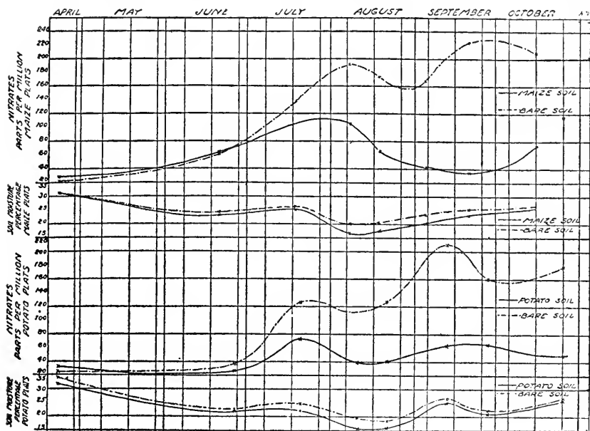
FIG. 37. Influence of crop upon nitrate content of the soil (after Lyon and Bizzell).
