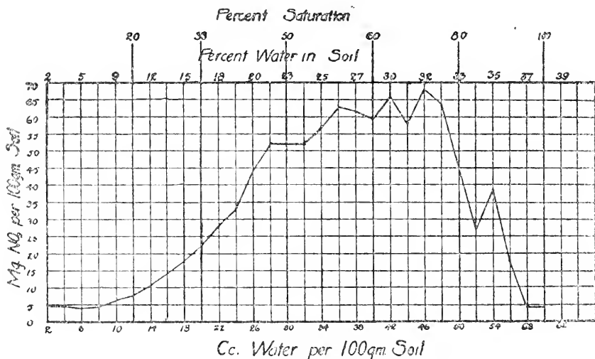
FIG. 36. Influence of moisture content upon nitrate production in the soil (from Gainey).
