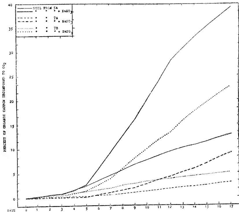
FIG. 54. Effect of nitrate upon the course of decomposition of cellulose in soils of different fertility (from Starkey).
