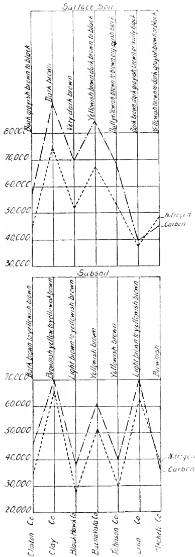
FIG. 57. Carbon and nitrogen content of Carrington silt loam (Brown and O'Neil).
