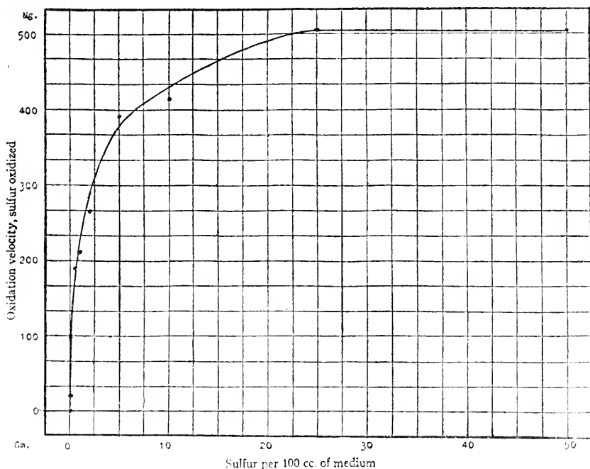
FIG. 45. Influence of sulfur content of medium upon the oxidation velocity of sulfur by Th. thiooxidans (from Waksman and Starkey).
