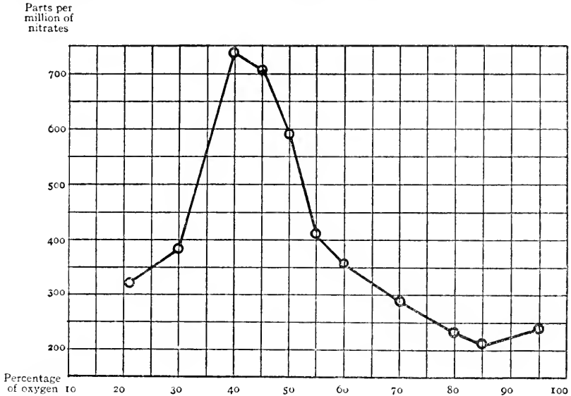
FIG. 35. Influence of oxygen tension upon nitrate formation in the soil (from Plummer).
