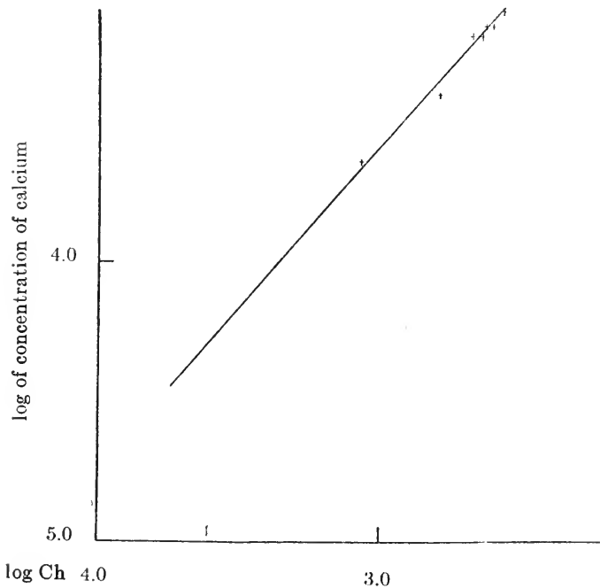
FIG. 49. Influence of B. lactis acidi upon the solubility of orthoclase (from Wright).
