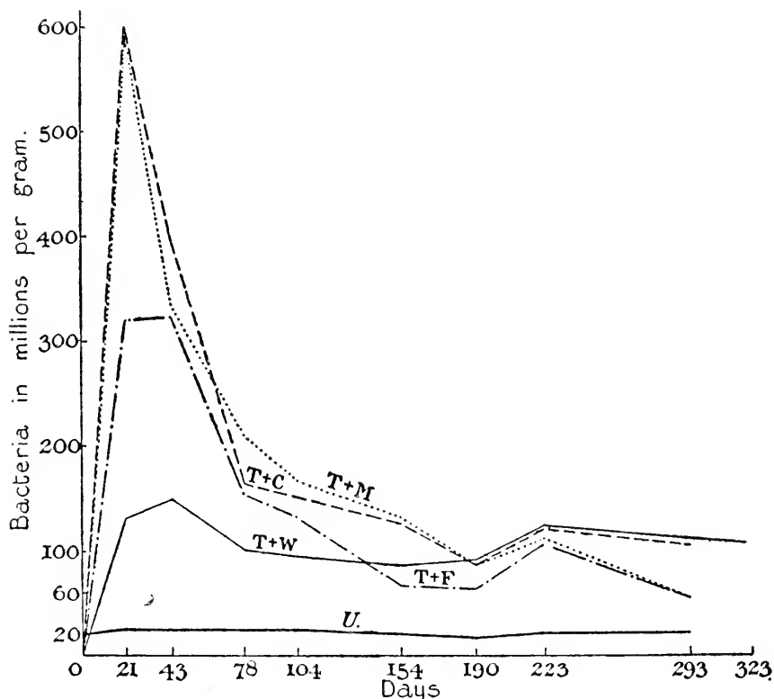
FIG. 71. Influence of protozoa upon the development of bacteria: U = uninoculated; T + W = toluene treated soil plus distilled water; T + F = toluene treated soil plus hay-infusion, filtered through a Berkefeld filter; T + C = toluene treated soil plus ciliates in hay-infusion; T + M = toluene treated soil plus mixed culture of protozoa and bacteria in hay-infusion (from Goodey).
