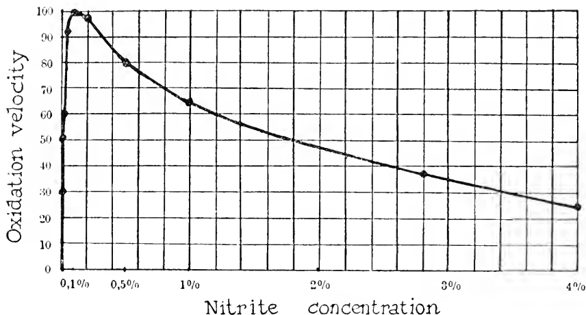
FIG. 18. Influence of nitrite concentration upon the oxidation velocity of nitrate forming bacteria (from Meyerhof).
