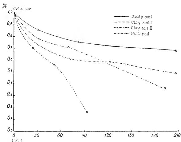
FIG. 24. Influence of soil type upon the decomposition of cellulose (after Charpentier).
