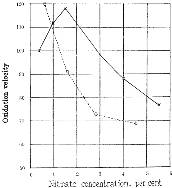
FIG. 19. Influence of nitrate concentration upon the growth (-----) and respiration (——) of nitrate forming bacteria (from Meyerhof).
