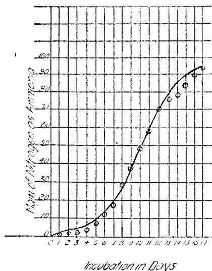
FIG. 13. Rate of ammonia formation from peptone by Asp. niger (after Waksman).
