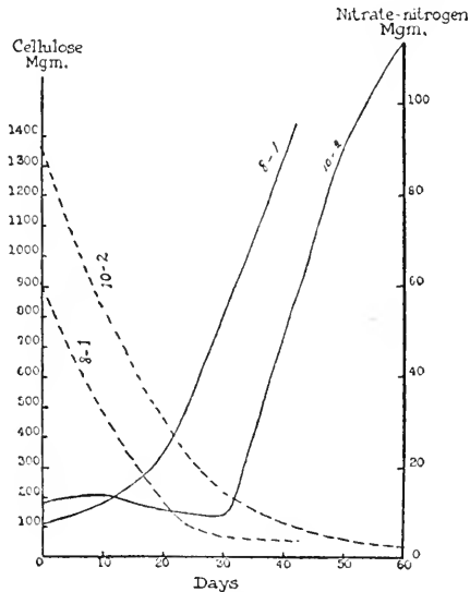
FIG. 31. Influence of cellulose on nitrate accumulation in the soil. ----- cellulose; ——— nitrate nitrogen. 8-1 and 10-2 are the experiment numbers (from Anderson).
