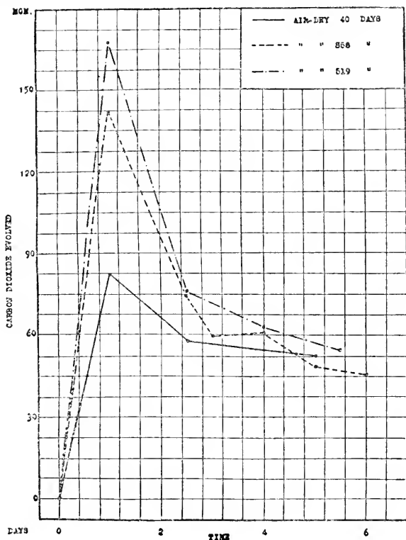
FIG. 64. Influence of length of air-drying of soil upon its biological activities, as indicated by the evolution of CO 2 (from Waksman and Starkey).
