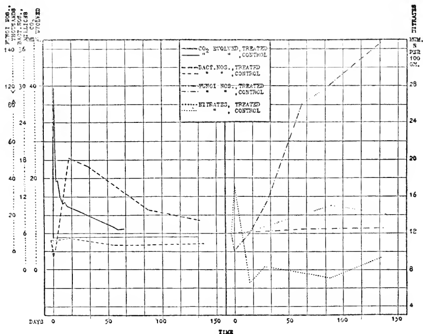
FIG. 65. Influence of heating of soil upon the numbers and activities of its population (from Waksman and Starkey).
