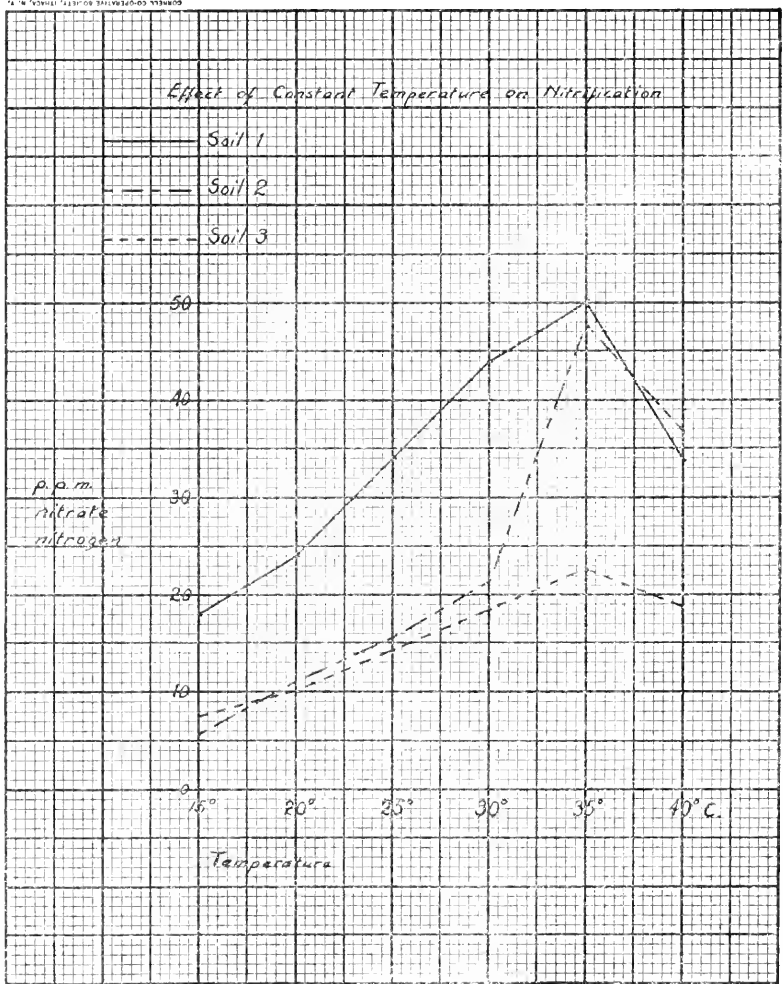
FIG. 73. Influence of temperature upon nitrification in the soil (from Pan-ganiban).
