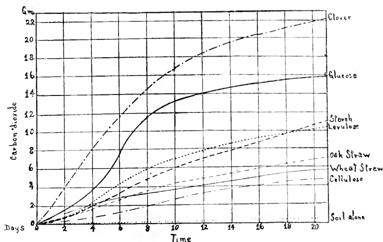
FIG. 52. Course of decomposition of different organic materials in the soil, as indicated by the evolution of carbon dioxide (after Dvorak).
