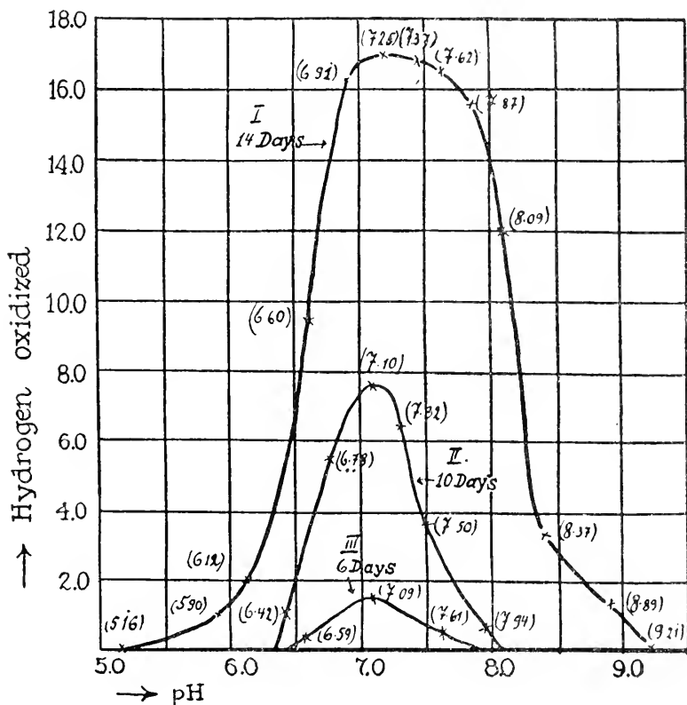
FIG. 22. Reaction of medium and oxidation of hydrogen by bacteria (Ruhland)
