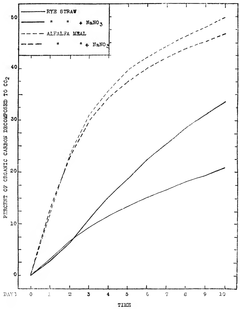
FIG. 53. Effect of nitrate upon the course of decomposition of rye straw and alfalfa meal (from Starkey).
