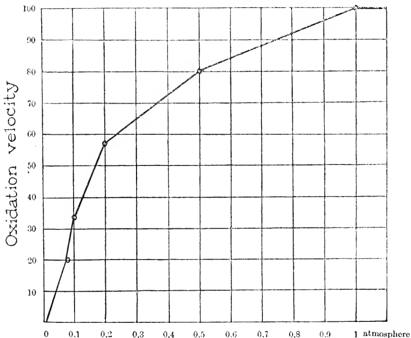
FIG. 20. Influence of oxygen pressure upon the oxidation of nitrite to nitrate (from Meyerhof).
