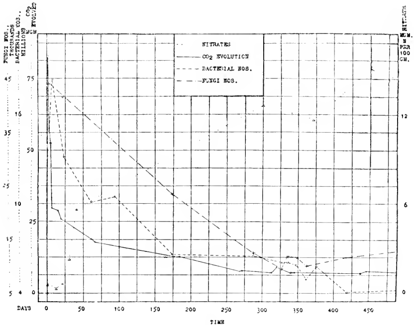
FIG. 63. Course of biological activities in undisturbed soil (from Waksman and Starkey).
