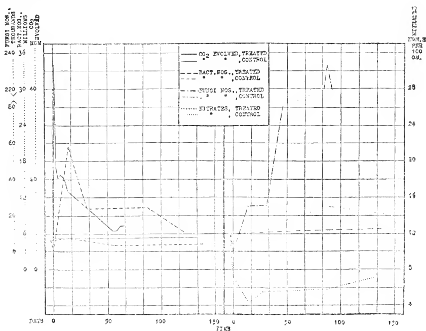
FIG. 69. Influence of CS_2 upon the numbers and activities of microorganisms in the soil (from Waksman and Starkey).
