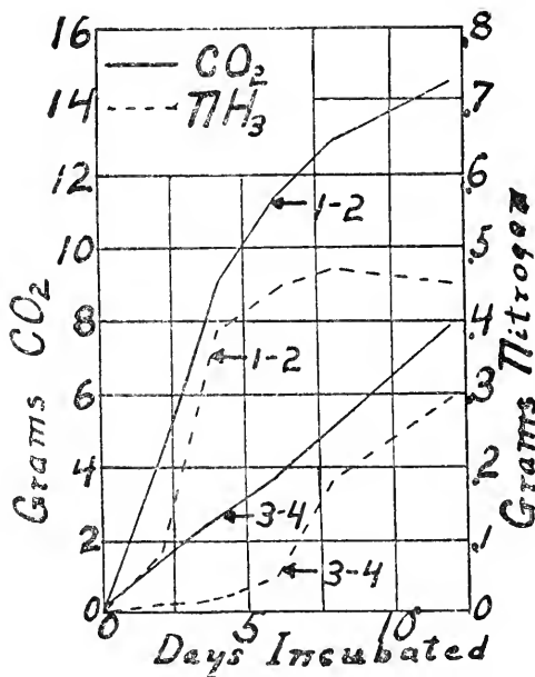
FIG. 28. Rate of decomposition of cottonseed meal in soil, as shown by the evolution of \text{CO}_2 and accumulation of \text{NH}_3 ; 1 and 2 were aerated continuously, 3 and 4 were aerated 30 minutes daily (from Gainey).
