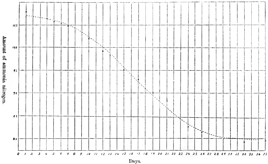
FIG. 15. Rate of oxidation of ammonia to nitrate, as shown by disappearance of ammonia in soil (after Miyake and Soma).
