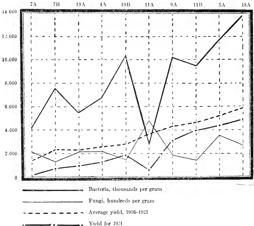
FIG. 5. Influence of soil treatment upon the numbers of bacteria and fungi in the soil: 7A and 7B, no fertilizer or manure; 4A, 19A, 19B, receiving only mineral fertilizers (phosphate and KCl); 11A and 11B, ammonium sulfate and minerals; 9A, sodium nitrate and minerals; 5A, stable manure and minerals; the B plots limed in 1908, 1913, 1918 (after Waksman and de Rossi).
