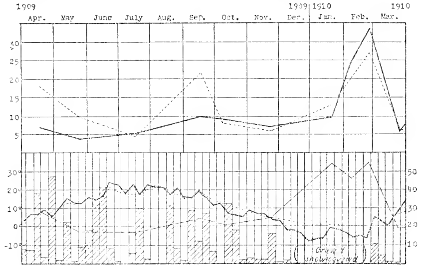
FIG. 1. Upper curves show millions of bacteria per gram of dry soil, throughout the year: ——— good soil, ----- poor soil; lower curves show: ---- soil moisture in per cent; ——— atmospheric temperature; ----- soil temperature; shaded columns represent rainfall per week, in millimeters (from Conn).
