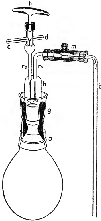
FIG. 21. Culture vessel for study of hydrogen utilization by bacteria (from Ruhland).
