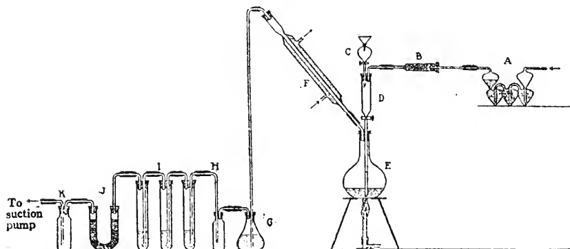
FIG. 16. Apparatus for carbon determination in solution cultures (after Waksman and Starkey).
