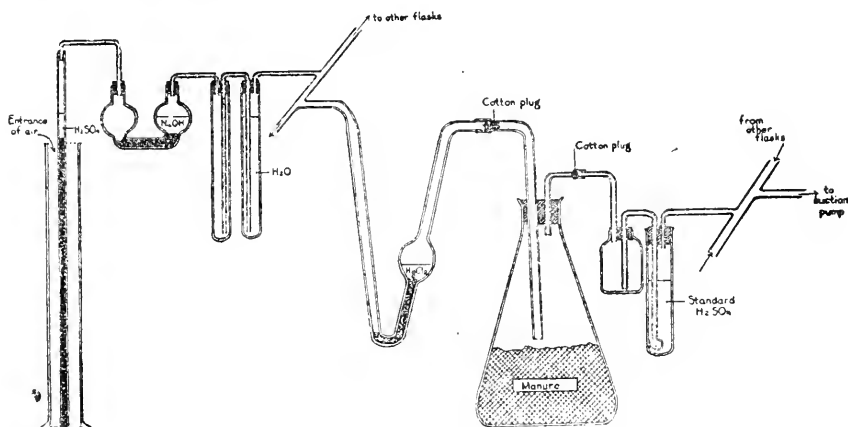
FIG. 29. Apparatus for study of ammonia formation in the decomposition of manure (from Conn and Collison).
