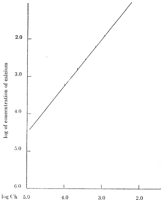
FIG. 48. Influence of sulfuric acid upon the solubility of calcium silicate (from Wright).
