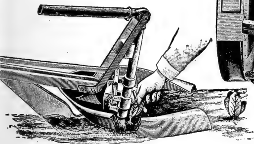
Fig. 43. Transplanting machines.
