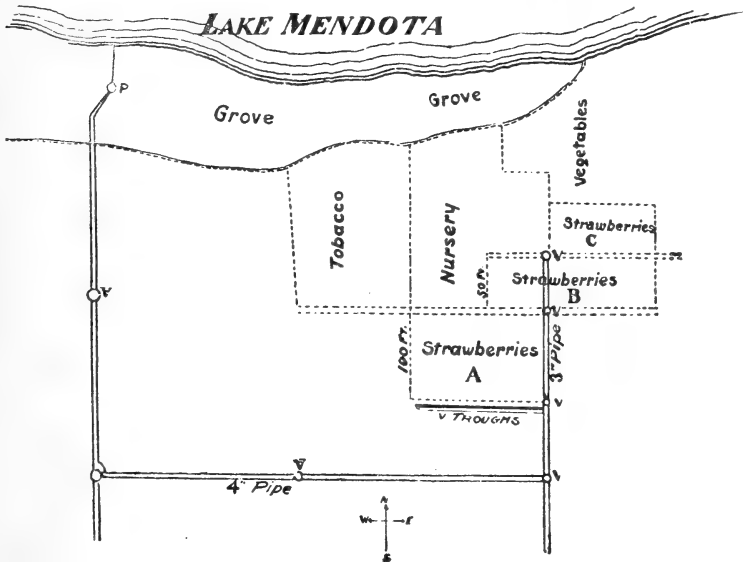
Fig. 39. Method of distributing water.
