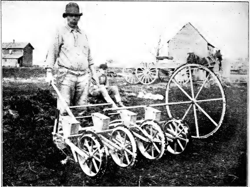
Fig. 95. A four-row onion seeder.
