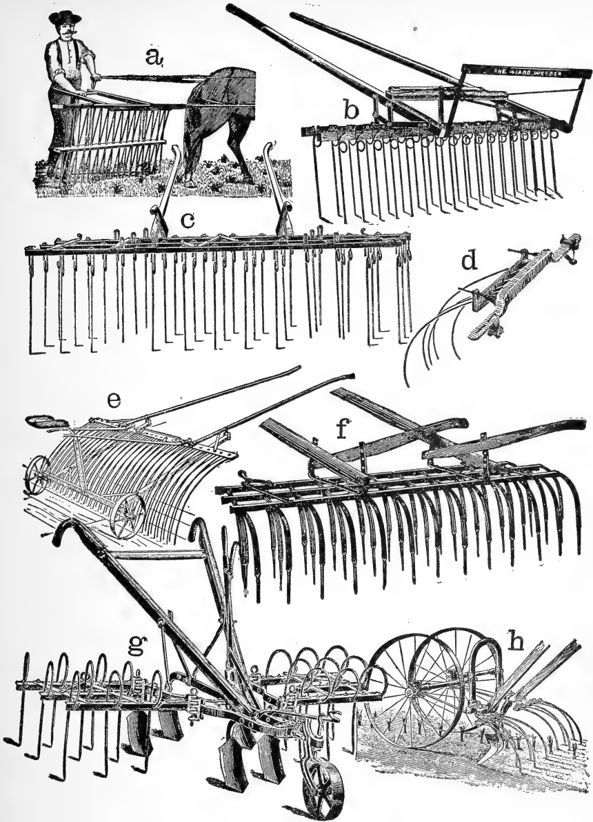
Fig. 30. Horse weeders.
