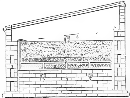
Fig. 17. Pipe-heated hotbed.
