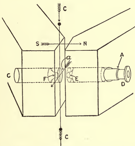
Fig. 16.—Lewis's diagram of the string galvanometer: A , Microscope for observing the movements of the string of silvered quartz ( C ) suspended in the field of the electromagnets ( S N ); \alpha , direction of current's movements, at right angles to the magnetic field; C F , electric light and condenser.
