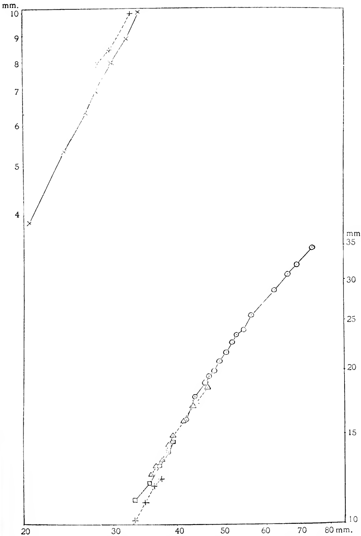
FIG. 92.—Graph to show relative growth of the mandible in the different male forms of the stag-beetle, Cyclommatus tarandus .
