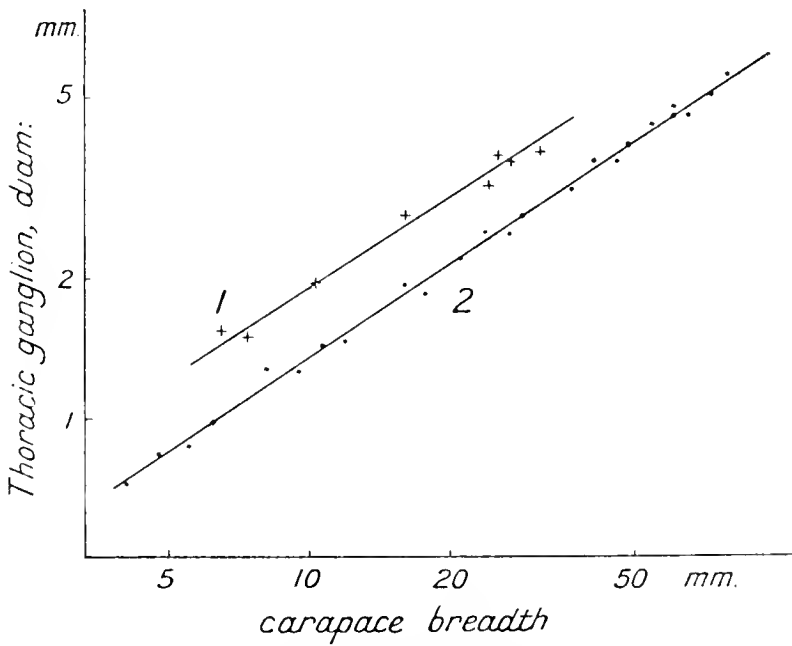
FIG. 15.—Diameter of the thoracic ganglion against carapace breadth in crabs : (1) Pachygrapsus ; (2) Carcinus ; logarithmic plotting.
