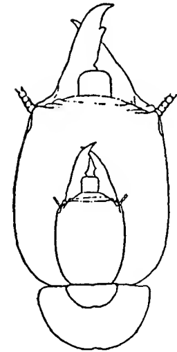
FIG. 38.—Heads of largest and smallest workers in a colony of the termite Termitopsis angusticollis , showing heterogony and change of proportions with increase of absolute size.
