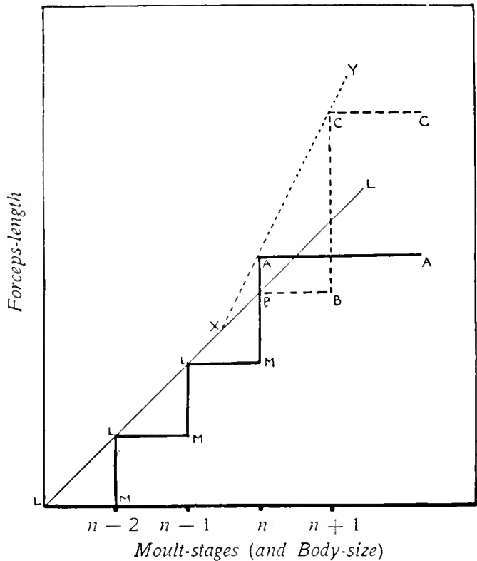
FIG. 41.—Diagram to show the possible origin of dimorphism of the male forceps in earwigs, Forficula .
