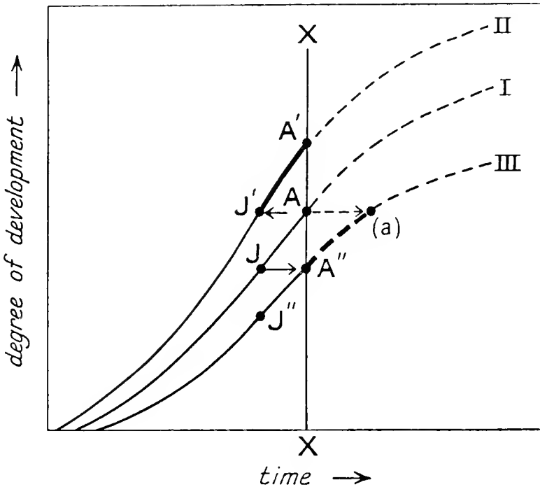
FIG. 104.—Diagram to illustrate positive and negative mutations in rate-factors, leading to recapitulation and pedomorphosis respectively.
