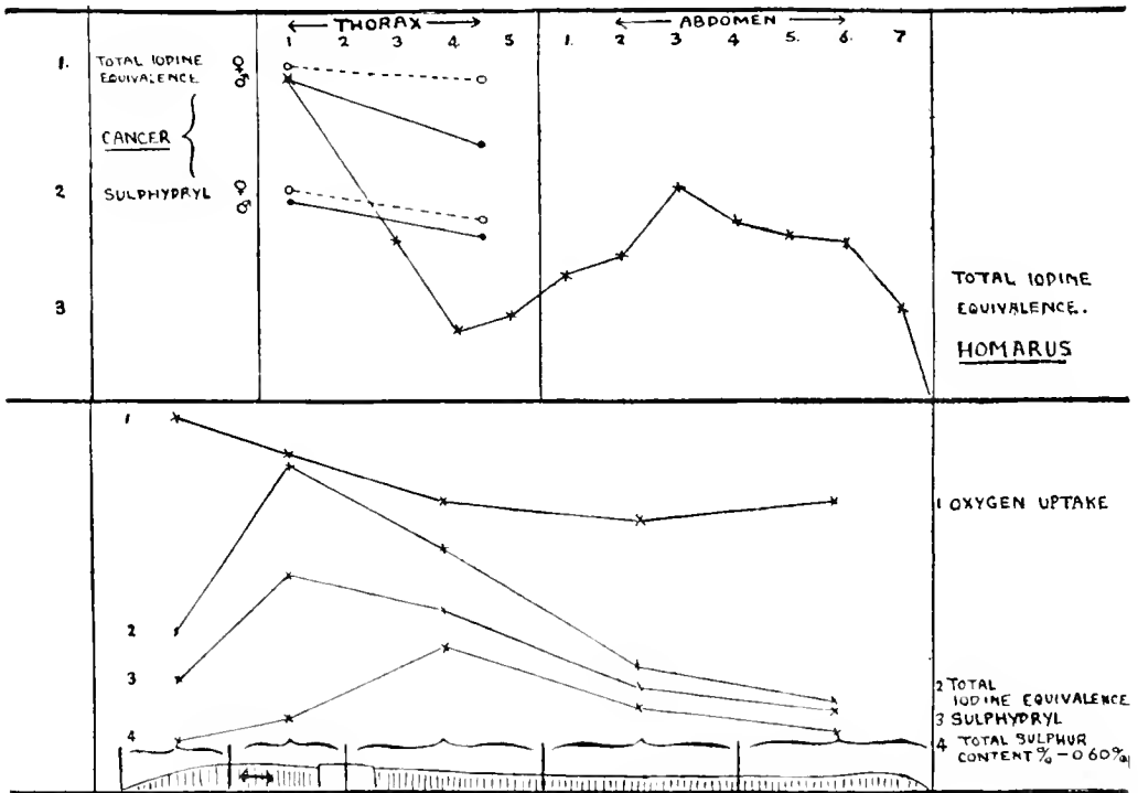
FIG. 79.—Gradients in content of various sulphur compounds and in oxygen uptake in the Crustacea, Cancer and Homarus (above), and the earthworm (below).
