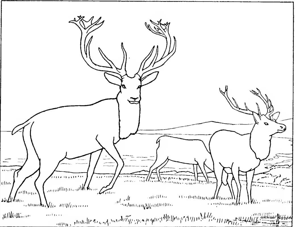
FIG. 90.—Differences in absolute body-size and relative antler-size of pre-historic (left) and modern (right) Scottish Red Deer.
