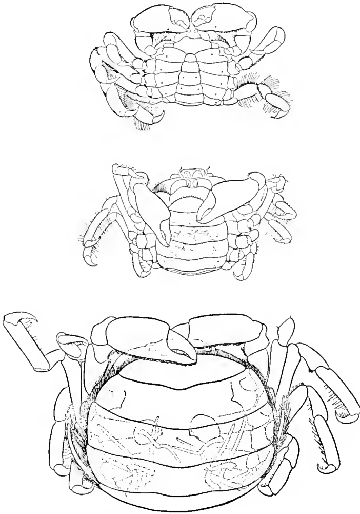
FIG. 53.—Changes of shape in the female abdomen of the pea-crab, Pinnotheres , during growth.
