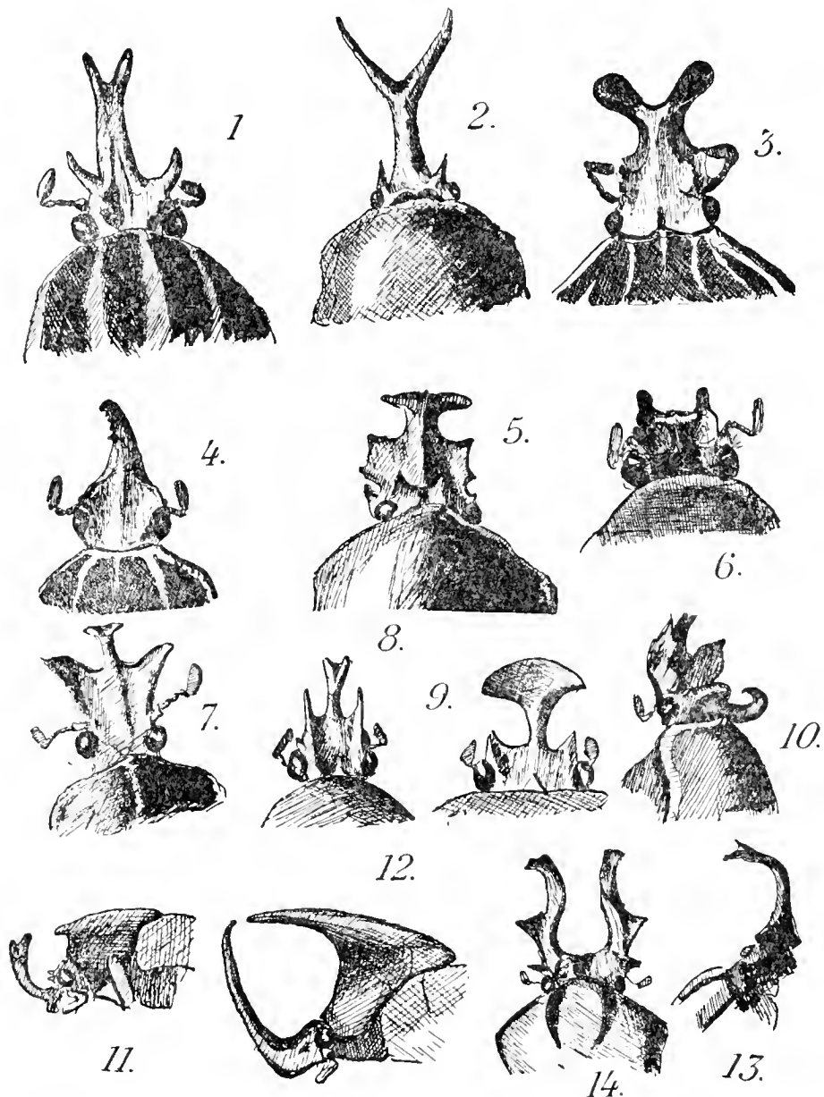
FIG. 95.—Specific variations in detail of heterogonic organ (cephalic horn) in different species of Goliath beetles (Goliathidae).
