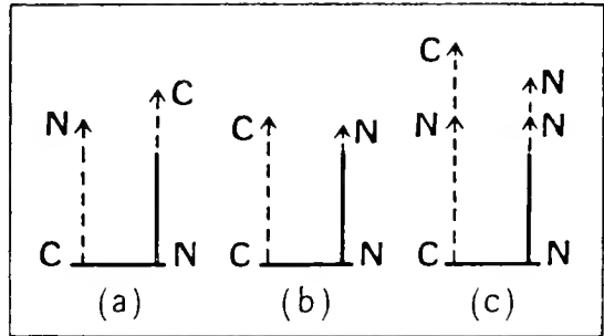
FIG. 84.—Diagram to illustrate Przibram's hypothesis as to reversal of chelae in heterochelous Crustacea.
