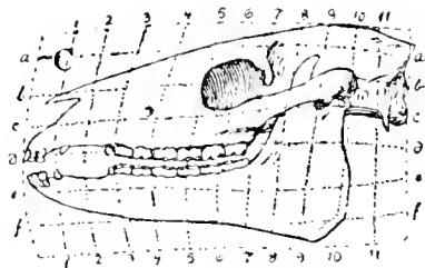
FIG. 60.—Comparison of hypothetical forms of the skull in the ancestry of the horse (C—E), constructed by applying the method of Cartesian transformation (A—H) with actual forms; (M) Mesohippus; (Mi) Miohippus; (Pa) Parahippus; (P) Protohippus.
