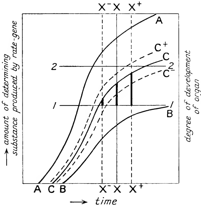
FIG. 102.—Hypothetical curves to illustrate the relation of rate-genes to vestigial organs.
