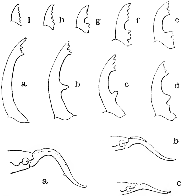
FIG. 93.—To illustrate change of form of mandible with increase of its absolute size in male stag-beetles.
