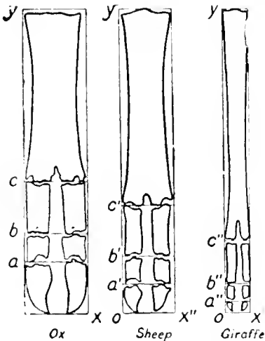
FIG. 48.—Comparison of the skeleton of the foot in Ox, Sheep and Giraffe, to show graded alteration in proportions of parts.
