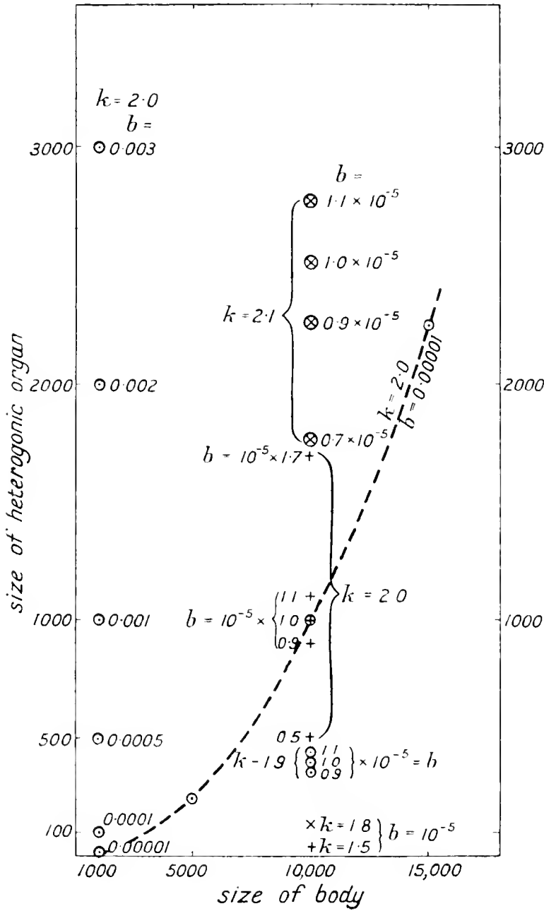
FIG. 1.—Diagram to show the quantitative effect of varying the constants in the simple heterogony formula, y = bx^k , assuming that the origin of growth in x and y begins at the same time.
