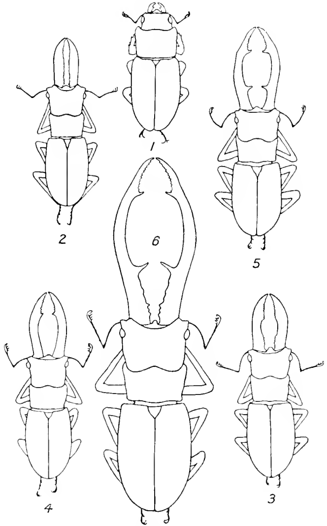
FIG. 91.—(1) Female and (2—6) five different-sized males of the stag-beetle, Cyclommatus tarandus , to scale, to show the change in form and relative size of the male mandible with increase of absolute body-size.
