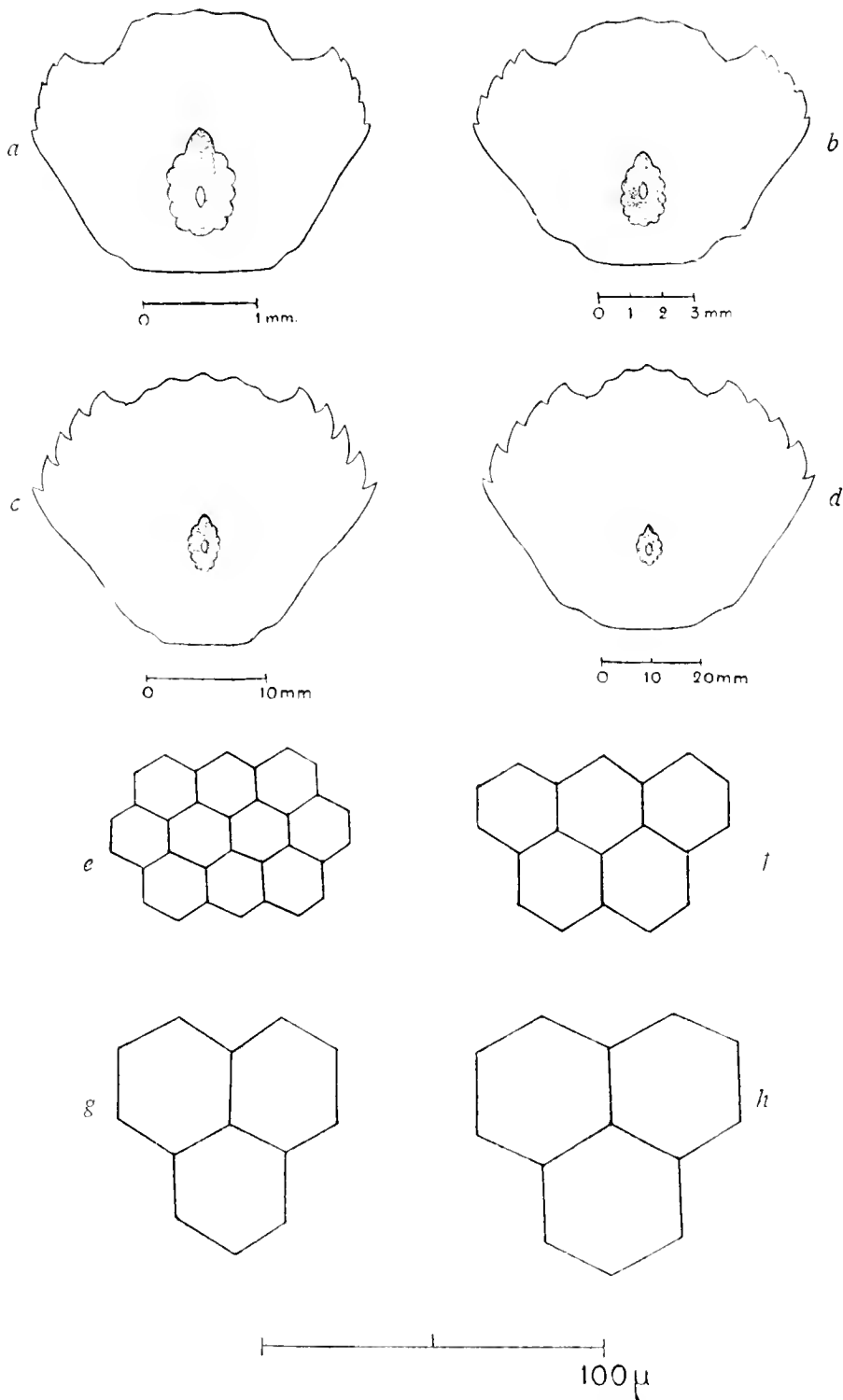
FIG. 14.—Change of proportions in the crab, Carcinus maenas .
