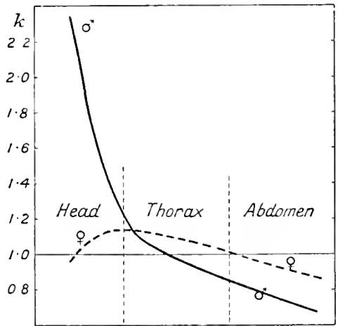
FIG. 63.—Probable growth-gradients in the body of male and female stag-beetles ( Lucanus cervus ).
