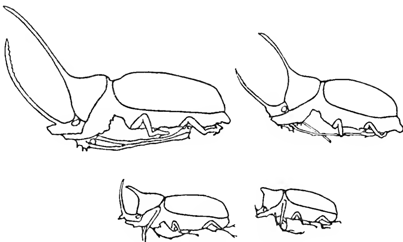
FIG. 94.—Phenomenon of Lameere and Geoffrey Smith in species of the Dynastid beetle Golofa .
