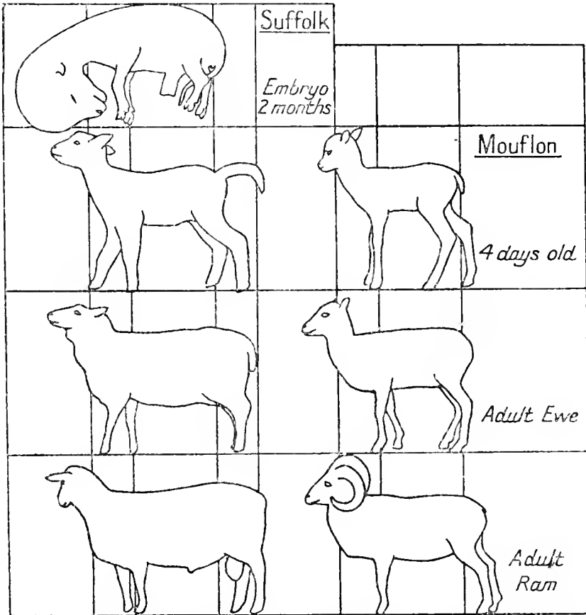
FIG. 96.—Changes in proportions during growth in wild sheep and improved breeds of domestic sheep (see text).
