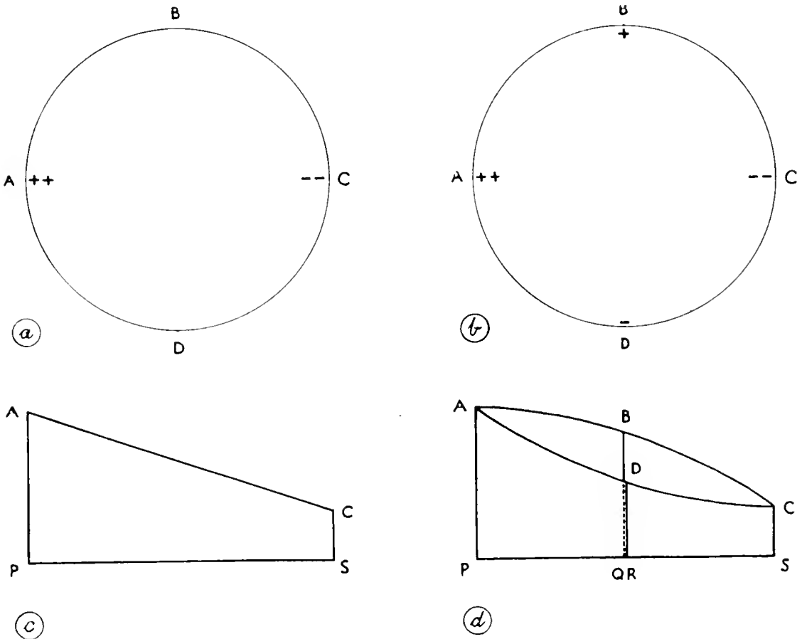
FIG. 76.—Diagram to illustrate the growth-gradients operating to produce the plane and the turbate spiral shells of Molluscs.
