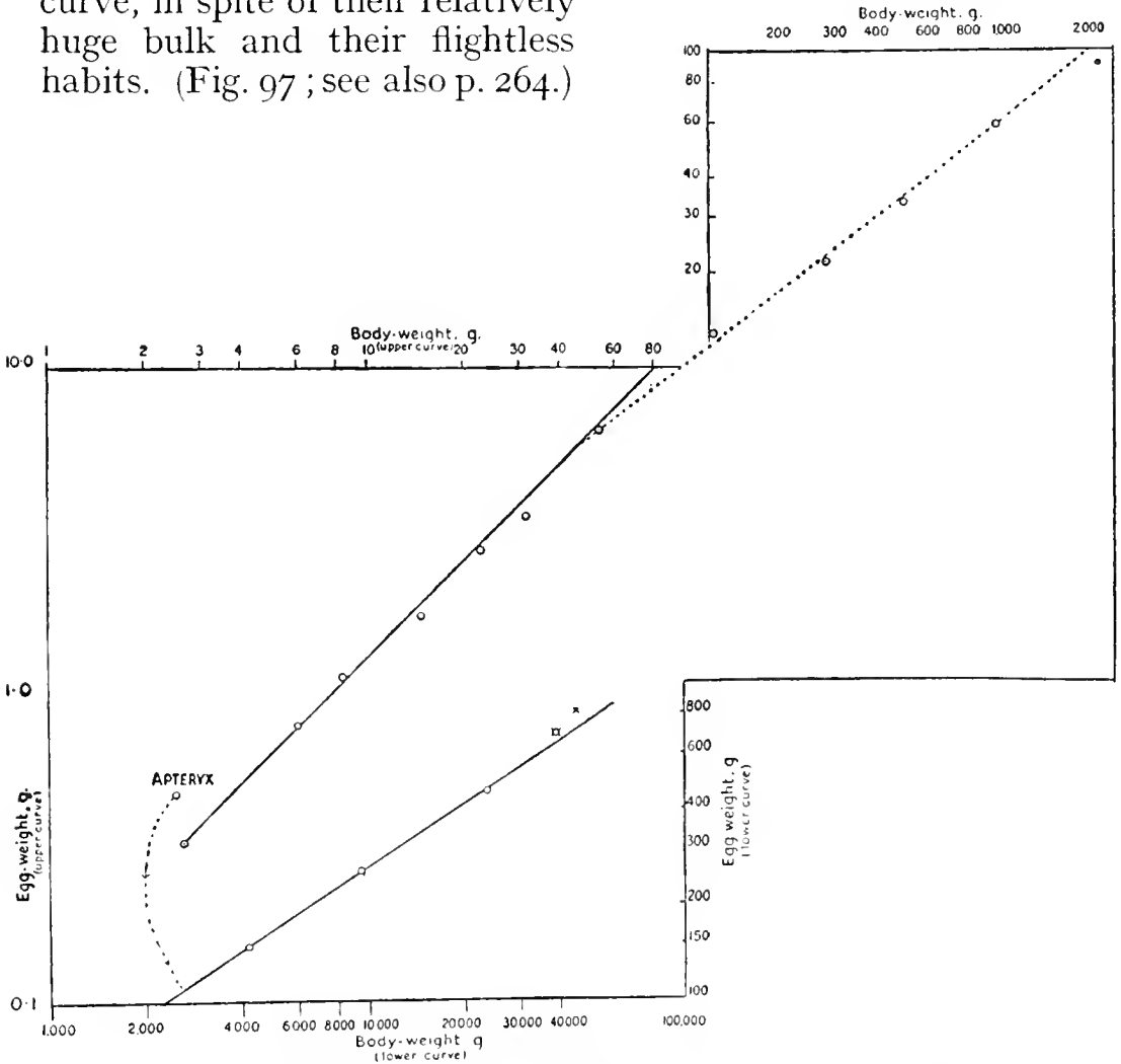
FIG. 97.—Graph showing change of egg-weight with body-weight in 432 species of birds: Means by weight-classes, logarithmic plotting.
