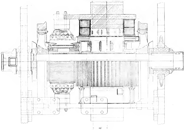
FIG. 2. BI-POLAR GEARLESS MOTOR.
