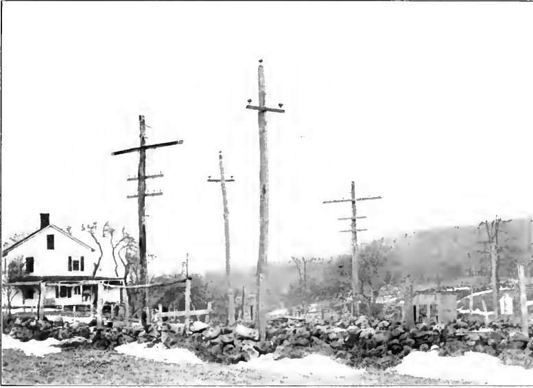
FIG. 1.—WIRE GRIDIRON UNDER 33 000-VOLT TRANSMISSION LINE.
