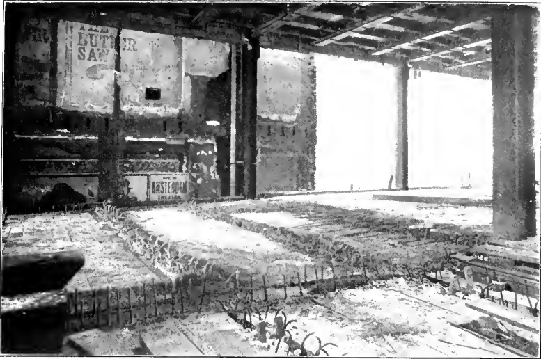
FIG. 1. THE BONWIT-TELER BUILDING.
