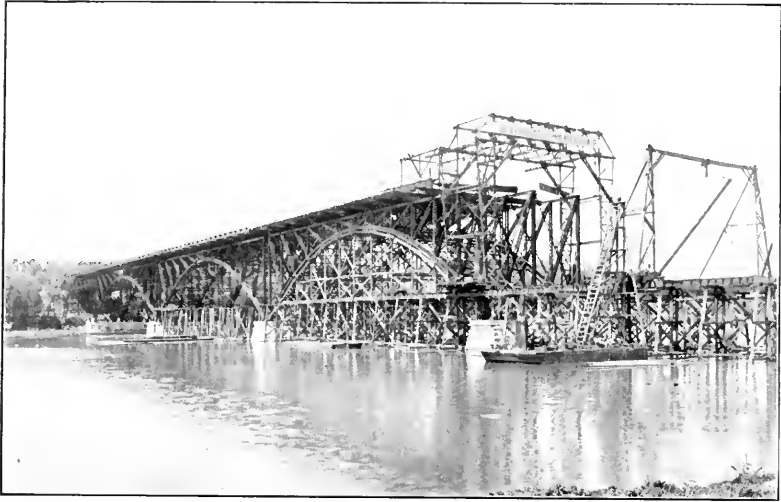
FIG. 1.—THE ERECTION OF THE FAIRMOUNT PARK BRIDGE, OVER THE SCHUWKILL RIVER, IN PHILADELPHIA.
