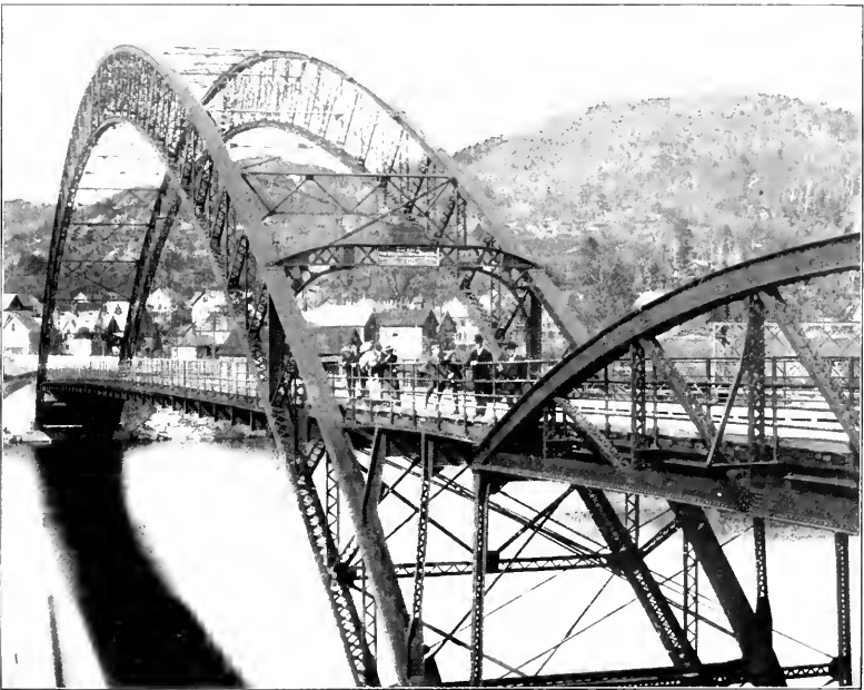
FIG. 2.—END VIEW, BELLEWS FALLS ARCH BRIDGE.
