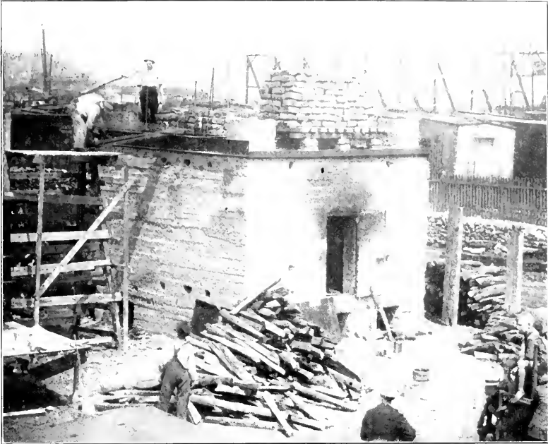
FIG. 1. CINDER CONCRETE TEST HOUSE, AFTER FOURTH FIRE
