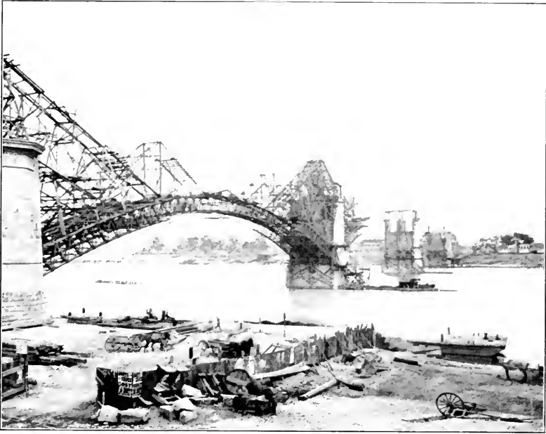
FIG. 1.—ERECTION OF THE EADS BRIDGE.
