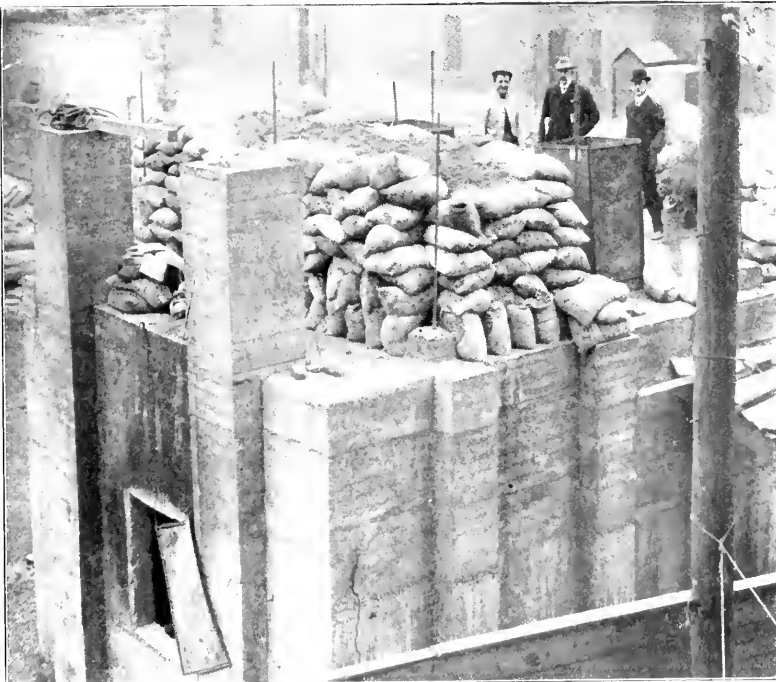
FIG. 2. STONE CONCRETE HOUSE, WITH TEST LOAD, AFTER FOUR-HOUR FIRE TEST.
