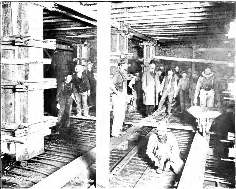
FIG. 2.—CONCRETING ON SECOND FLOOR, MANUFACTURERS' FURNITURE EXCHANGE BUILDING.
