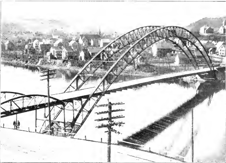
FIG. 1.—THE BELLEWS FALLS ARCH BRIDGE.
