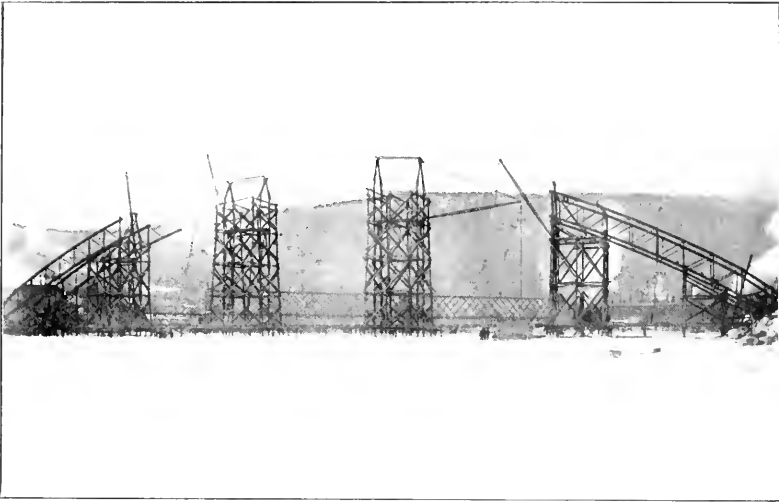
FIG. 1.- BELLOWS FALLS ARCH BRIDGE IN PROGRESS.
