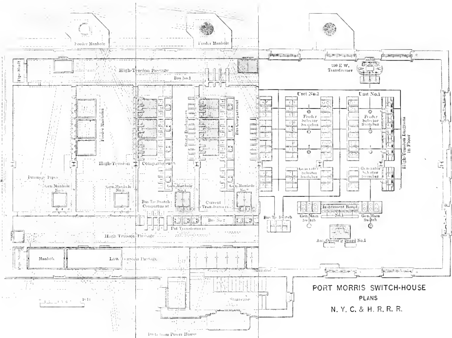
PLAN OVER BASEMENT
