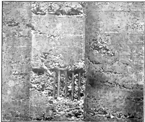
FIG. 3.—CAVITIES IN COLUMN.
