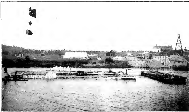
FIG. 2. BUILDING COFFER-DAM OF PIER 3. SHOWING CABLEWAY.
