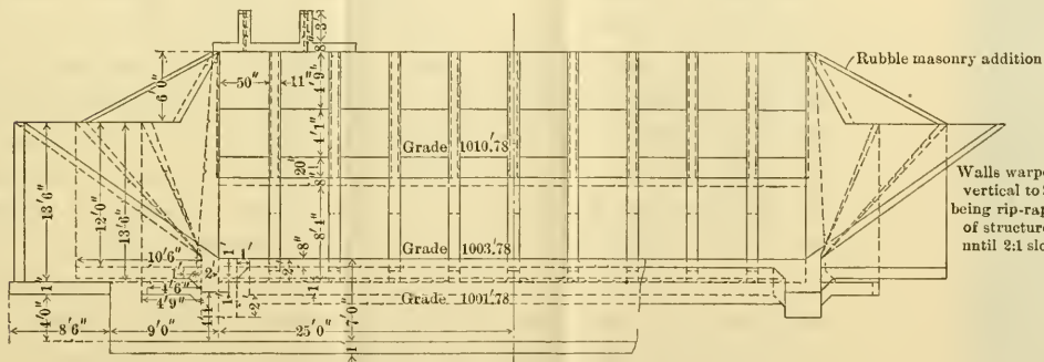
ELEVATION OF DOWN-STREAM END
