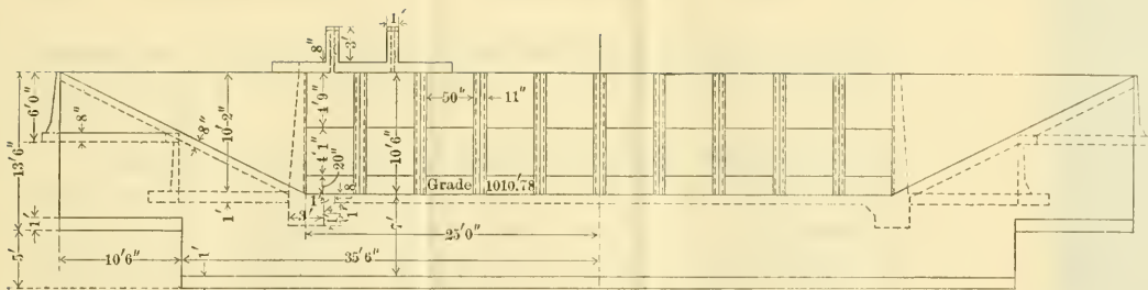
ELEVATION OF UP-STREAM END
