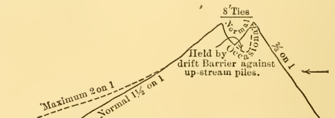
RESULTING SECTION OF ROCK FILL DAMS MADE DURING FIRST AND SECOND CLOSINGS
