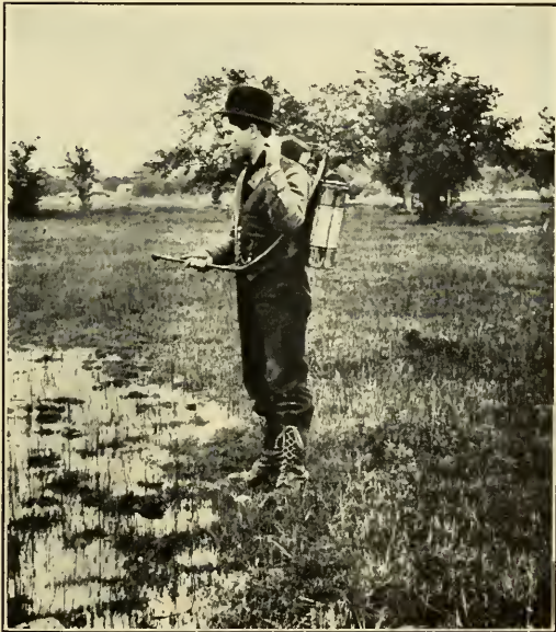
FIG. 2.—KNAPSACK SPRAY-PUMP IN USE, SPRAYING OIL ON A TYPICAL ANOPHELE BREEDING PLACE.
