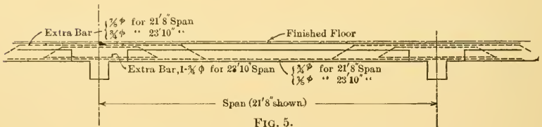
FIG. 5. TYPICAL DETAIL OF FLOOR JOIST
