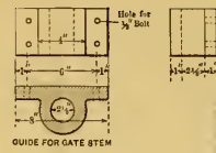
GUIDE FOR GATE STEM
