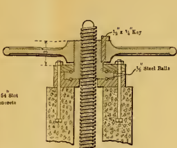
STANDARD SQUARE THREADS ON STEMS 2 AND 1/2" DIAM., PITCH 1/2" AND 4" RESP.
