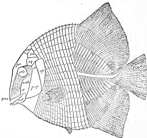
Mesodon macropterus (Agassiz); left side view of fish, about one-half natural size.—Lithographic Stone; Bavaria. fr. , frontal; m.cth. , mesethmoid; md. , mandible; op. , operculum; orb. , orbit; p.op. , preoperculum; pa. , parietal; pma. , premaxilla; s.occ. , supraoccipital; sq. , squamosal; v. vomer.
