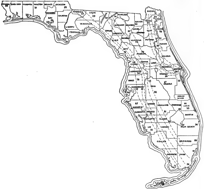
FIG. 2. Temperatures (F.) morning of December 13, 1934. Dotted lines show air flow as indicated by damage to vegetation.
