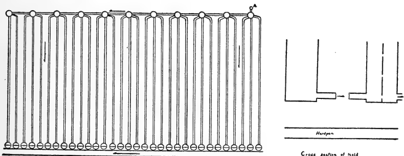
Fig. 1 Irrigation system for a five-acre tract of land
