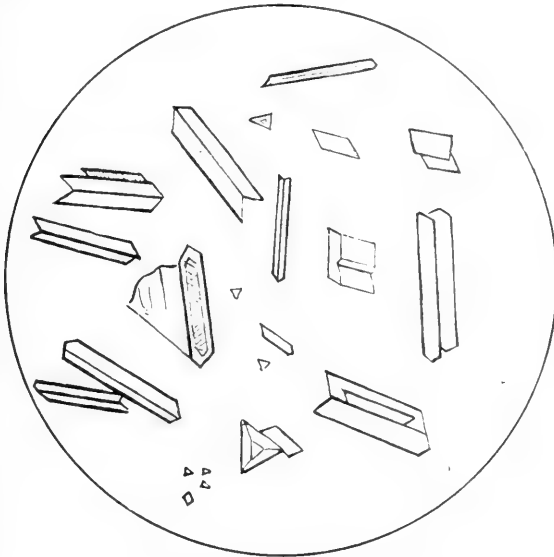
Fig. 2. Crystal and twin forms of selenite, \times 45 .
