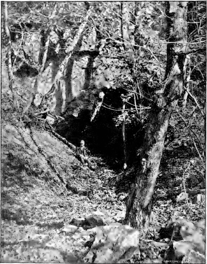
FIG. 1. Entrance to Hartman's Cave.
