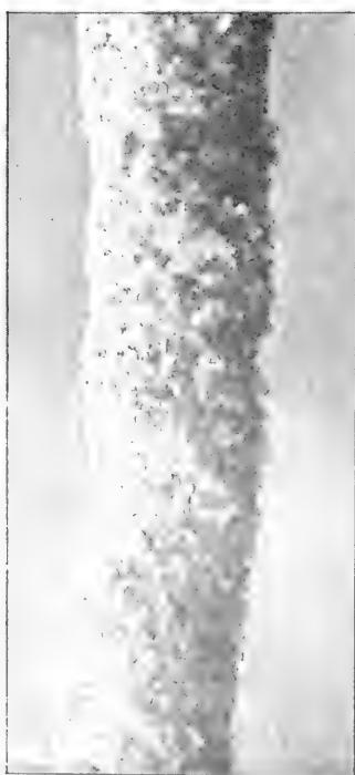
Fig. 1. Volcanic stalactite covered with selenite, x 4.
