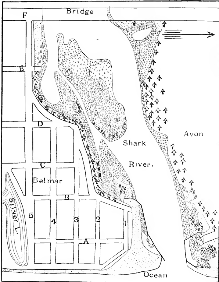
Fig. 5.—Salt Marshes along Shark River. X, Spartina stricta maritima ; V, Spartina patens ; Z, Scirpus pungens ; O, Distichlis spicata ; θ, Baccharis halimifolia ; J, Juncus Gerardi ; *, Phragmites communis ; ≡, Salicornia herbacea ; II, Gerardia purpurea ; dotted areas = sand with typic dune plants; ↑, tree thickets.
