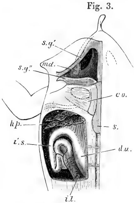
Fig. 3. A portion of the right half of fig. 2, dissected to show the intestine and liver, together with the mode of attachment of the gular sac.
