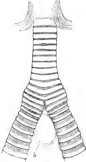
Syrinx of Balæniceps rex . Front view. b , free margin of bronchidesmus.
