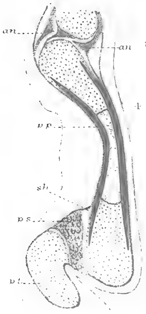
Supernumerary phalanx & syndesmoses in Amphibia.
