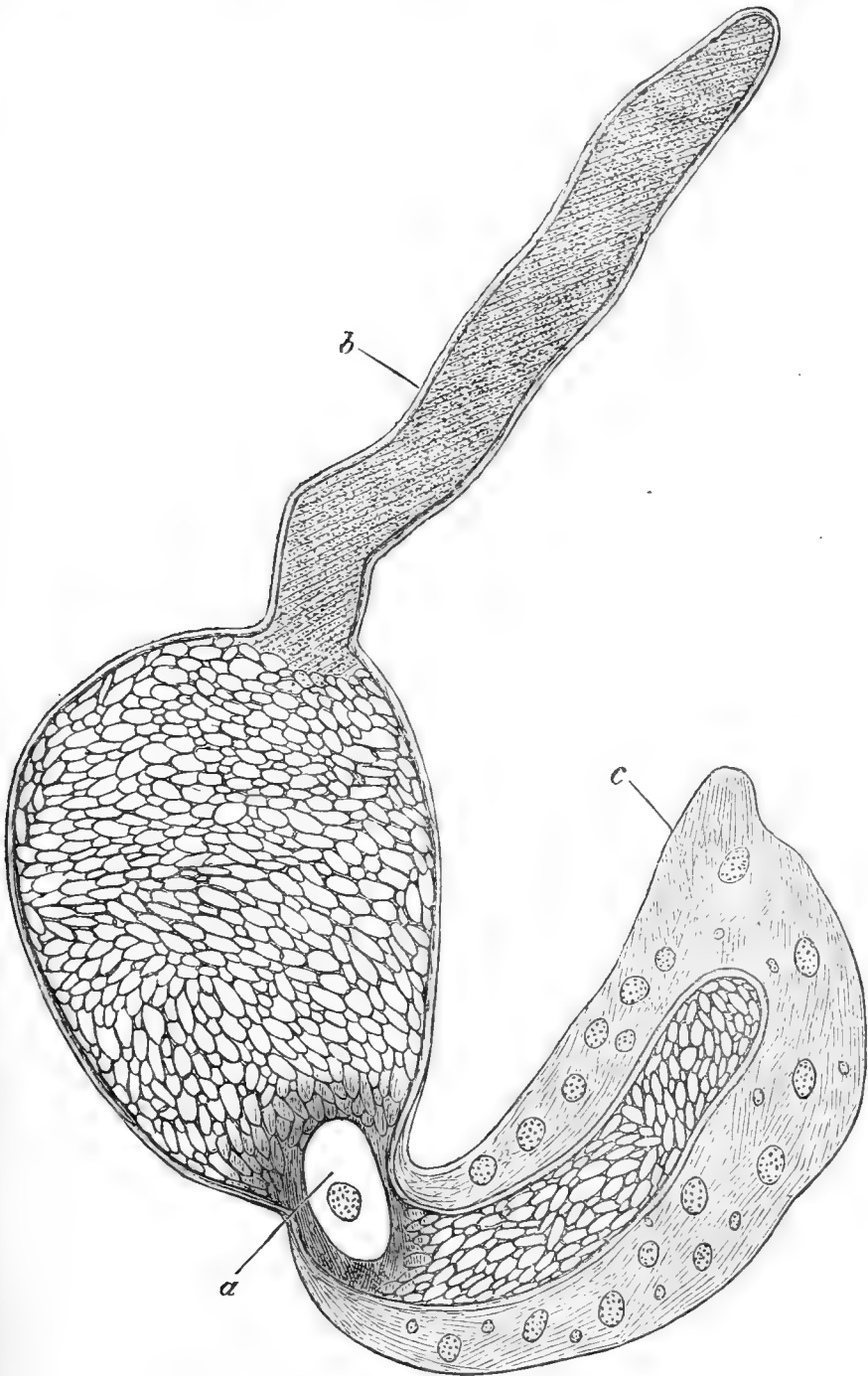
Gregarine from body-cavity of Pericheta novæ-zelandiæ .
