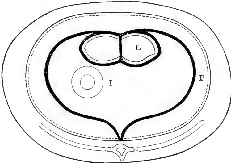
Diagrammatic section through body of a Crocodile .
