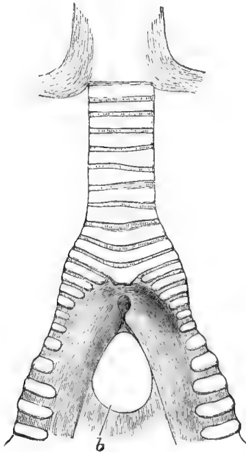
Syrinx of Balæniceps rex . Posterior surface. b , as in fig. 1.
