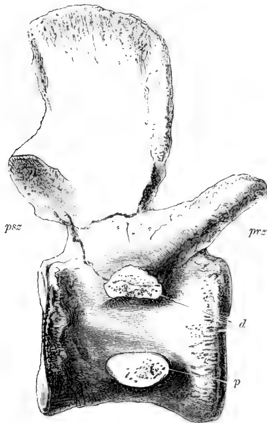
Cervical vertebræ of Stenocaurus .
