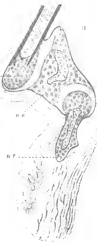
Supernumerary phalanx & syndesmoses in Amphibia.
