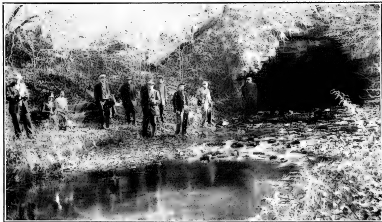
Fig. 27. Upper Dalton cave, part of Shawnee cave (Fig. 11) east of Mitchell, Ind. The location of cross caves and a sink at this point caused a collapse which brings the stream to the surface for several rods when it again continues in its subterranean channel.
