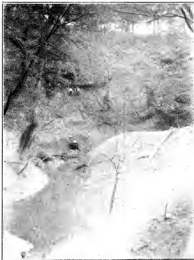
Fig. 23. A "Gulf" of Lost river above its outlet at Orangeville. The water rises to the surface at the right of the middleground of the picture and flows to the right and left, forming two streams, for a very short distance which sink and finally rejoin the subterranean channel. The little pond on the left side of the group in the middle background is a large cave, one of the abandoned subterranean channels of the river. The second, or present channel is considerably below the water shown in the foreground. Here a large area has collapsed blocking the lower channel and forcing the water to the surface, when it again finds new channels around or through the obstruction to its main channel again in which it continues.
