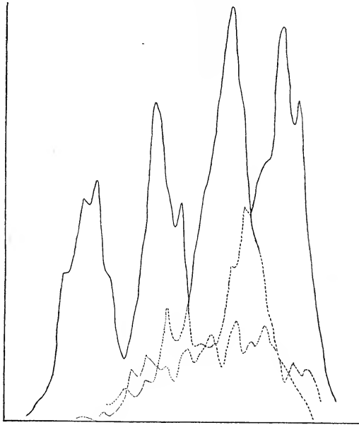
Text-fig. 9.—Composite curve based on measurements from different localities, and showing the possible occurrence of age groups in the flathead. The maxima are at 24, 32, 42 and 54 cm. respectively.
