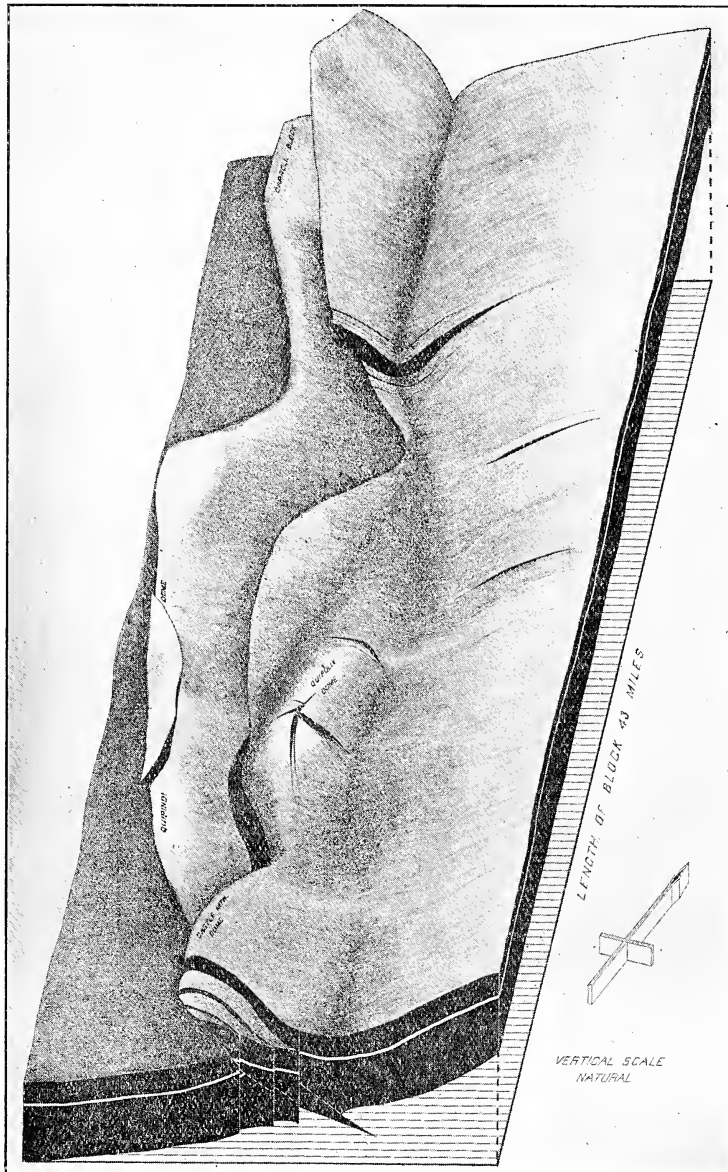
Text-fig. 1.—Reconstruction of the folding and faulting of the Werrie Basin. The folded strata in the diagram are the Kuttung sediments, all superficial rocks having been removed and the eroded portions restored. The white band is the porphyry boulder horizon.
