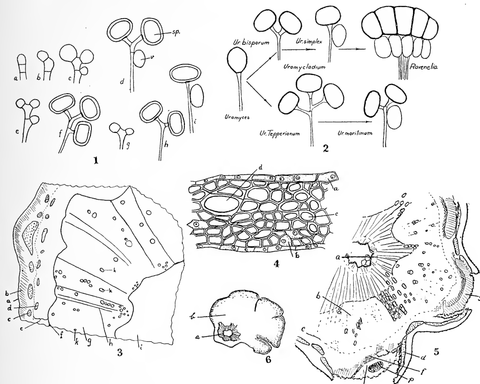
Fig. 1.—a-d, segmentation of the teleutospores of Uromycladium maritimum ; e-f, Ur. Teppermanum ; g-h, Ur. bisporum ; g and i, Ur. simplex ; sp, spore; v, vesicle. All diagrammatic.
