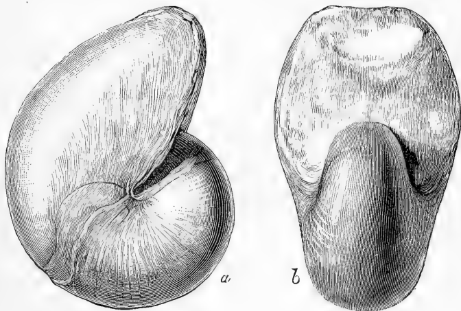
FIG. II.— Nautilus Bradfordensis , n. sp. a , lateral view of an example of the more inflated form, showing the 'black-layer' immediately in front of the aperture, and the fine line indicating the course of the anterior boundary of the muscular scar and of the annulus; a portion of the test on the body-chamber is represented as having been broken away, in order to depict this line, which really exists on the opposite side of the fossil. b , front view of the same. Inferior Oolite ( concauzone ): Bradford Abbas, Dorset. Drawn from a specimen in the British Museum Collection [C. 3177]. About five-sixths natural size.
