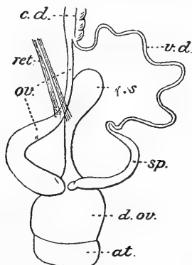
Portion of the reproductive organs of Ariunculus Austriacus , n.sp.
