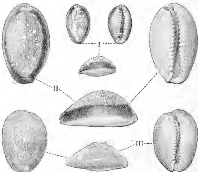
FIG. I. Cypraea caput-anguis , Phil. ,, II. C. caput-serpentis , Linn., variety usually mistaken for the preceding. ,, III. C. caput-serpentis , var. caput-colubri , n.
