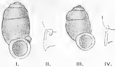
I, II. Rhabaulus Perakensis , n.sp. III, IV. ——— Lorraini , Pfr.
