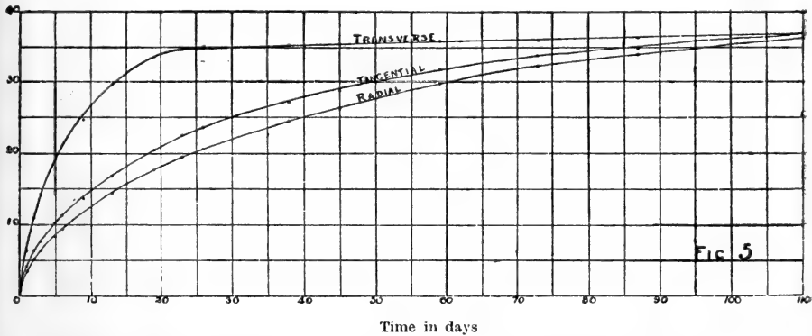
FIG. 5 CURVES OF LOSS OF MOISTURE FROM THE TRANSVERSE TANGENTIAL AND RADIAL FACES OF CUBES OF WOOD.
