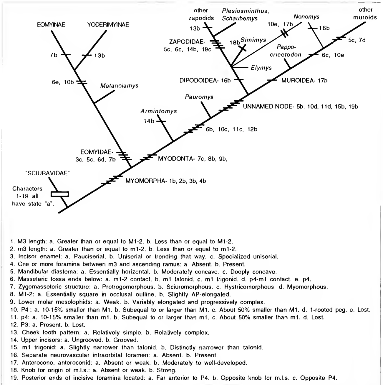
Figure 10. Cladogram showing hypothesized relationships of various Paleogene myomorph rodents. Geomyoidea and Dipodidae omitted for simplicity. See text for discussion.
