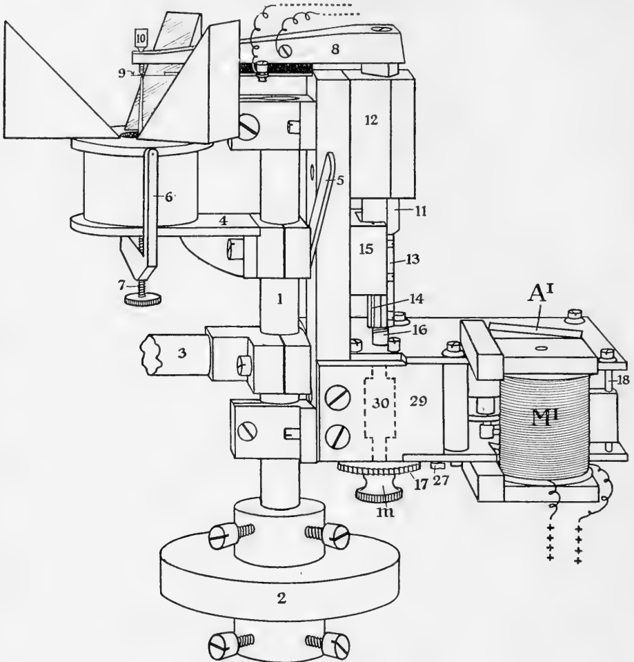
Fig. 1. The auxanometer.
