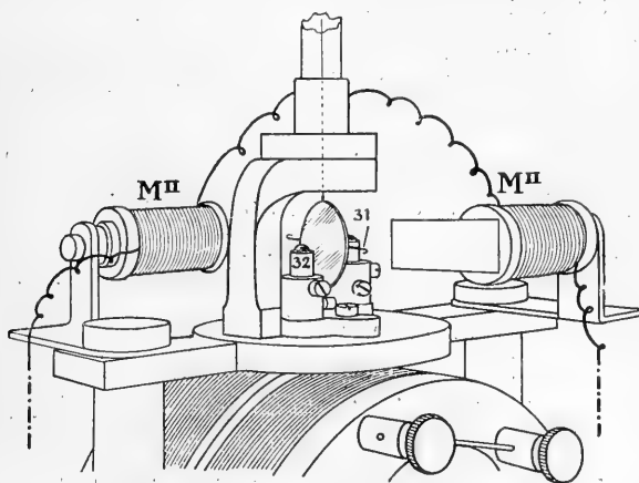
Fig. 3. The galvanometer, transformed into a relais.
