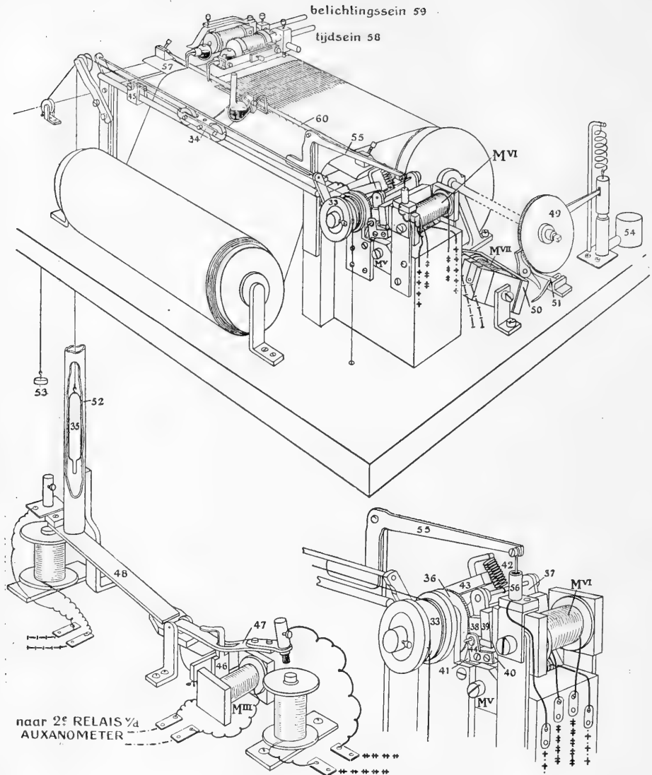
Fig. 5. The Recording Apparatus.
