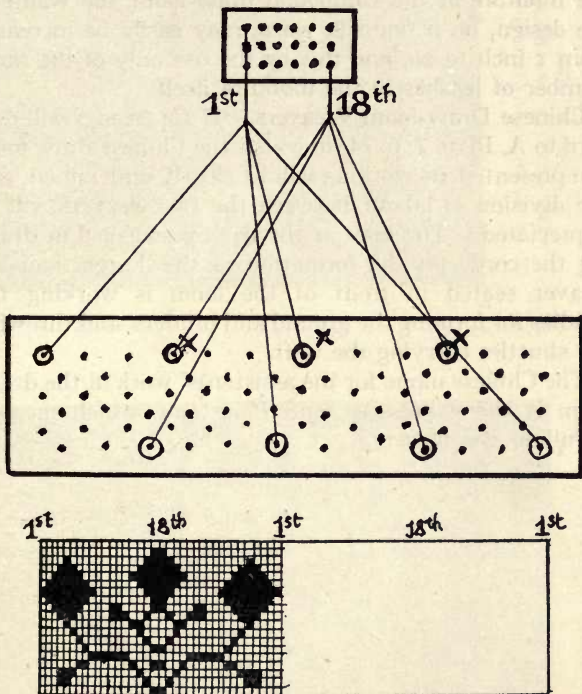
FIG. 37. POINT REPEATING MONTURE
