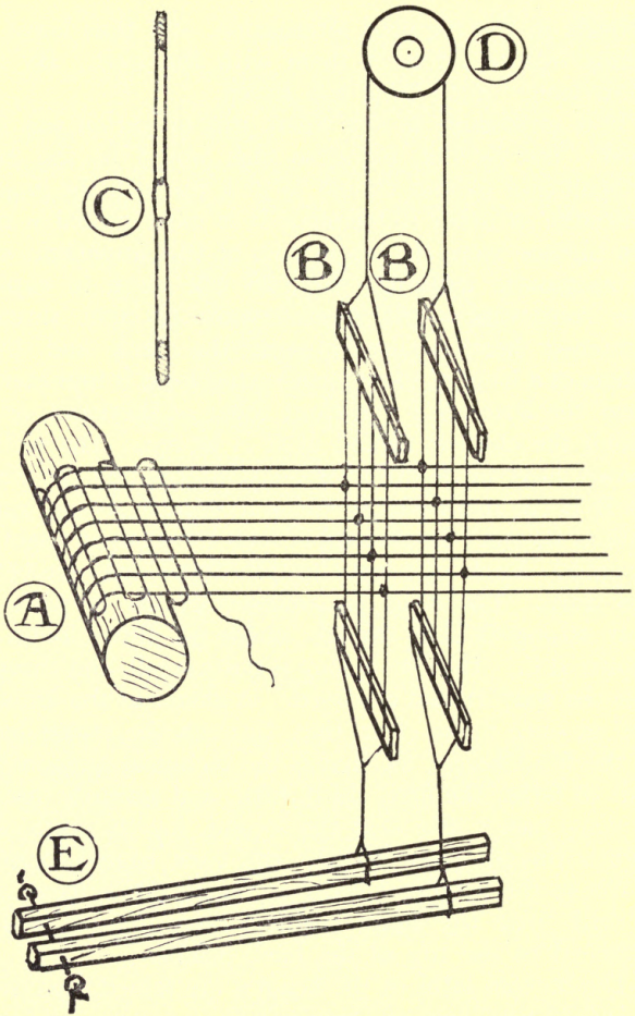
FIG. 25. HEADLES FOR OPENING THE WARP OR SHED
