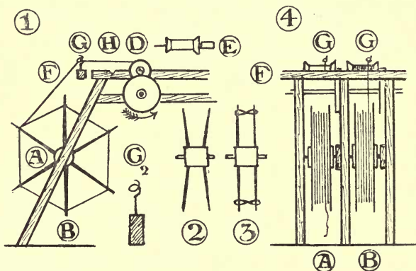
FIG. 14. WINDING MACHINE
