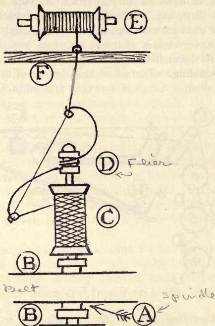
FIG. 16. SPINDLE AND FLIER 1
