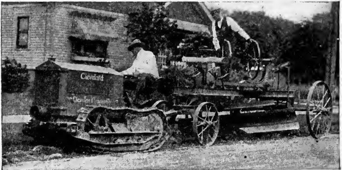
FIG. 245.—Opening road drains with scraper and tractor. (Cleveland Tractor Co.)
