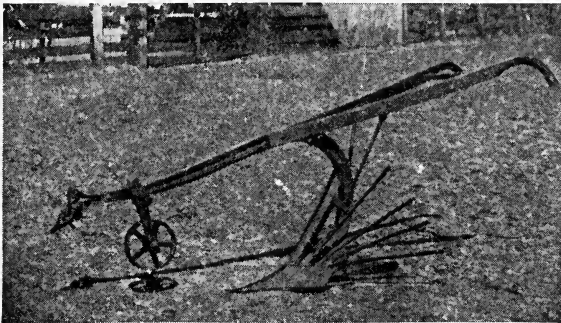
FIG. 87a.—An inexpensive potato digger to be drawn by one or two horses. (Plant Industry.)
