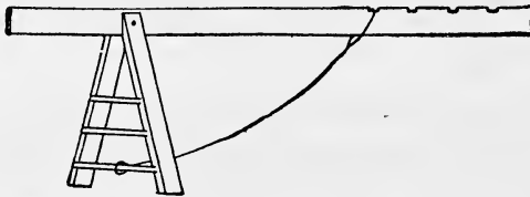
FIG. 237.—Lifting lever for wagon rack or bed. It saves heavy lifting and requires only one person.
