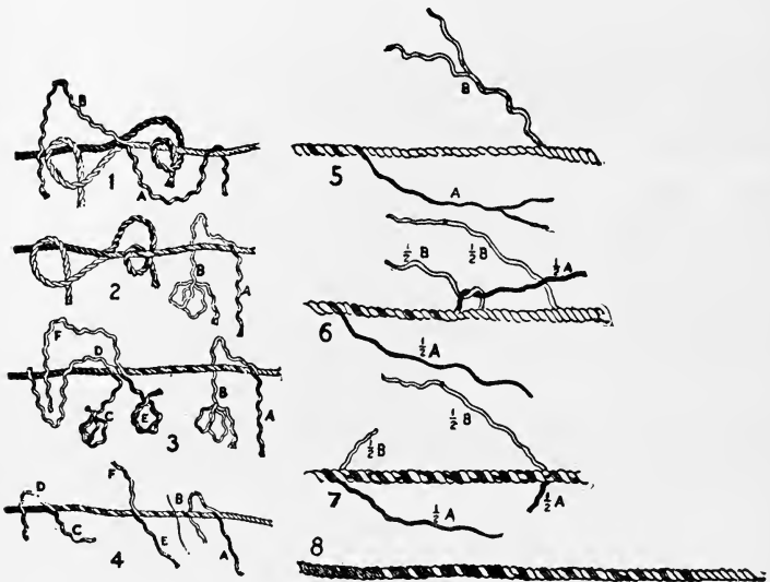
FIG. 232.—Eight stages or steps in the long splice. (First four stages after H. W. Riley.)
