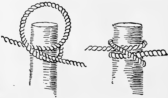
FIG. 230.—Clove hitch, sailor method.
