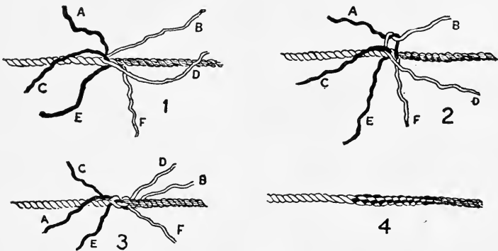
FIG. 231.—Short splice, showing four stages in the operation 1. The six strands of the two ropes arranged in pairs, A-B, C-D, E-F. 2. A-B tied with first overhand knot. 3. Each of the three pairs tied with first step of surgeon's knot. 4. Completed splice.
