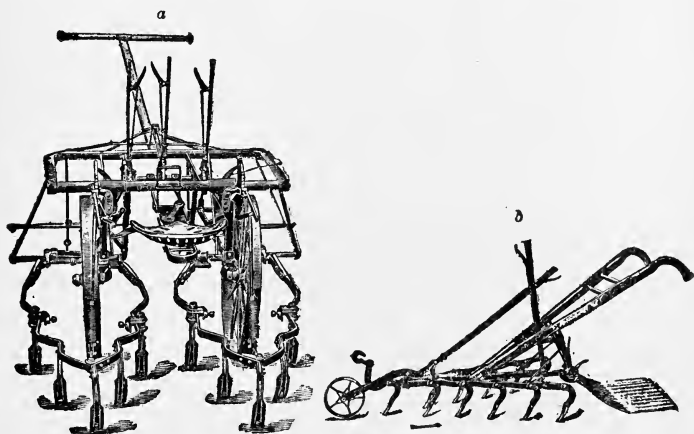
FIG. 36a.—A ten-shovel sulky cultivator. This form of machine leaves a fine soil surface which helps to save moisture.
