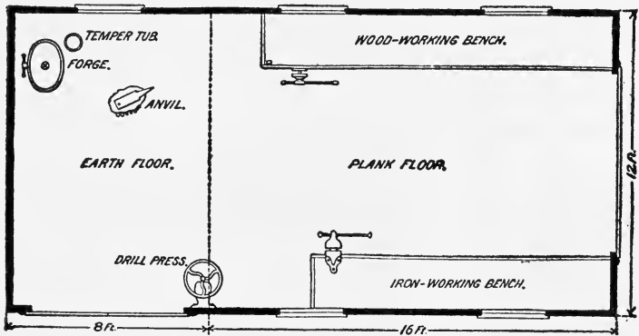
FIG. 234.—Floor plan of workshop. (U.S.D.A.)
