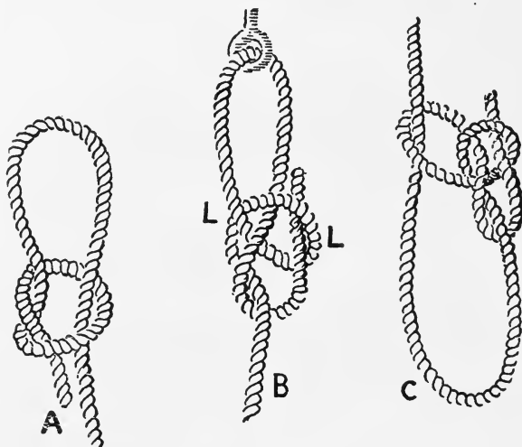
FIG. 228.— A , slip knot; B , bowline; C , running bowline.
