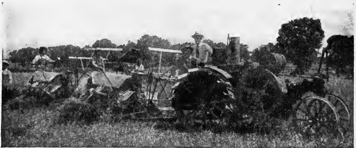
FIG. 251.—Tractor used in harvesting oats with two self-binders. (International Harvester Co.)
