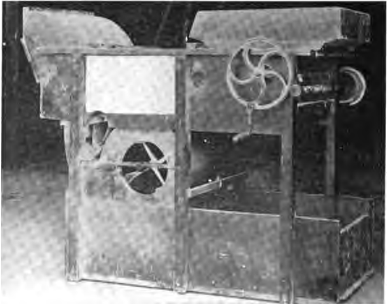
FIG. 40.—An inexpensive fanning mill should be used to reclean farm seeds before planting. Light seeds, chaff and other trash are blown out by the fan. Sieves should be used of suitable size to separate the seeds of different sizes. (U. S. D. A.)
