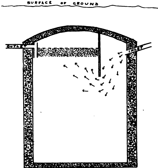
FIG. 309.—A septic tank should receive all wastes from the kitchen and bath room. It will destroy these materials and allow only clear water to pass on.
