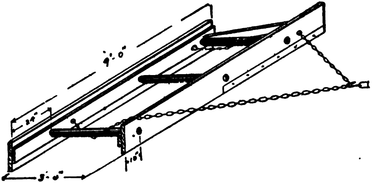
FIG. 306.—This drag is made from two pieces of ten or twelve inch plank, two or three inches thick and eight or nine feet long, reinforced by a two-inch by six-inch strip. The cross braces are four-inch sticks shaped to fit a two-inch hole. A board platform, not shown in the cut, is laid on the cross pieces for the driver to stand upon. (U. S. D. A.)
