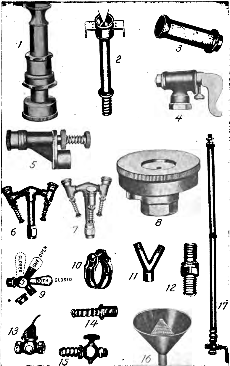
FIG. 297.—Spraying accessories. 1, simplest type nozzle; 2, 3, types little used; 4, Bordeaux nozzle; 5, 6, 7, Vermorel type much used, also nozzle clusters; 8, recent type, similar to Vermorel but of greater capacity; 9, cut-off; 10, hose clamp; 11, Y for cluster; 12, hose coupling; 13, 15, stopcocks; 14, connection, 16, strainer; 17, bamboo rod, with cut-off. (Fights of the Farmer.)
