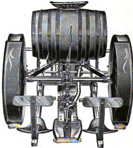
FIG. 180.—The transplanting machine is used on farms growing large crops of cabbage, cauliflower, tobacco and sweet potatoes. Water is supplied to each plant from the barrel. (see also figure 255.) (Productive Vegetable Growing.)
