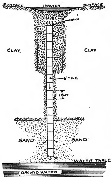
FIG. 62.—A vertical drain. A porous or gravelly stratum should underlie the impervious hard-pan or subsoil, and the water must have a chance to flow away. (Wis. Station.)
