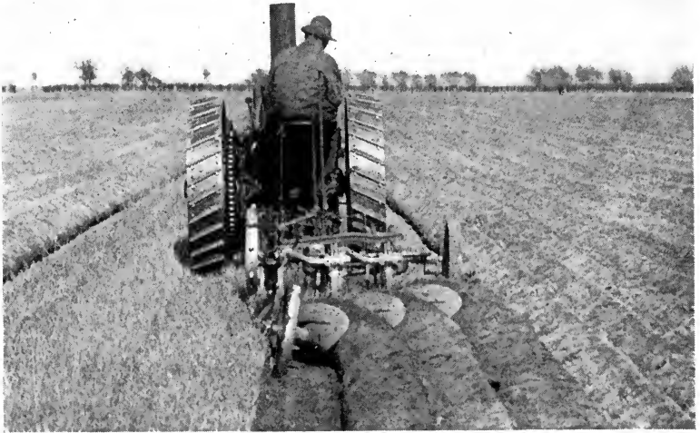
FIG. 87.—A three-bottom tractor plow at work.
