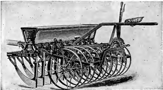
FIG. 98.—Press drill.
