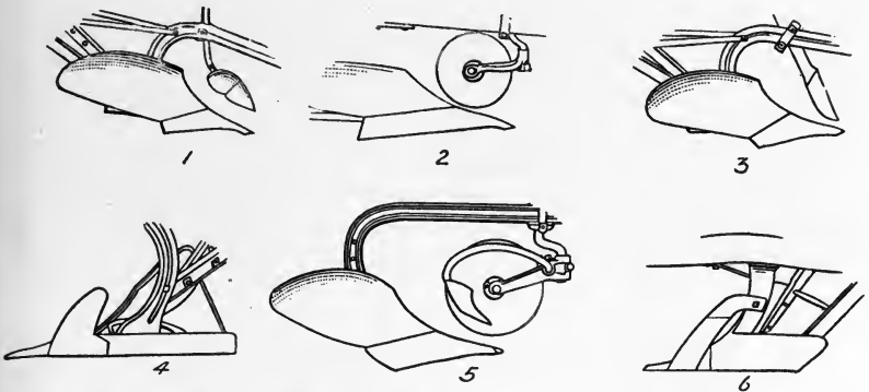
FIG. 74.—Different types of coulters and jointers. Note proper adjustment. 1, jointer; 2, rolling coulters; 3, blade coulters or hanging cutters; 4, fin coulters or cutters; 5, combination rolling coulters and jointers; 6, knee cutters or coulters.
