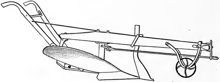
FIG. 79.—A prairie breaker.
