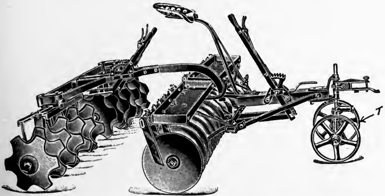
FIG. 90.—A double disk harrow. Cutaway disk in rear. T , truck or forecarriage.
