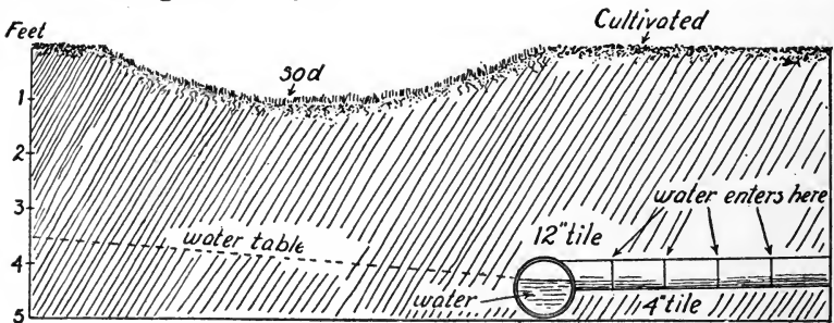
FIG. 59.—Tile combined with surface-run. The surface-run carries the water when there is a flood, while the tile works throughout the year. (Wisconsin Station.)
