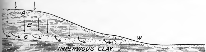
FIG. 39.—Diagram showing difference between percolation and seepage; A , the tilled soil; B , permeable subsoil through which free water percolates; C , sandy gravel substratum through which ground water moves laterally; W , area at foot of slope kept wet by seepage of water out from the upland; O , place to put tile to catch the seepage water.
