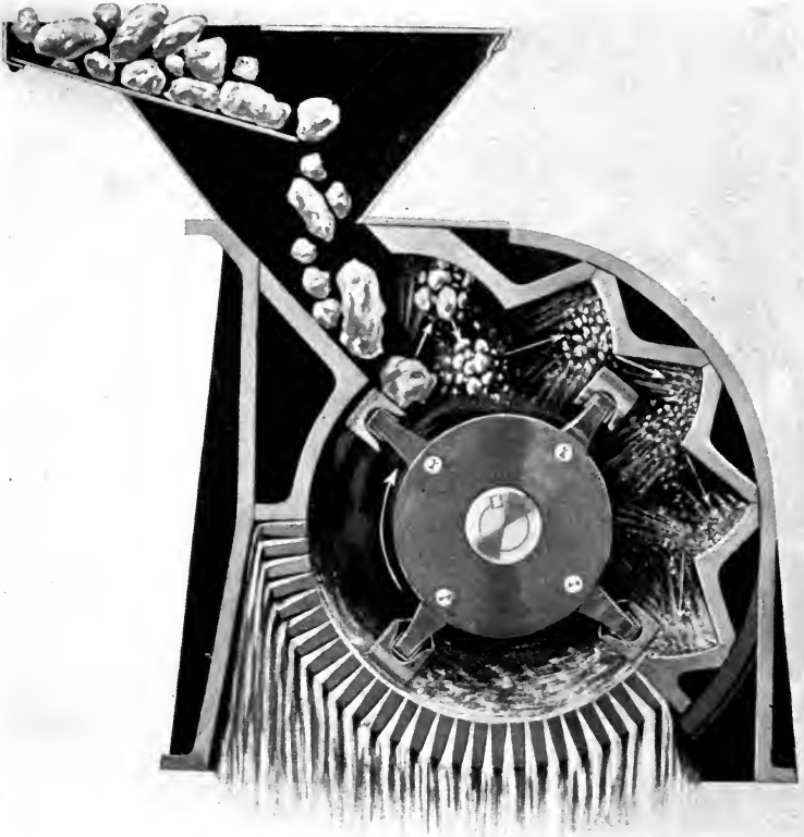
FIG. 155.—Limestone pulverizers are built on the swing-hammer principle.
