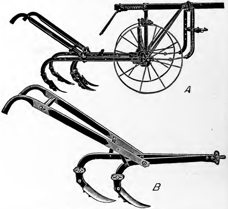
FIG. 110.—Two other types of walking cultivators. A, four-shovel; B, two-shovel cultivator, or double shovel plow. B is a cultivator commonly used in the South.
