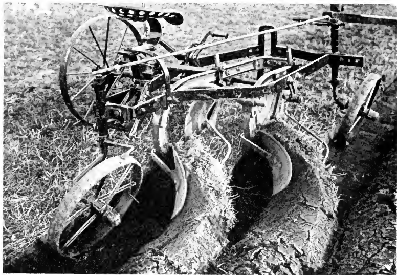
FIG. 69.—The way a good plow does its work. When one becomes interested in the action of the plow, plowing ceases to be a drudgery.
