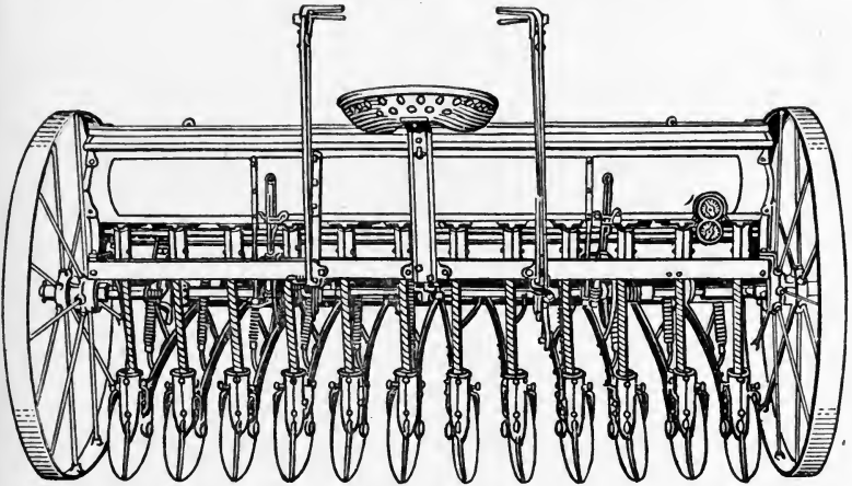
FIG. 99.—Single disk grain drill.
