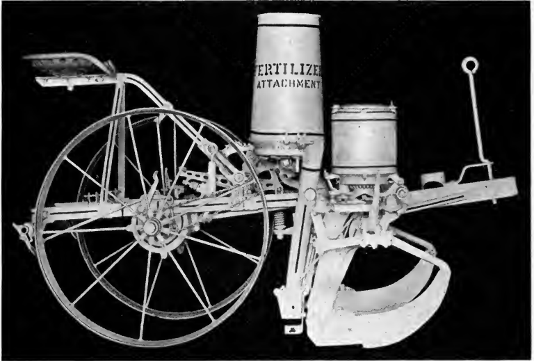
FIG. 143.—A fertilizer attachment on the corn planter. Note the fertilizer spreader (S).
