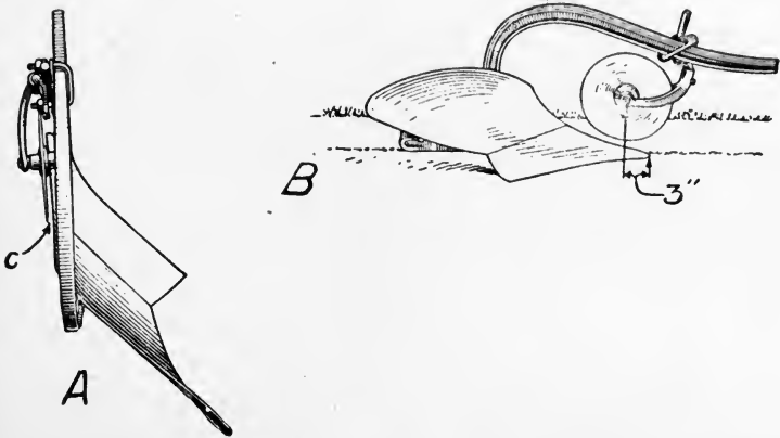
FIG. 73.—Adjustment of coulters. A , ordinarily set coulters one-half inch from landside ( c ). In deep plowing or for sod one-quarter inch. Secure a full furrow slice to keep shin covered with dirt. B , set middle of rolling coulters about three inches back from point. In loose or trashy soils, one or two inches back. In hard or sticky soils, about four inches back.
