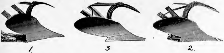
FIG. 72.—Three types of plow bottoms: 1, stubble bottom; 2, general purpose; 3, sod.
