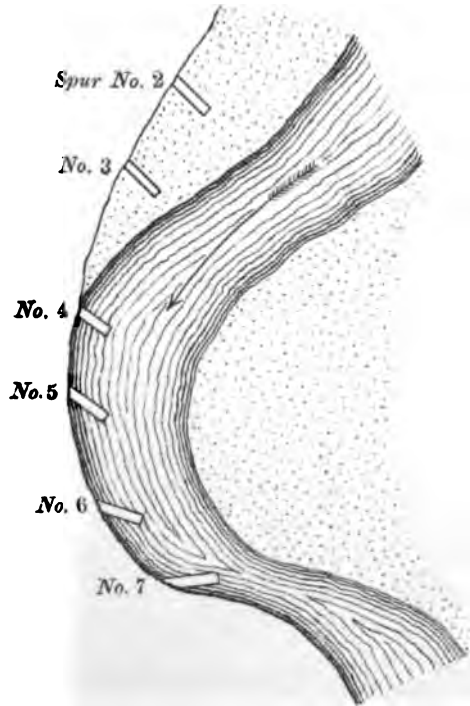
FIG. 4. EROSION AT KHARAK- WALA, RIVER INDUS, JANUARY 1879.
