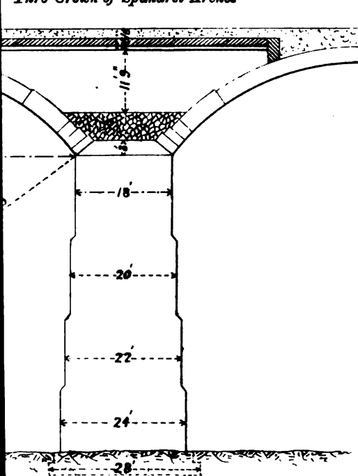
LONGITUDINAL SECTION Thro' Crown of Spandrel Arches
