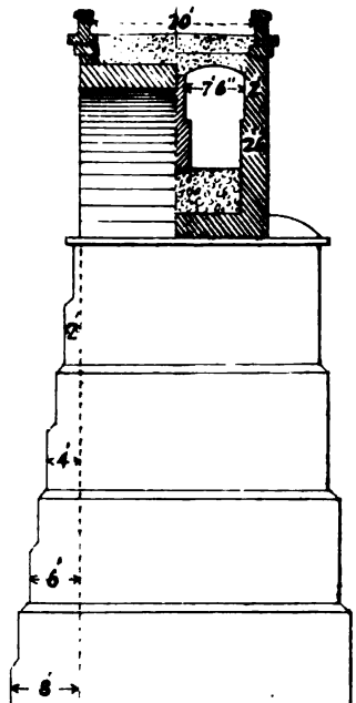
CROSS SECTION Thro' Crown over Pier
