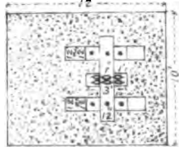
FIG. 3. PLAN OF ABUTMENT.
