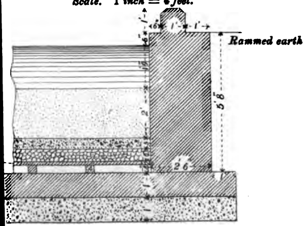
SECTION OF FILTER. SEE PLATE I. Shape Rectangular—160' X 80' Scale. 1 inch = 4 feet.
