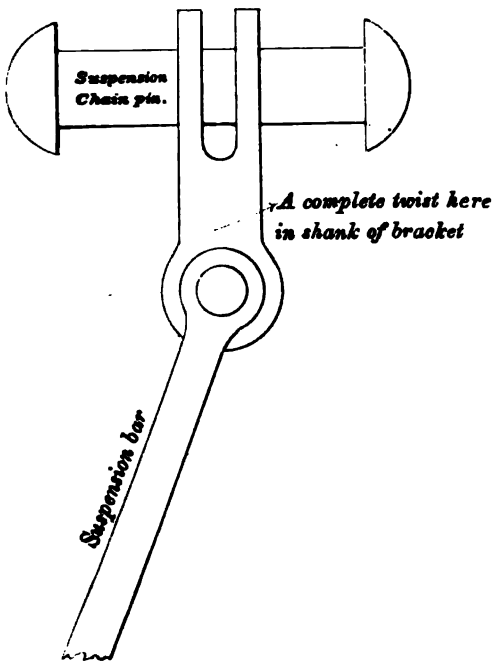
FIG. 1. AS DESIGNED
