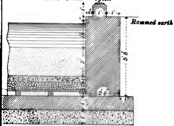
SECTION OF FILTER. SEE PLATE I. Shape Rectangular—160' X 80 Scale. 1 inch = 4 feet.
