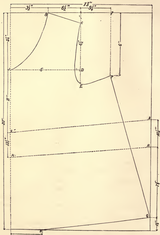
Fig. 69. — Front of chemise waist.
