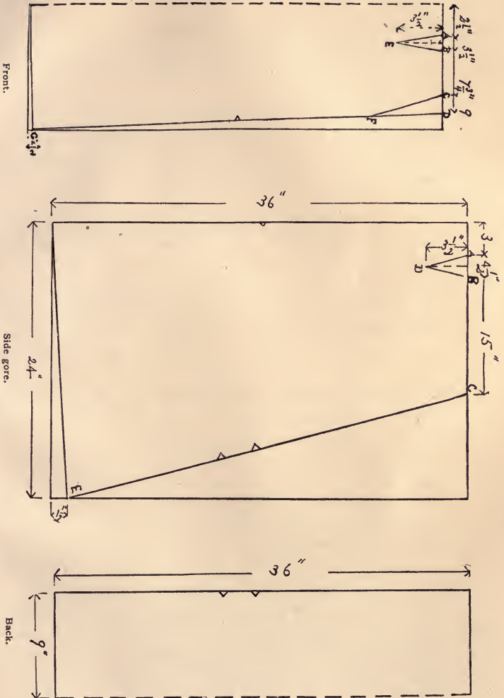
Fig. 83.—Pattern of a gored skirt. Scale 1/8" = 1".
